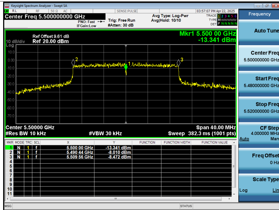
Freq. Stability -10C 12V ax20 5500MHz Ant1 0 Minutes
