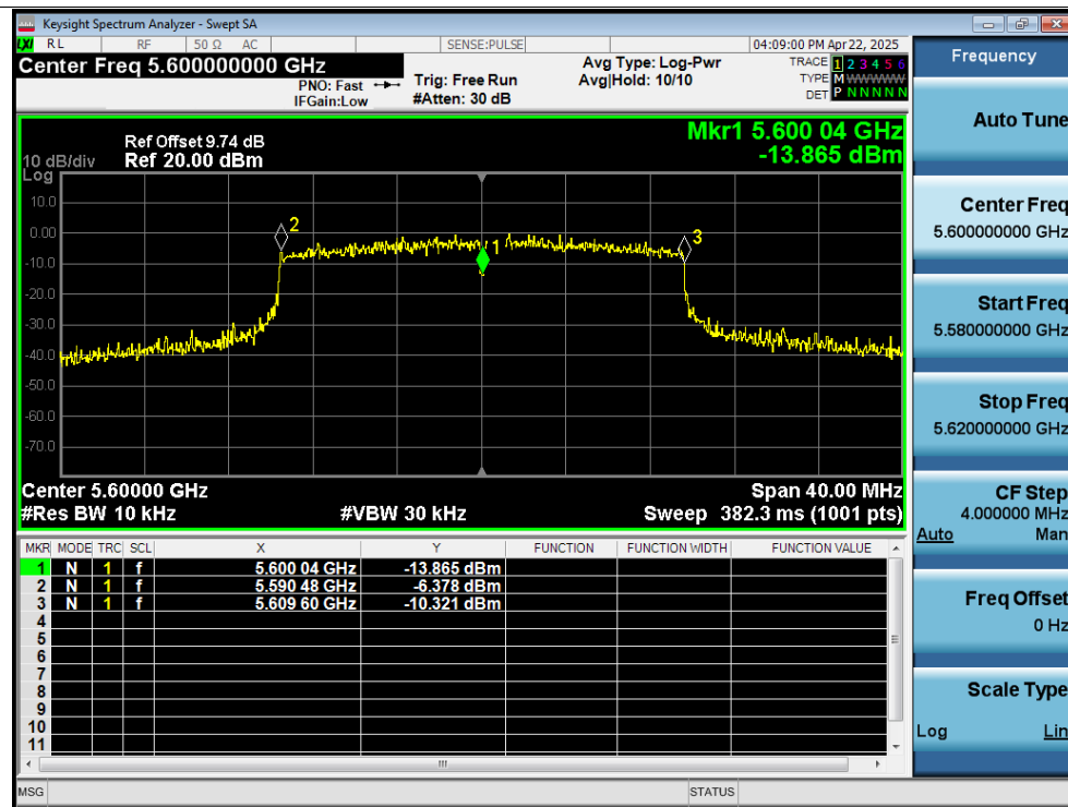
Freq. Stability -10C 12V ax20 5600MHz Ant1 0 Minutes
