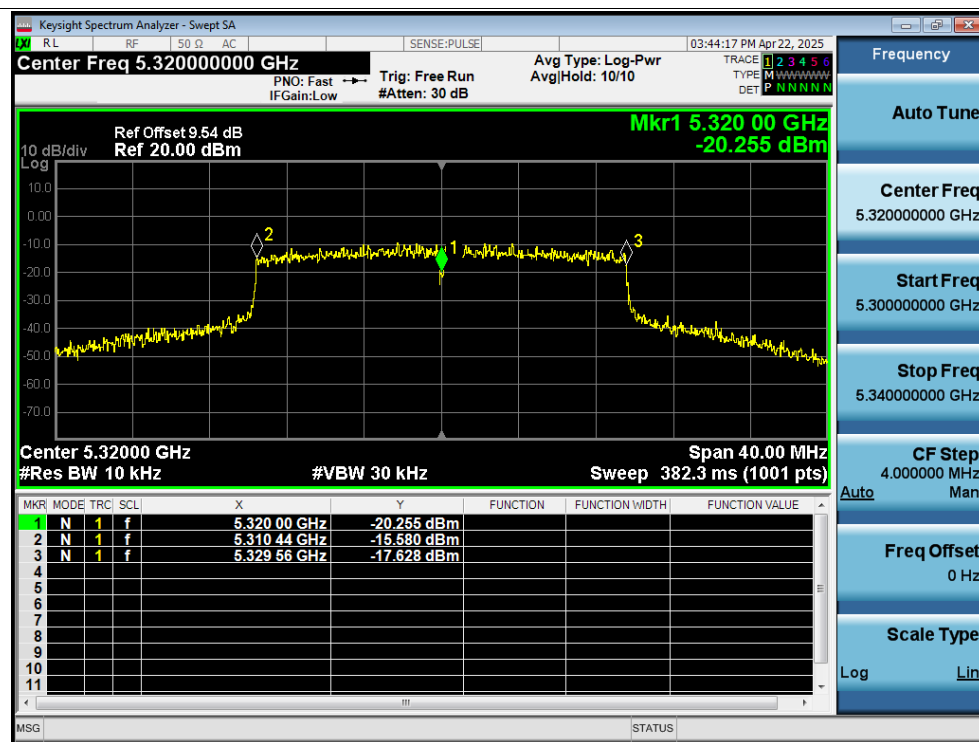
Freq. Stability -10C 12V ax20 5320MHz Ant1 0 Minutes
