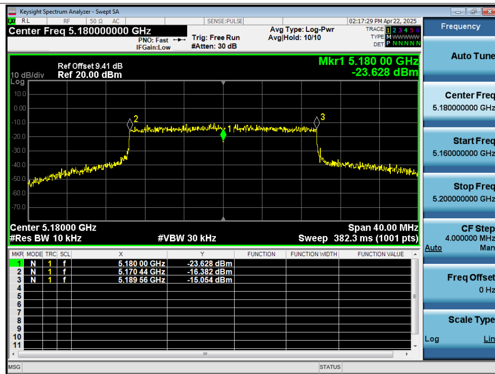
Freq. Stability -10C 12V ax20 5180MHz Ant1 0 Minutes
