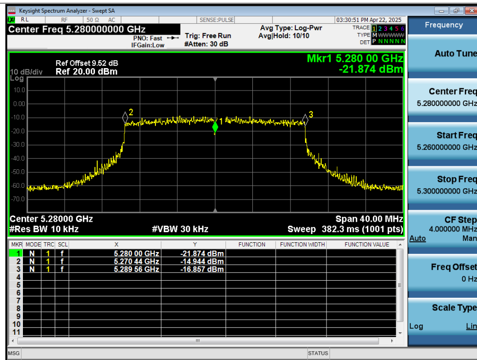
Freq. Stability 20C 13.8V ax20 5280MHz Ant1 0 Minutes
