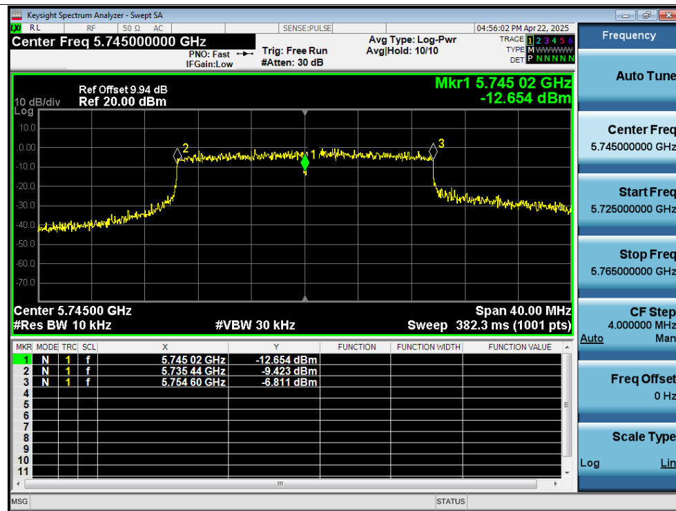
Freq. Stability -10C 12V ax20 5745MHz Ant1 0 Minutes
