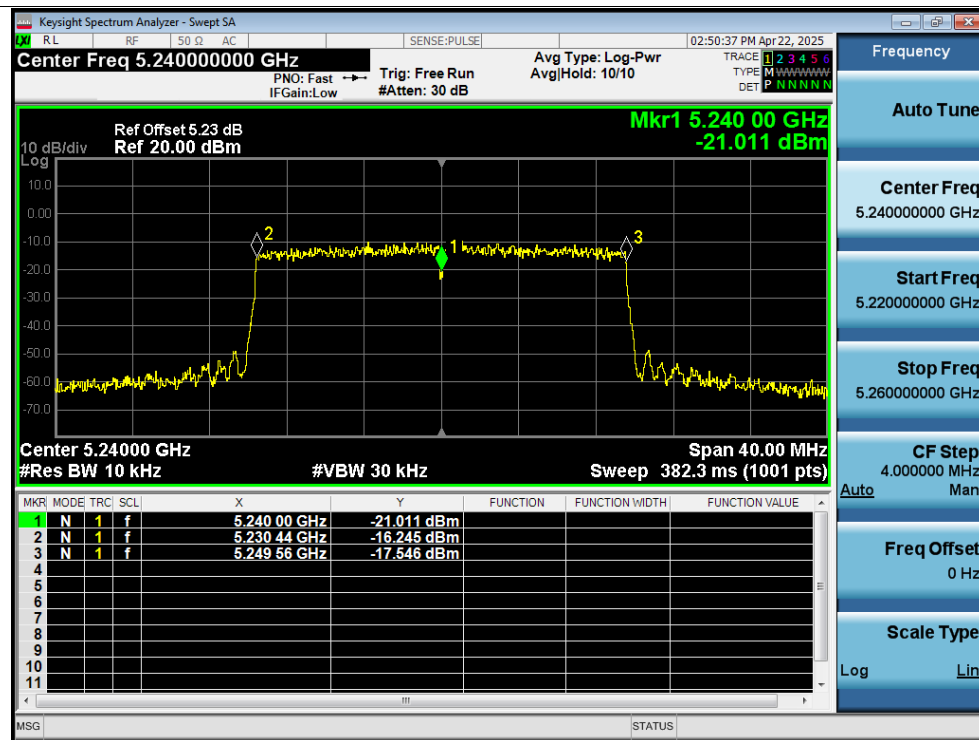
Freq. Stability 20C 13.8V ax20 5240MHz Ant2 0 Minutes
