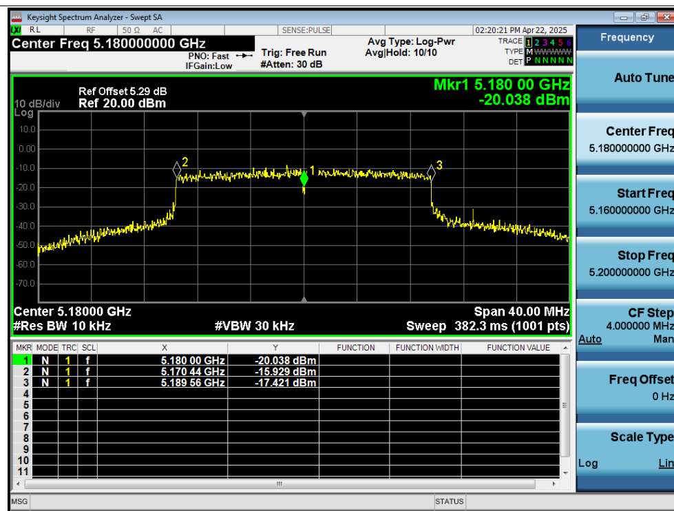
Freq. Stability 20C 10.2V ax20 5180MHz Ant2 0 Minutes
