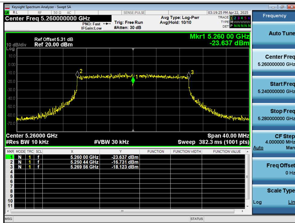
Freq. Stability -10C 12V ax20 5260MHz Ant2 0 Minutes
