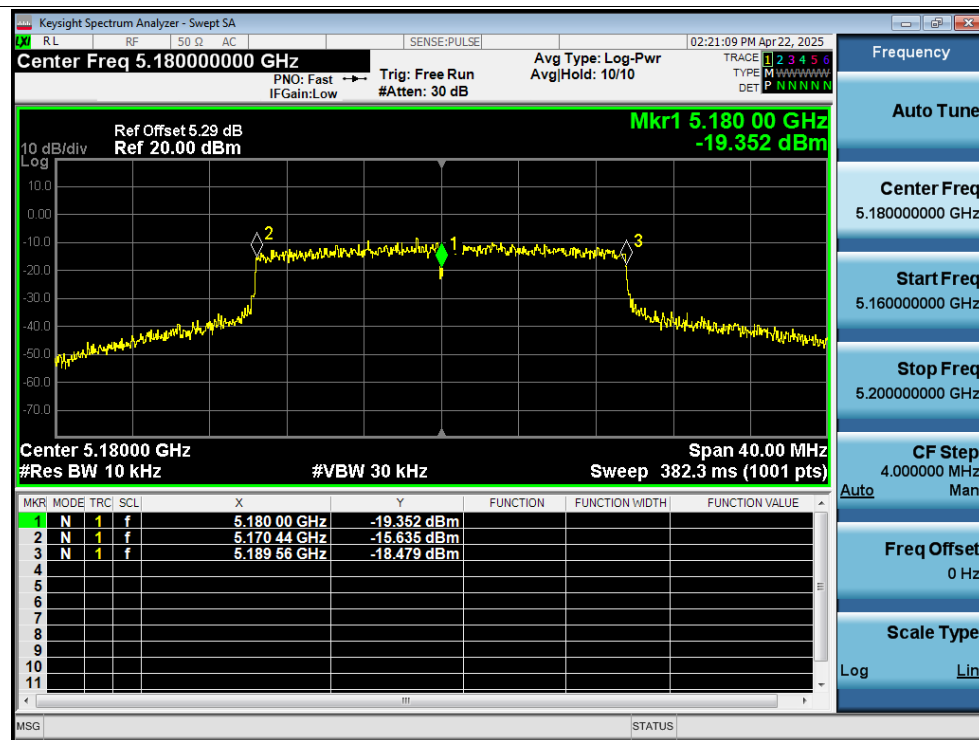
Freq. Stability -10C 12V ax20 5180MHz Ant2 0 Minutes
