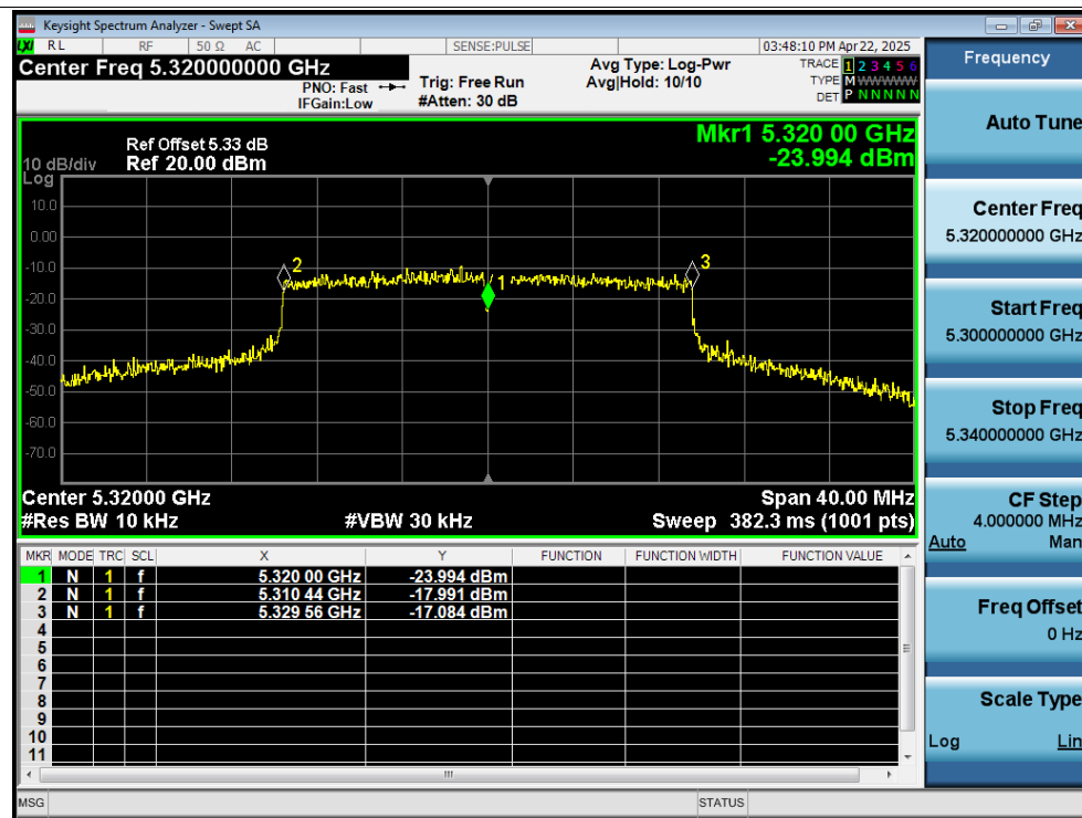
Freq. Stability -10C 12V ax20 5320MHz Ant2 0 Minutes
