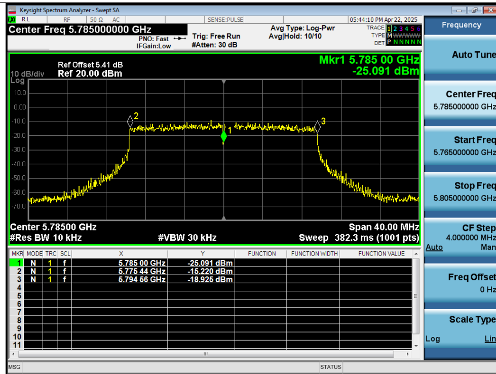
Freq. Stability -10C 12V ax20 5785MHz Ant3 0 Minutes
