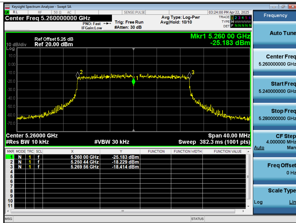
Freq. Stability 20C 13.8V ax20 5260MHz Ant3 0 Minutes
