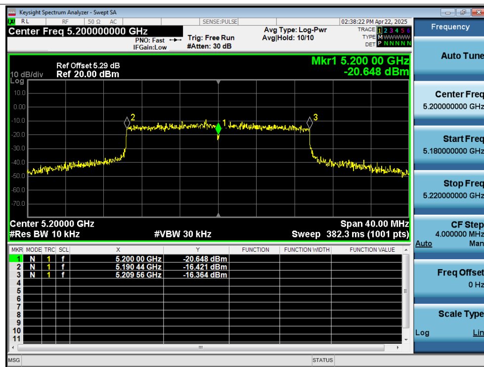
Freq. Stability 20C 13.8V ax20 5200MHz Ant3 0 Minutes
