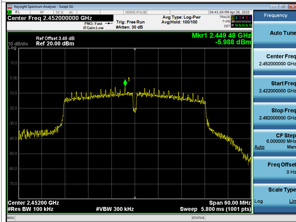
Tx. Spurious NVNT ac40 2452MHz Ant2 Emission
