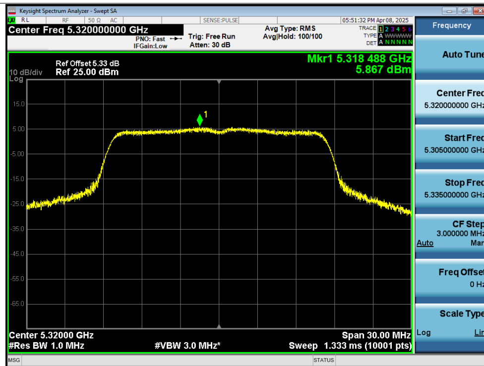
PSD NVNT a 5320MHz Ant3
