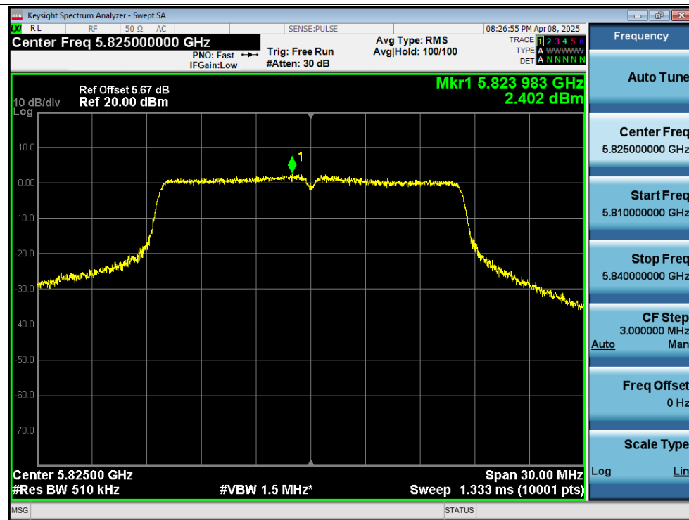
PSD NVNT a 5825MHz Ant3
