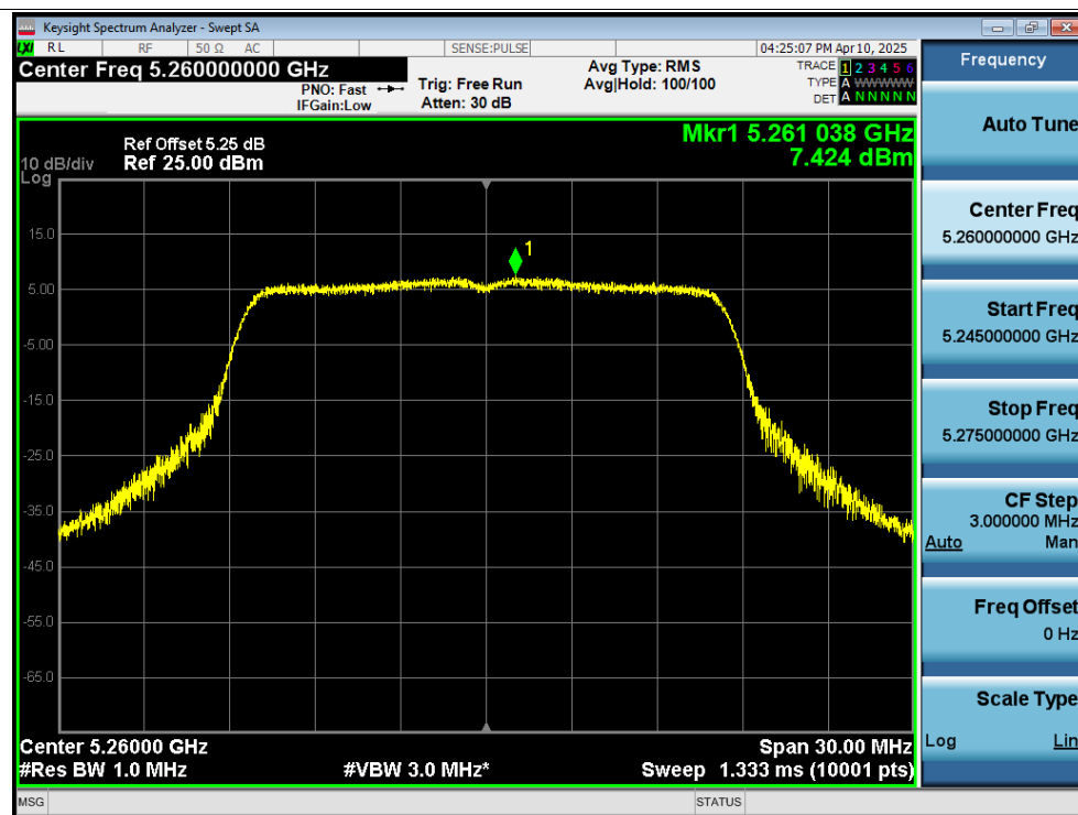
PSD NVNT a 5260MHz Ant3
