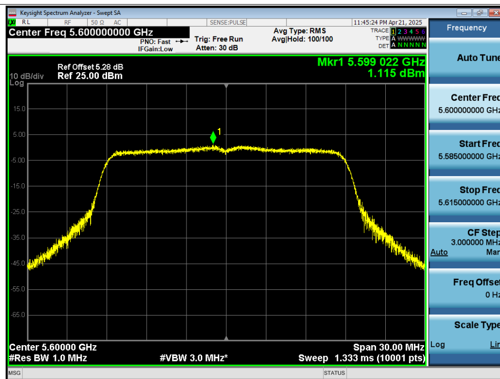
PSD NVNT n20 5600MHz Ant3
