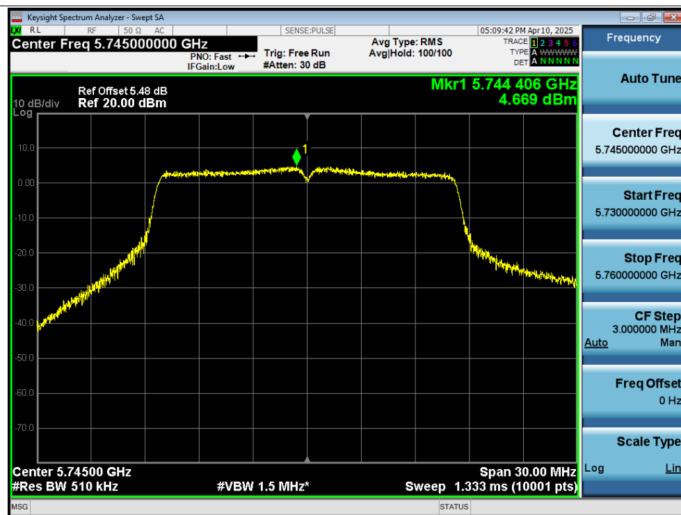
PSD NVNT a 5745MHz Ant3
