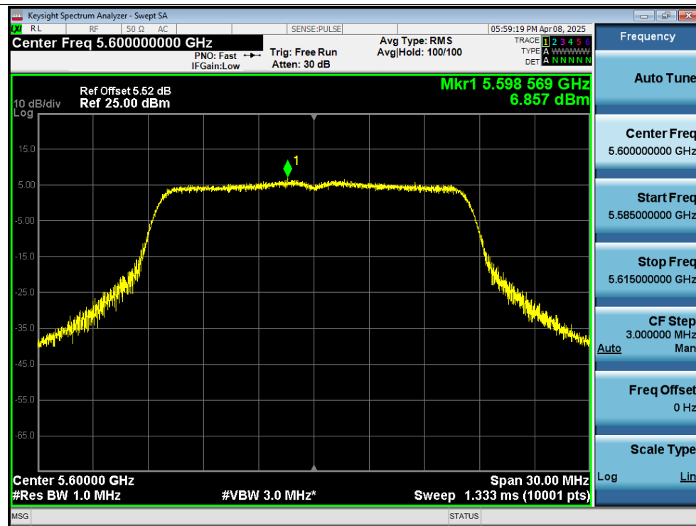
PSD NVNT a 5600MHz Ant3
