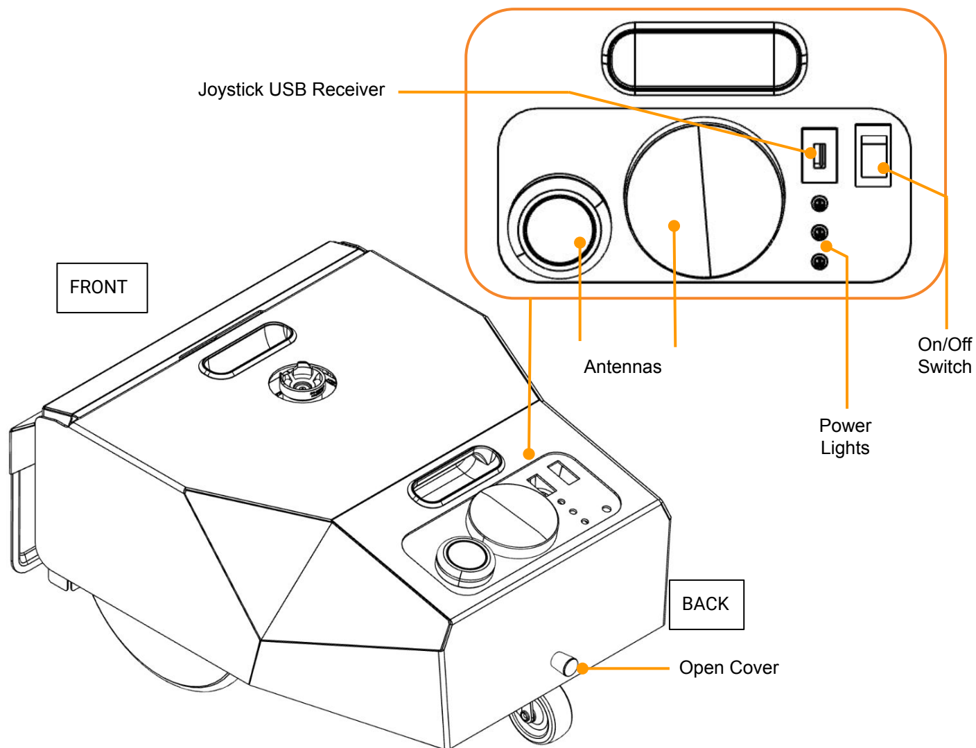
TOP PANEL VIEW
