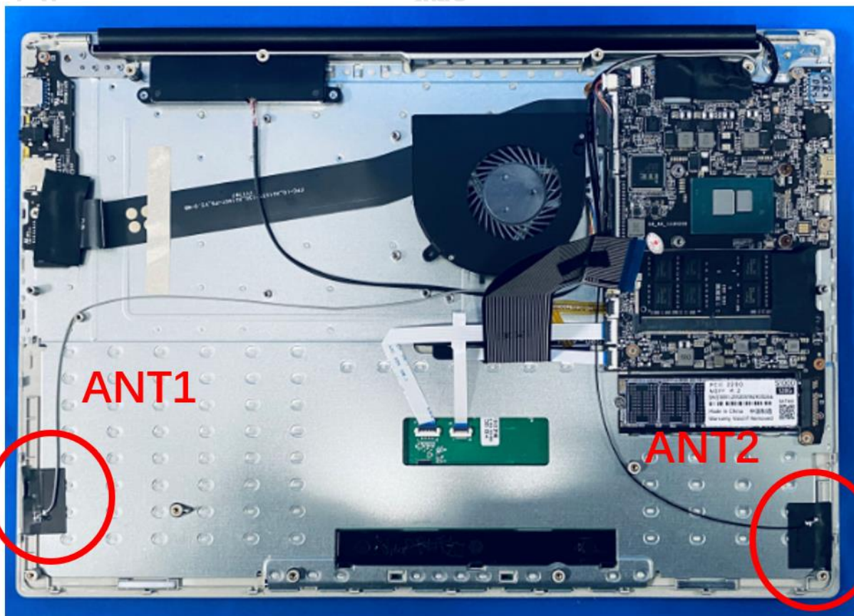
REAR VIEW
