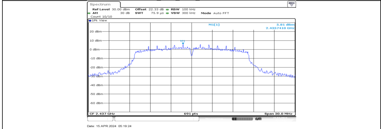
11G_Ant1_2437_0-Reference
