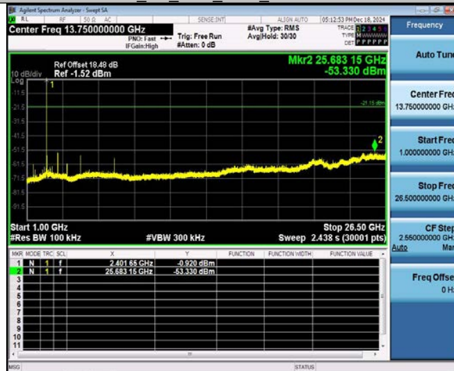
BLE_1M_Ant1_2402_1000~26500
