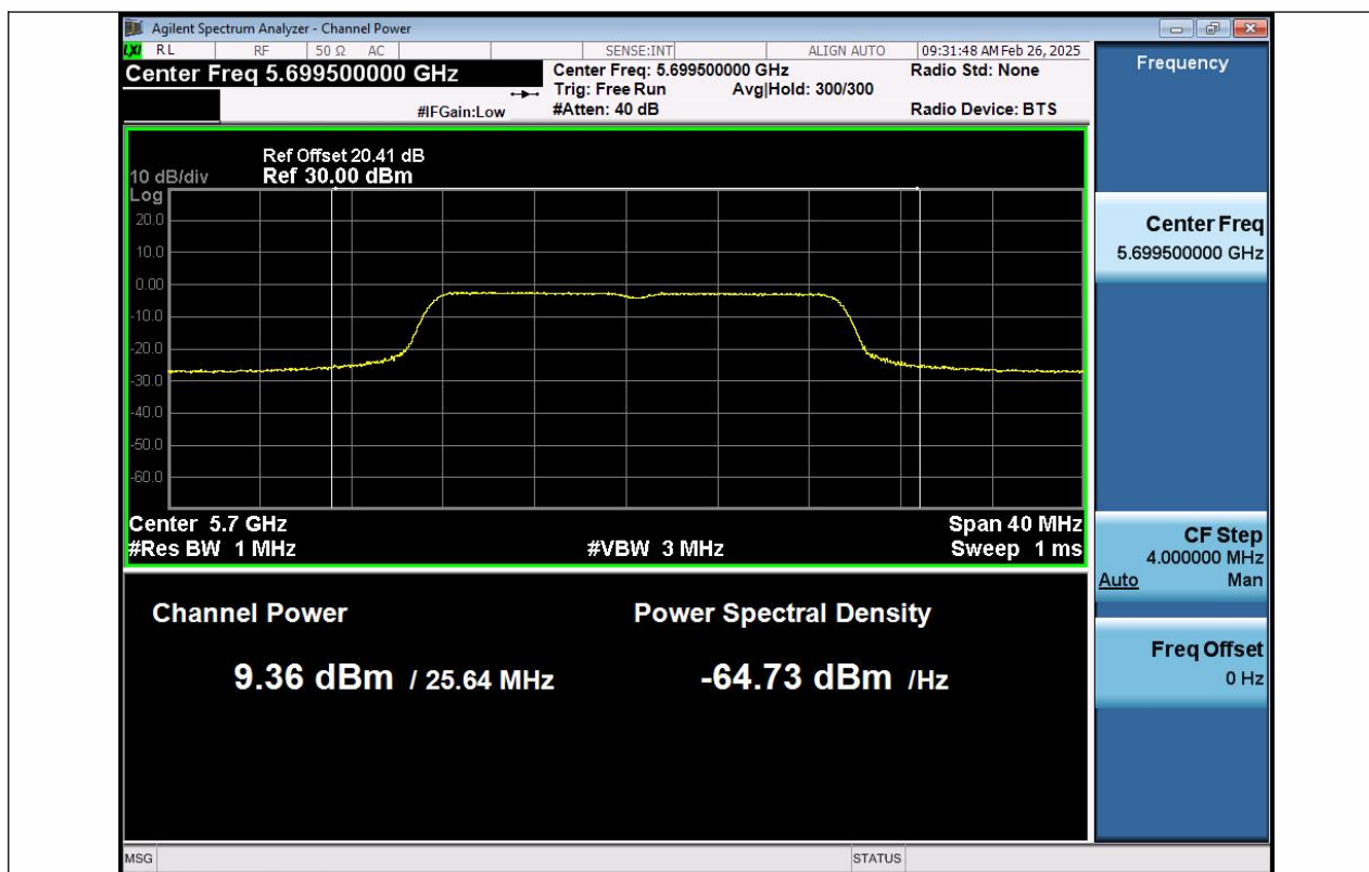
11N20SISO-Ant1-5700-PASS
