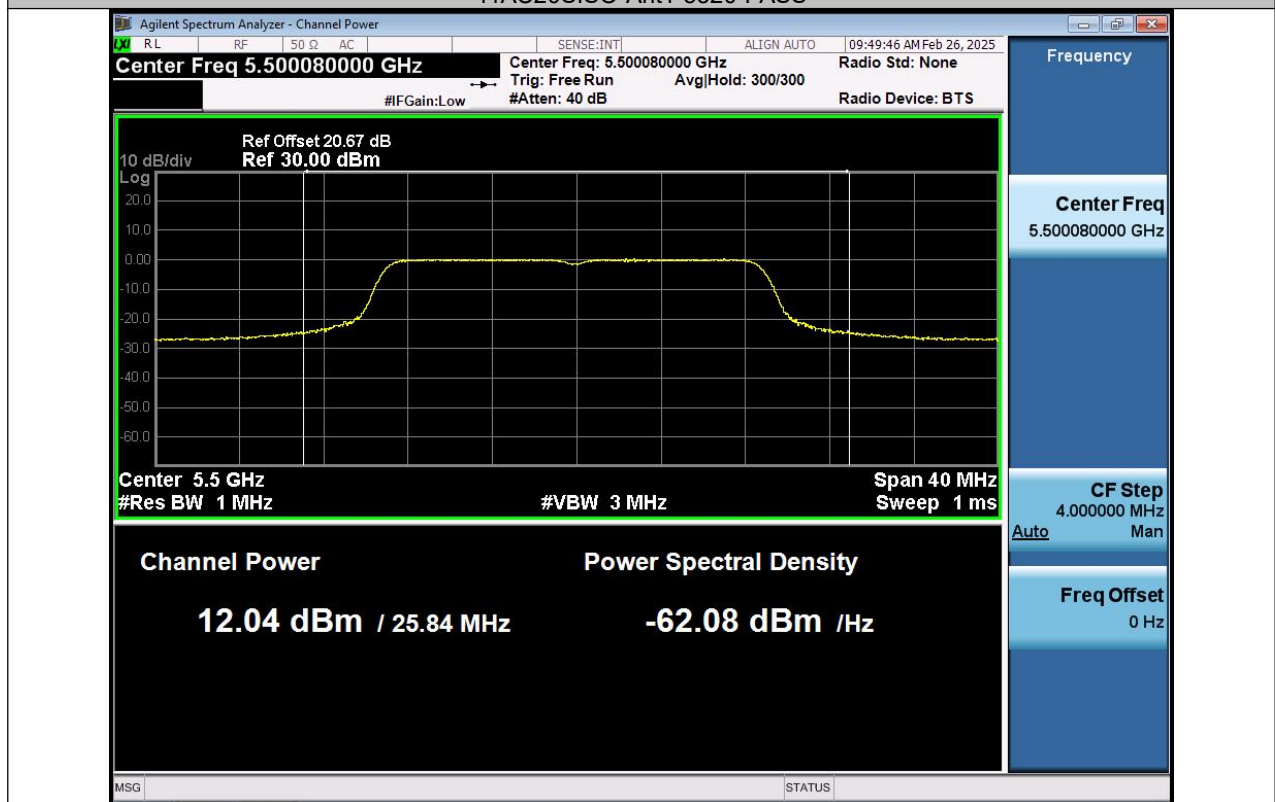
11AC20SISO-Ant1-5500-PASS
