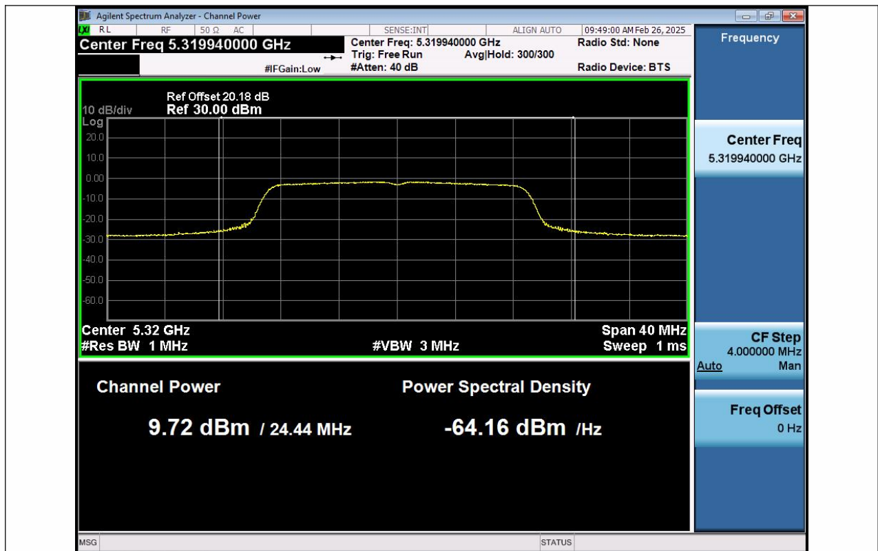
11AC20SISO-Ant1-5320-PASS
