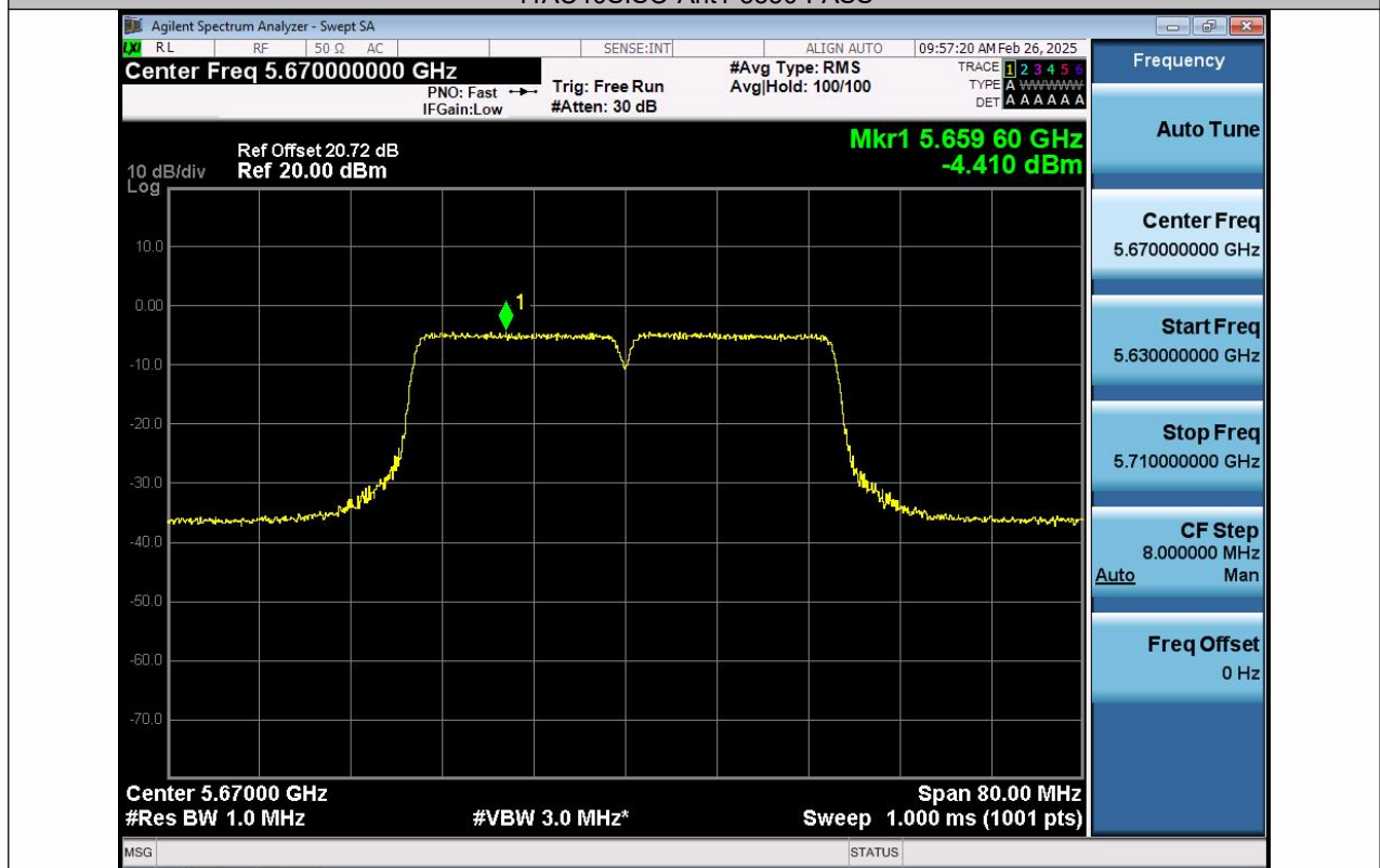
11AC40SISO-Ant1-5670-PASS
