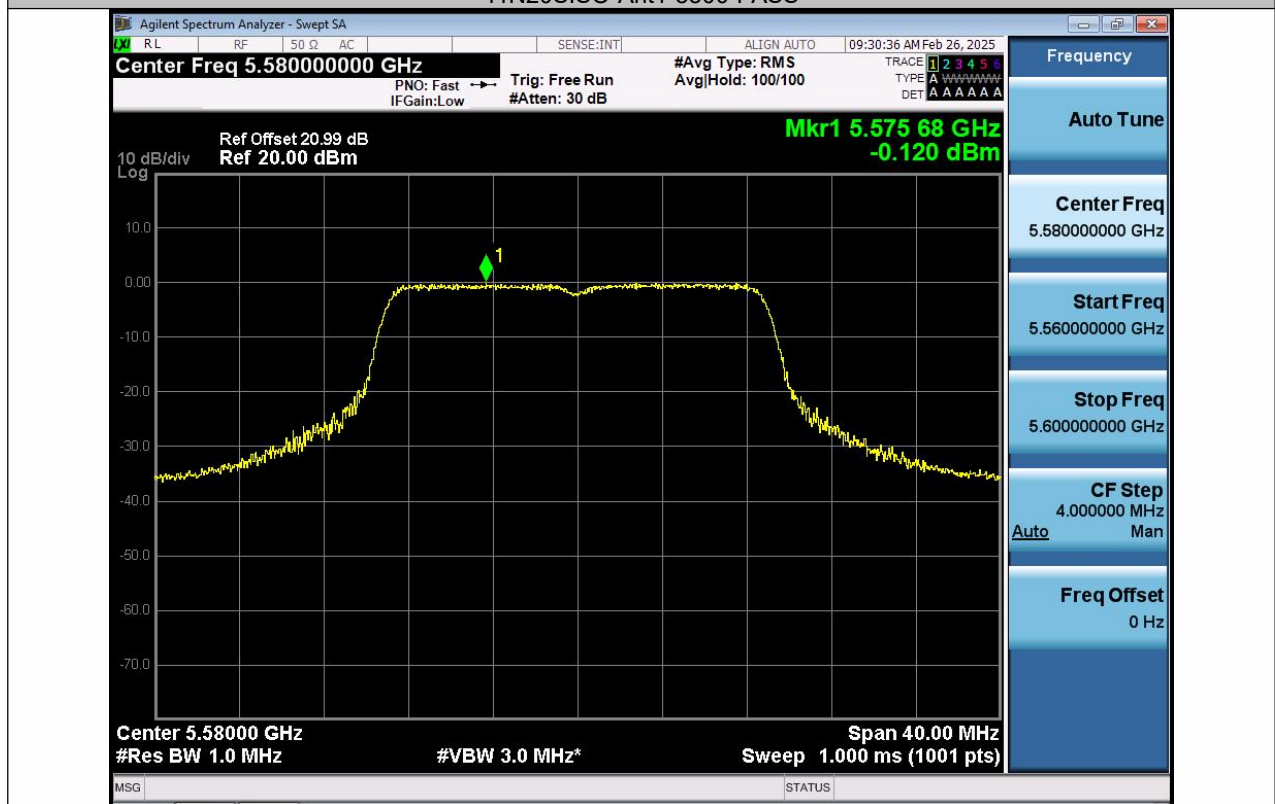
11N20SISO-Ant1-5580-PASS
