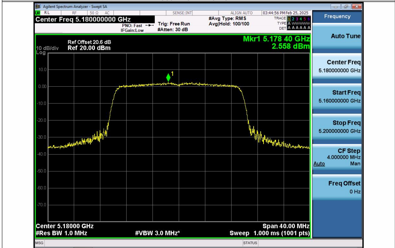
11AX20SISO-Ant1-5180-PASS
