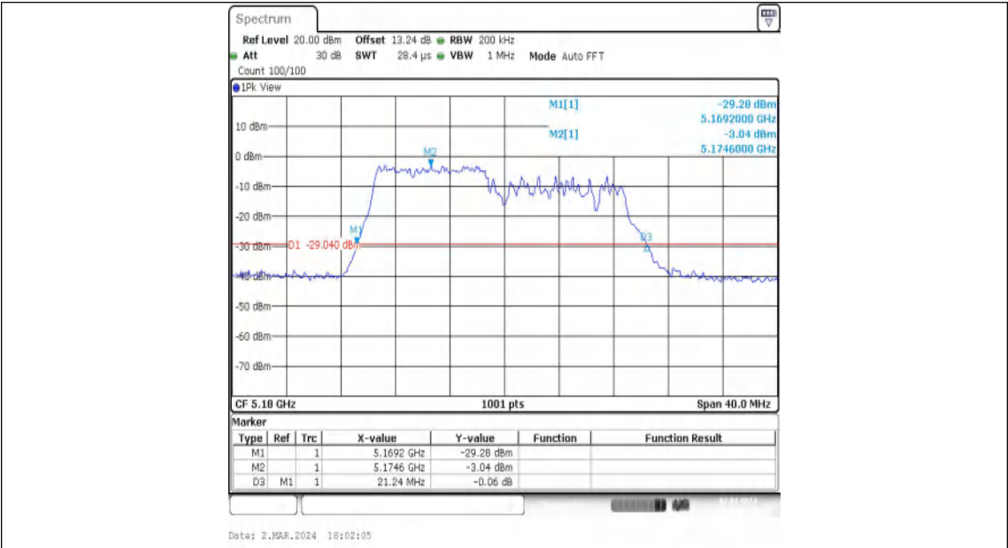
11AX20MIMO-Ant2-5180-106Tone-RU53
