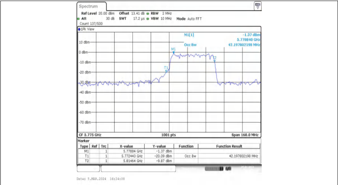
11AX80MIMO-Ant1-5775-484Tone-RU66
