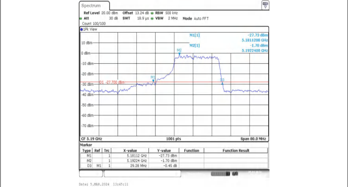
11AX40MIMO-Ant2-5190-242Tone-RU62
