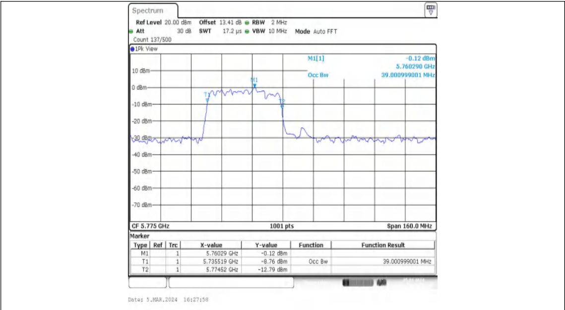
11AX80MIMO-Ant1-5775-484Tone-RU65
