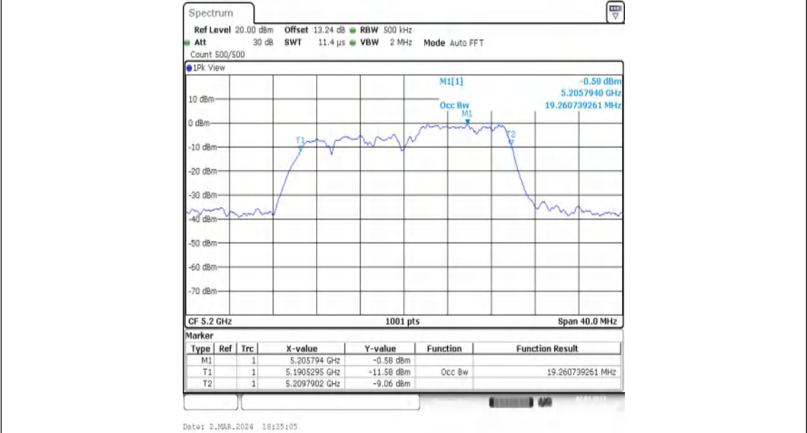
11AX20MIMO-Ant2-5200-106Tone-RU54
