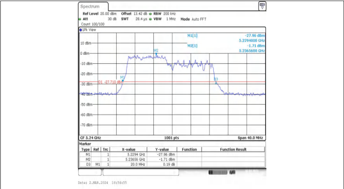
11AX20MIMO-Ant1-5240-106Tone-RU53
