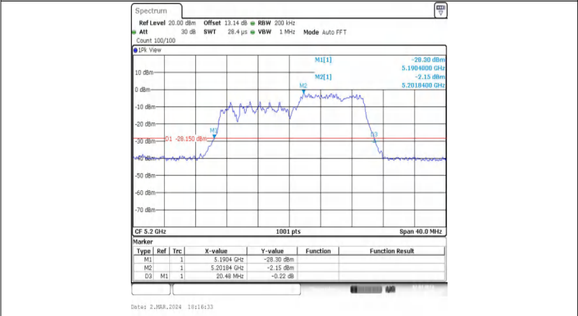
11AX20MIMO-Ant1-5200-106Tone-RU54
