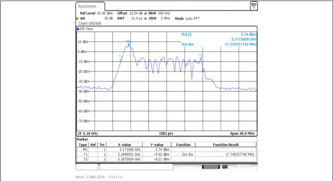
11AX20MIMO-Ant2-5180-26Tone-RU0
