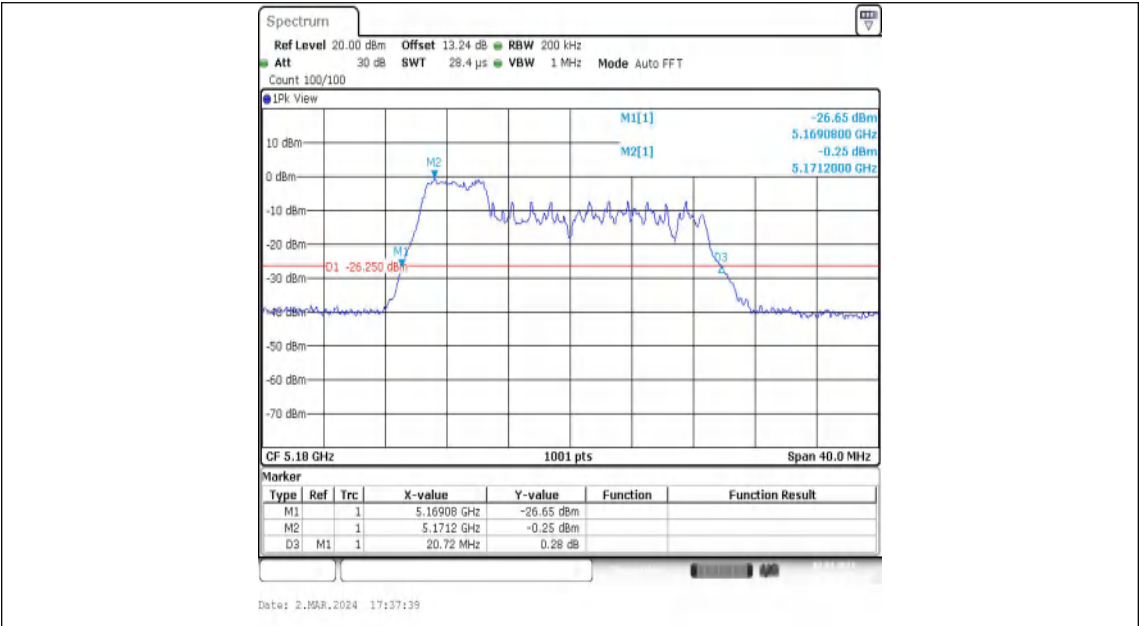
11AX20MIMO-Ant2-5180-52Tone-RU37
