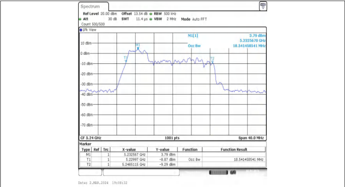
11AX20MIMO-Ant2-5240-52Tone-RU37
