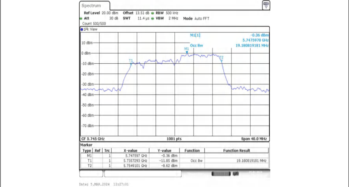
11AX20MIMO-Ant2-5745-106Tone-RU54
