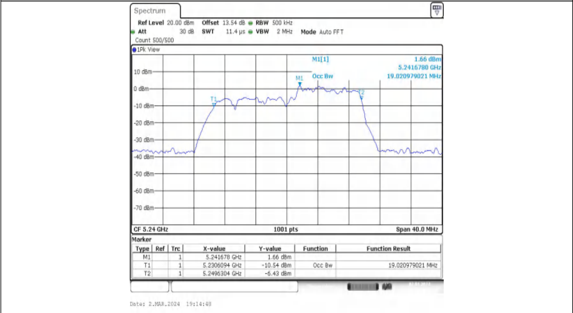
11AX20MIMO-Ant2-5240-106Tone-RU54
