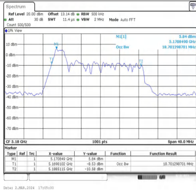
11AX20MIMO-Ant1-5180-26Tone-RU0
