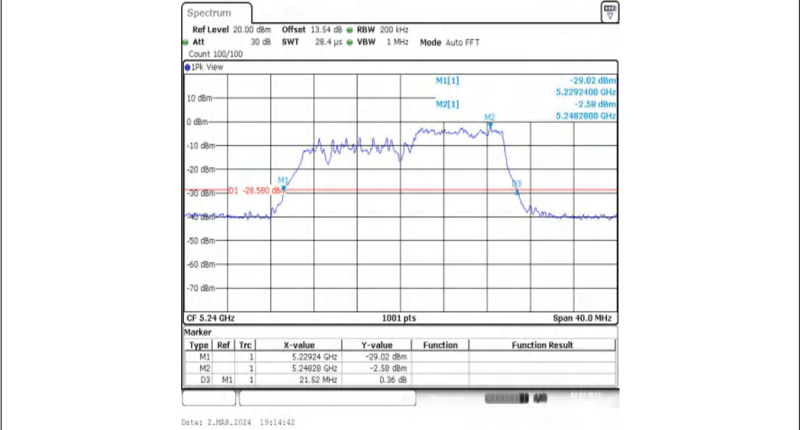
11AX20MIMO-Ant2-5240-106Tone-RU54
