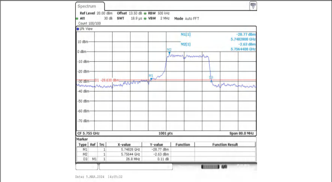
11AX40MIMO-Ant2-5755-242Tone-RU62
