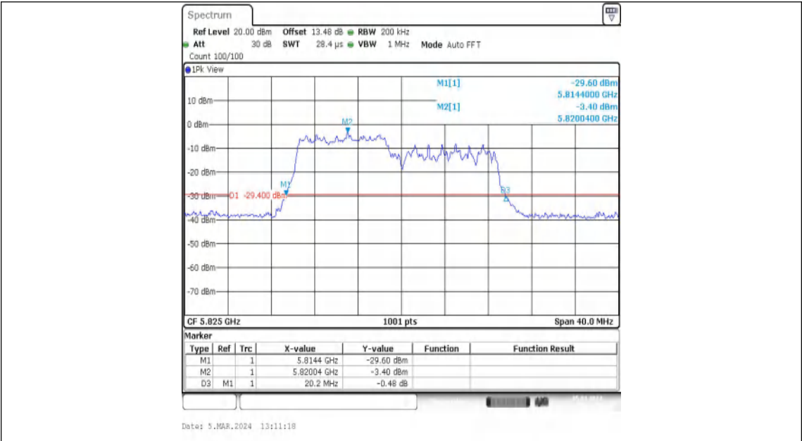
11AX20MIMO-Ant1-5825-106Tone-RU53
