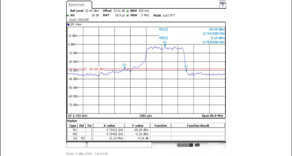
11AX40MIMO-Ant1-5755-242Tone-RU62
