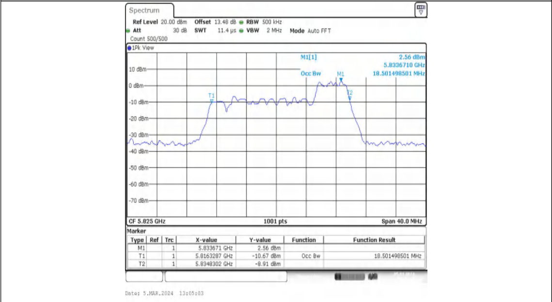
11AX20MIMO-Ant1-5825-52Tone-RU40
