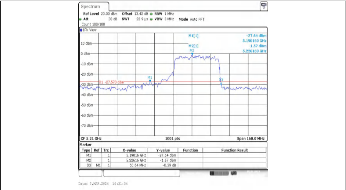
11AX80MIMO-Ant1-5210-484Tone-RU66
