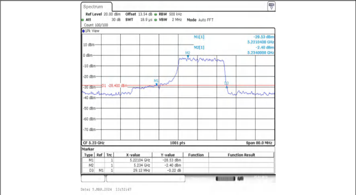
11AX40MIMO-Ant2-5230-242Tone-RU62
