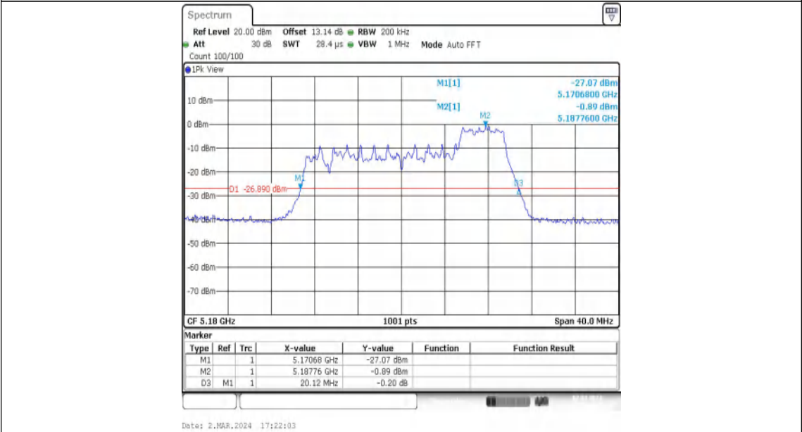
11AX20MIMO-Ant1-5180-52Tone-RU40
