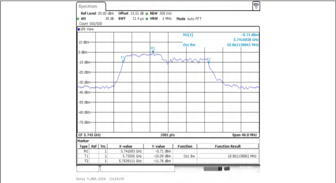
11AX20MIMO-Ant2-5745-106Tone-RU53
