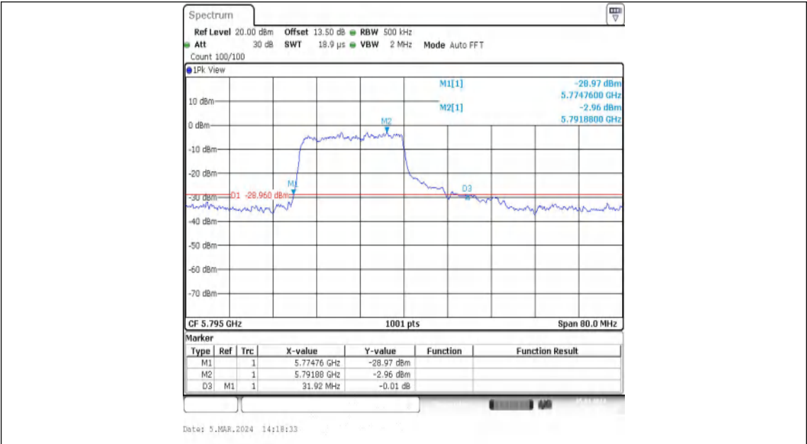
11AX40MIMO-Ant2-5795-242Tone-RU61
