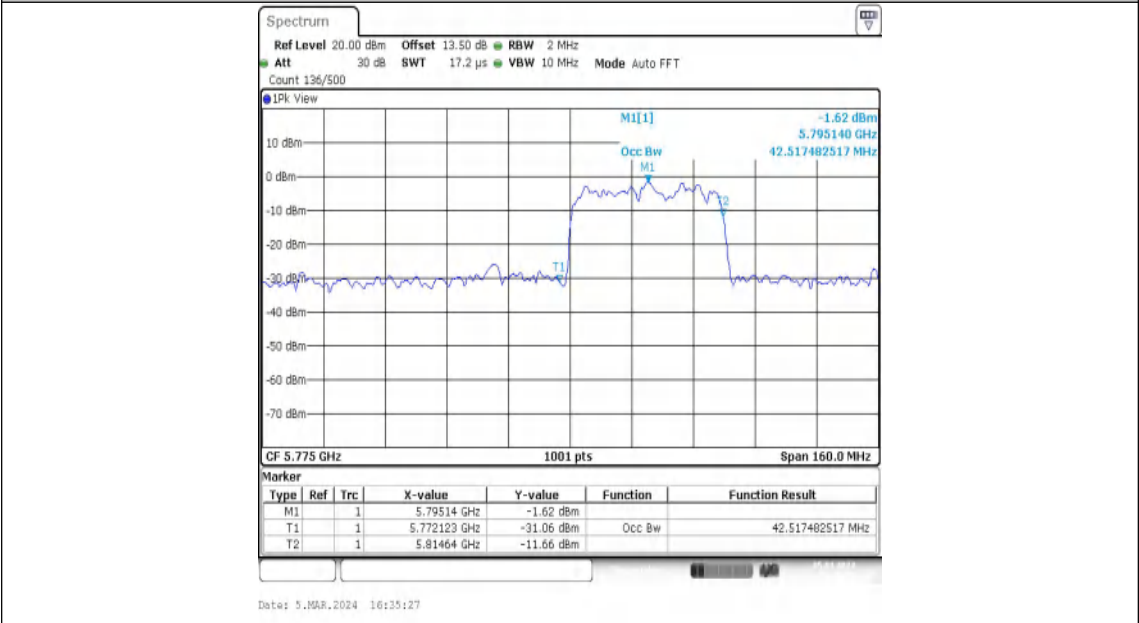
11AX80MIMO-Ant2-5775-484Tone-RU66
