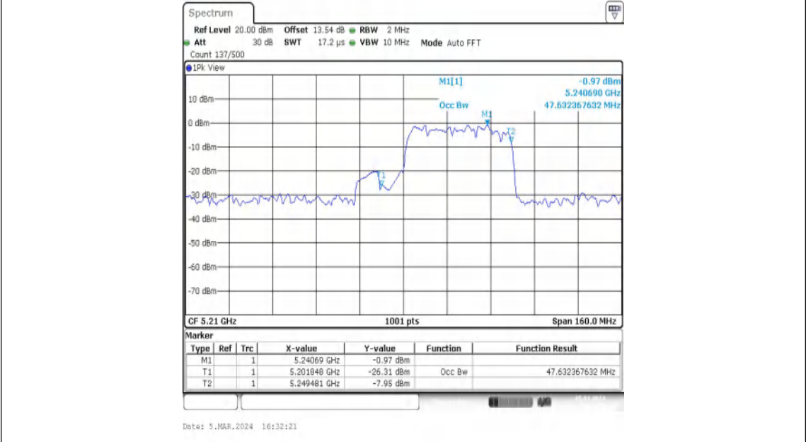
11AX80MIMO-Ant2-5210-484Tone-RU66
