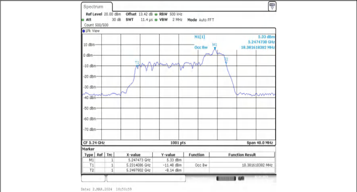
11AX20MIMO-Ant1-5240-52Tone-RU40
