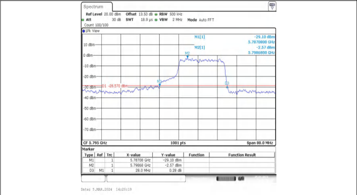
11AX40MIMO-Ant2-5795-242Tone-RU62
