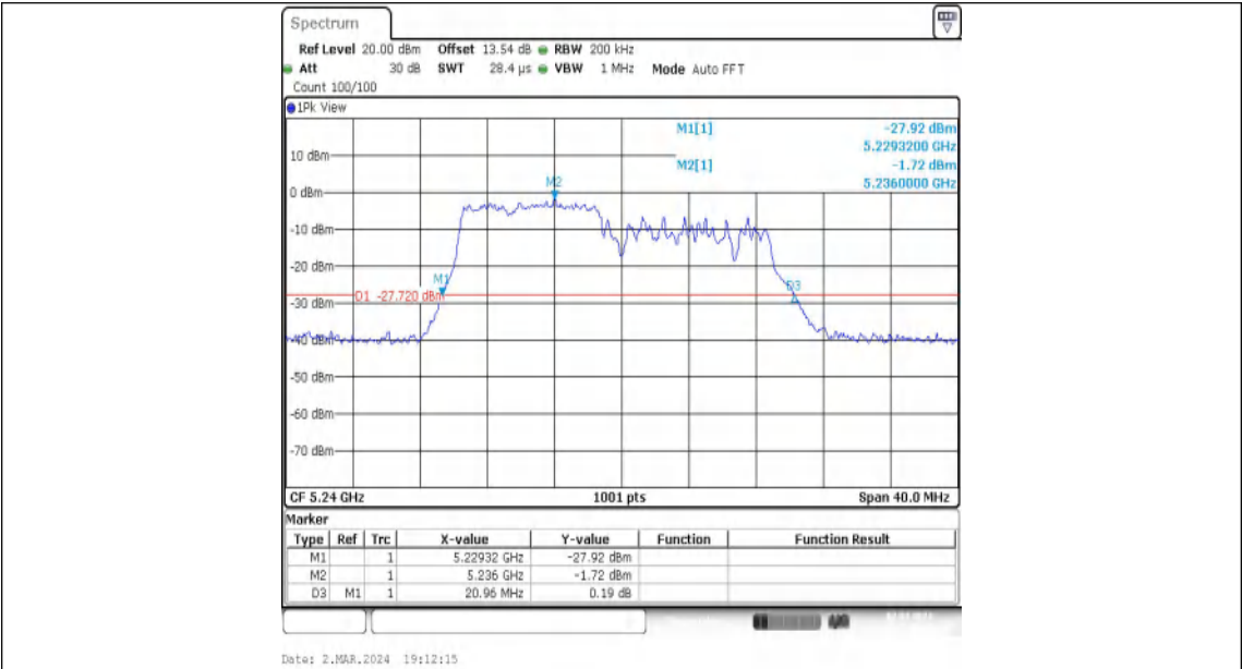
11AX20MIMO-Ant2-5240-106Tone-RU53
