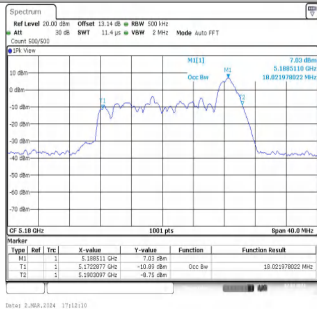
11AX20MIMO-Ant1-5180-26Tone-RU8
