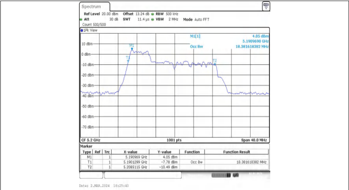
11AX20MIMO-Ant2-5200-52Tone-RU37
