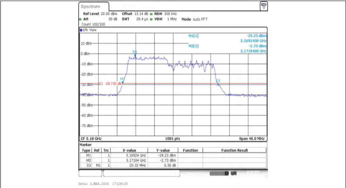
11AX20MIMO-Ant1-5180-106Tone-RU53
