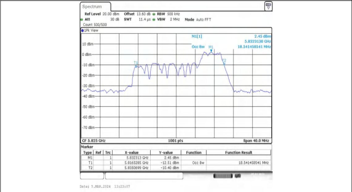
11AX20MIMO-Ant2-5825-52Tone-RU40
