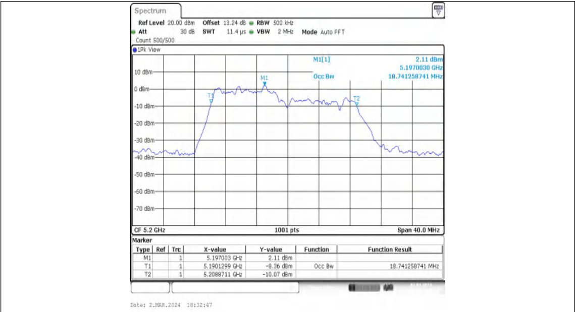
11AX20MIMO-Ant2-5200-106Tone-RU53
