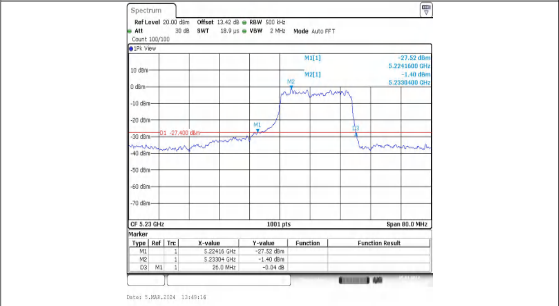
11AX40MIMO-Ant1-5230-242Tone-RU62
