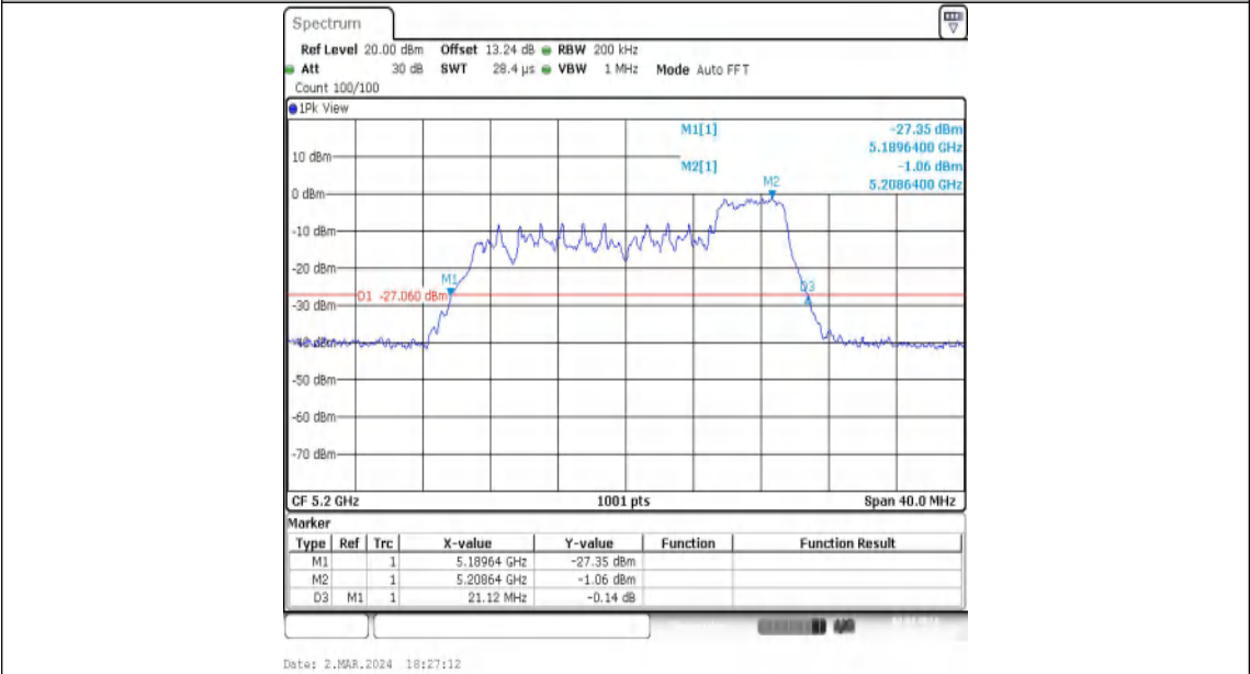
11AX20MIMO-Ant2-5200-52Tone-RU40
