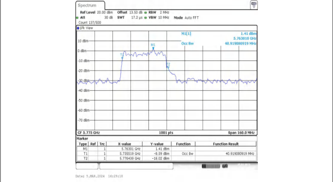
11AX80MIMO-Ant2-5775-484Tone-RU65
