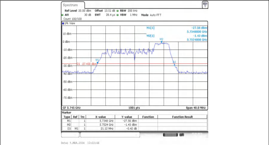
11AX20MIMO-Ant2-5745-52Tone-RU40
