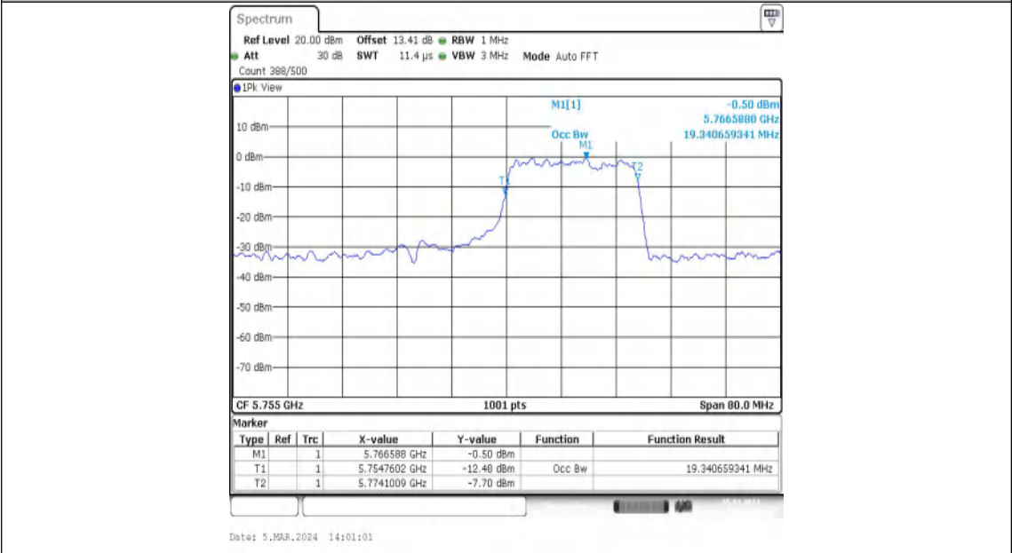
11AX40MIMO-Ant1-5755-242Tone-RU62
