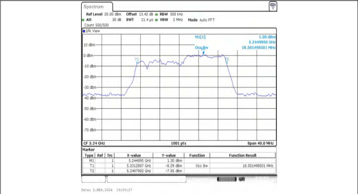
11AX20MIMO-Ant1-5240-106Tone-RU54
