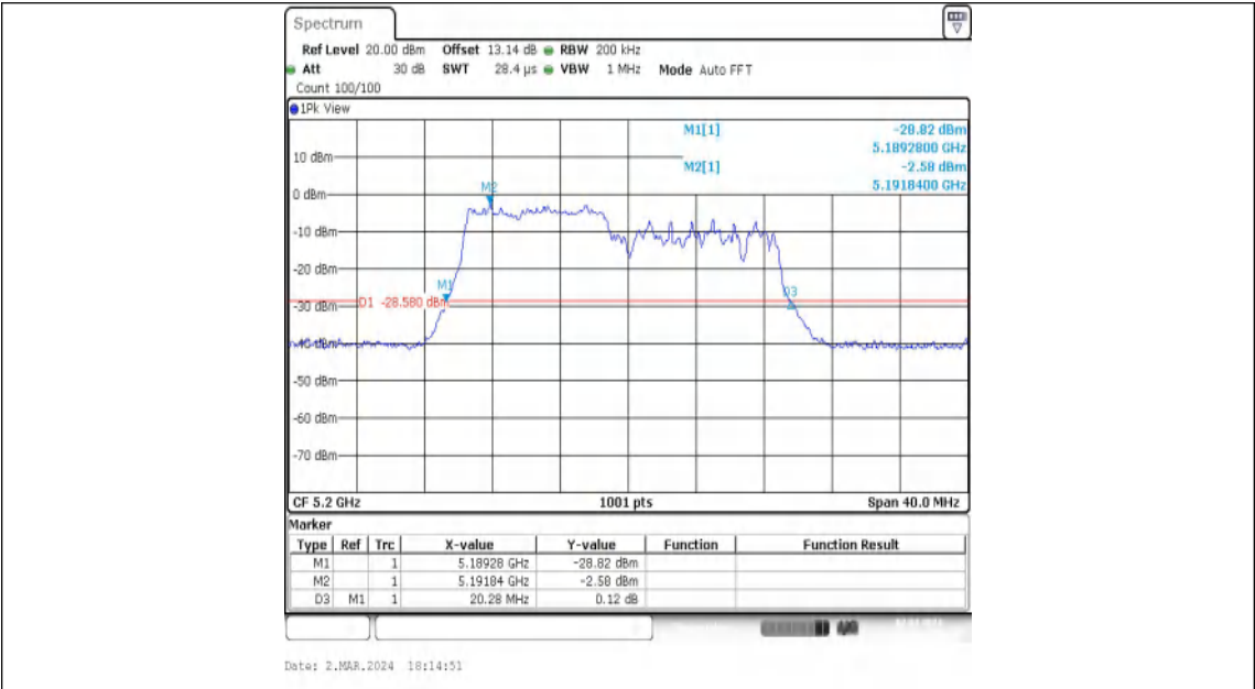
11AX20MIMO-Ant1-5200-106Tone-RU53
