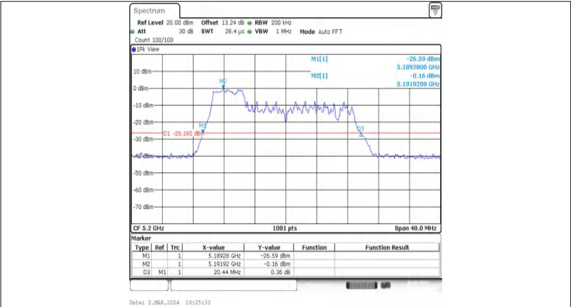
11AX20MIMO-Ant2-5200-52Tone-RU37
