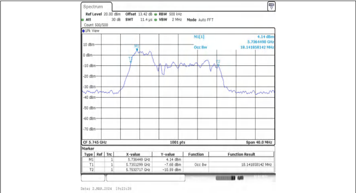
11AX20MIMO-Ant1-5745-52Tone-RU37
