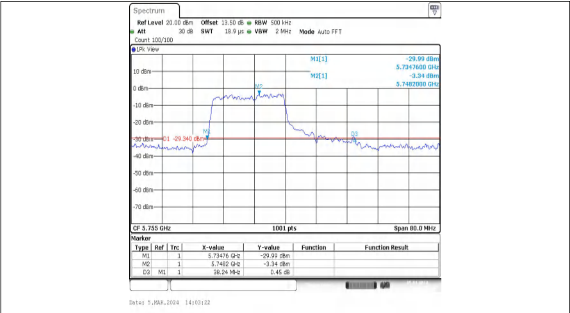
11AX40MIMO-Ant2-5755-242Tone-RU61
