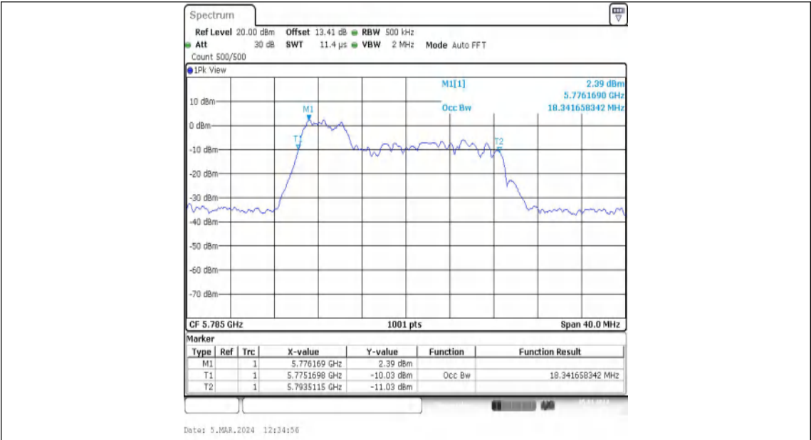
11AX20MIMO-Ant1-5785-52Tone-RU37
