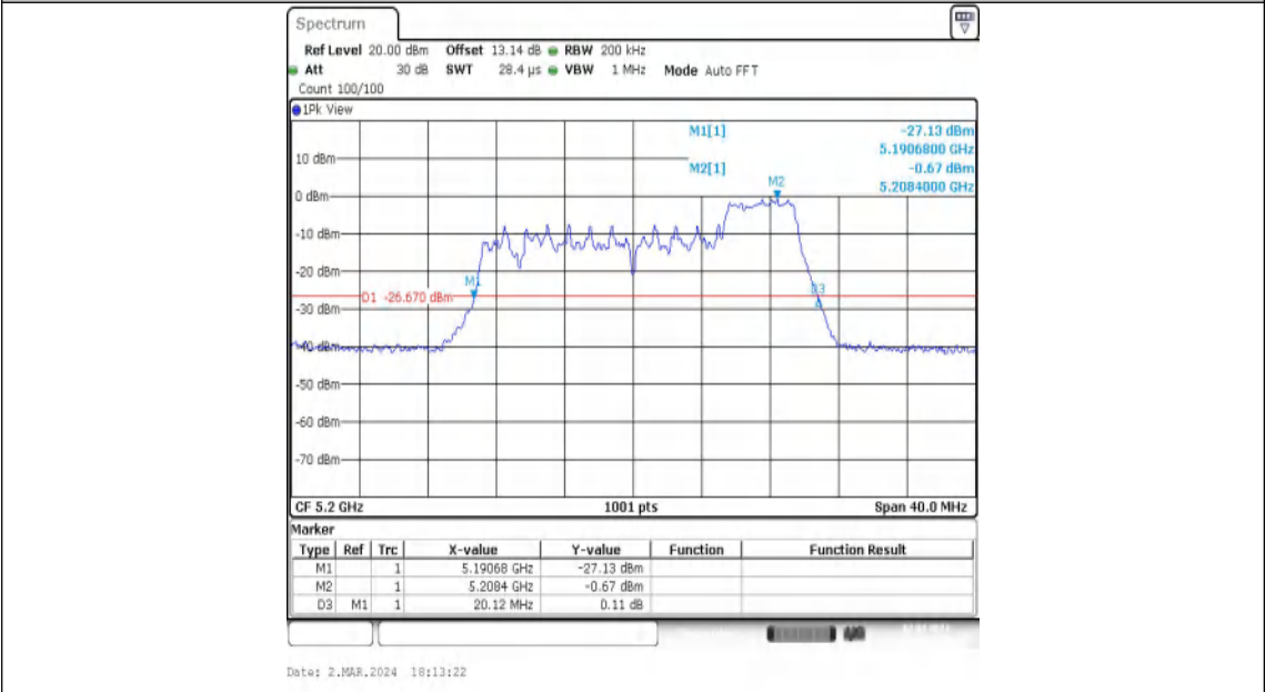
11AX20MIMO-Ant1-5200-52Tone-RU40
