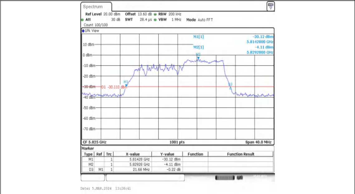
11AX20MIMO-Ant2-5825-106Tone-RU54
