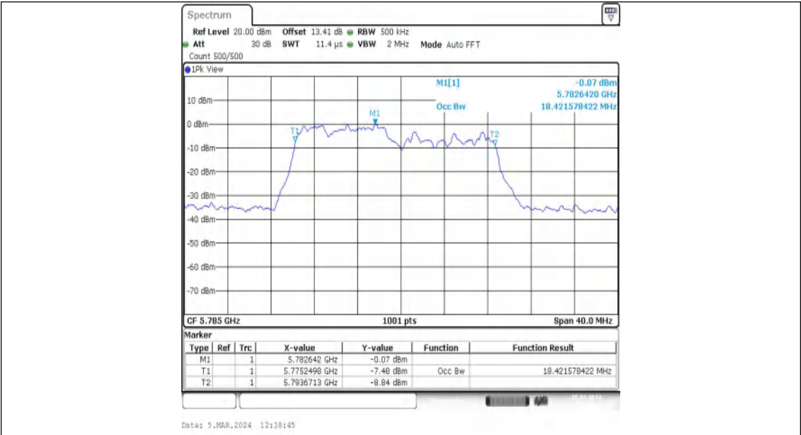
11AX20MIMO-Ant1-5785-106Tone-RU53
