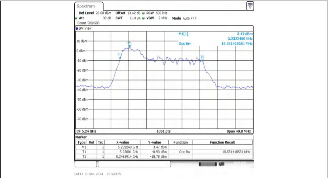
11AX20MIMO-Ant1-5240-52Tone-RU37
