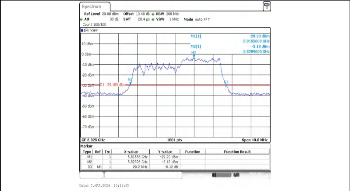
11AX20MIMO-Ant1-5825-106Tone-RU54
