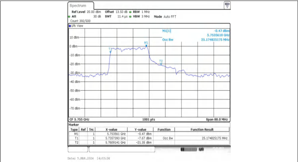
11AX40MIMO-Ant2-5755-242Tone-RU61
