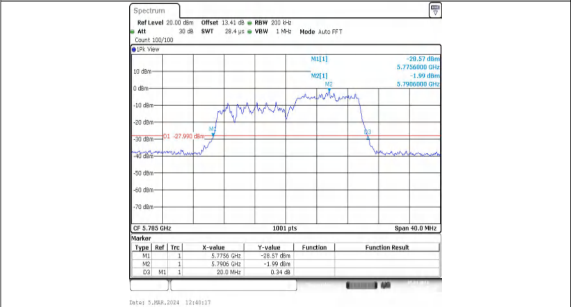
11AX20MIMO-Ant1-5785-106Tone-RU54
