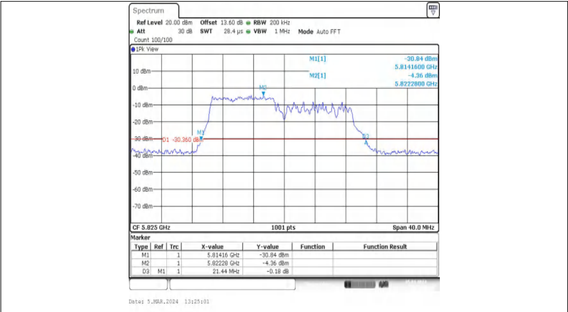
11AX20MIMO-Ant2-5825-106Tone-RU53
