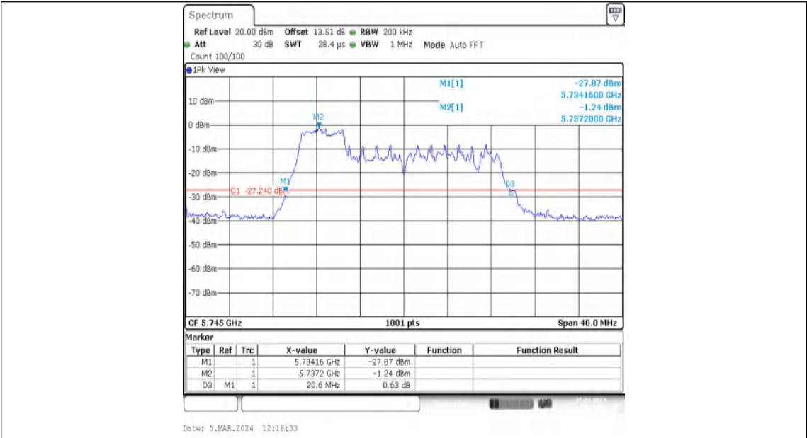
11AX20MIMO-Ant2-5745-52Tone-RU37
