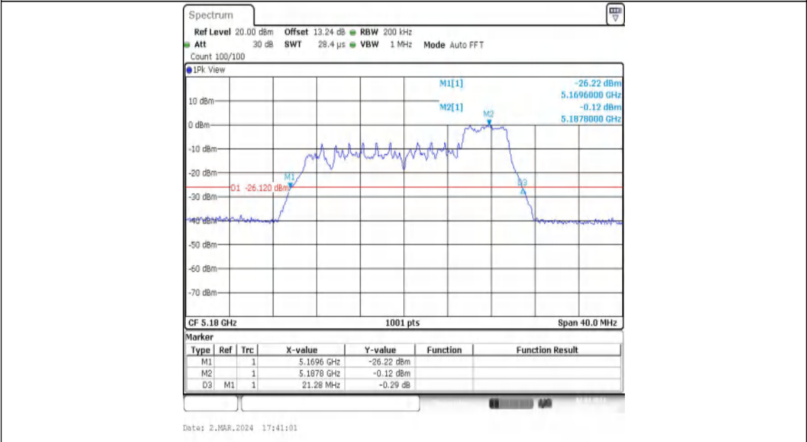
11AX20MIMO-Ant2-5180-52Tone-RU40
