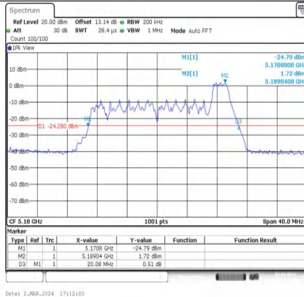
11AX20MIMO-Ant1-5180-26Tone-RU8
