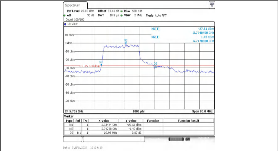
11AX40MIMO-Ant1-5755-242Tone-RU61
