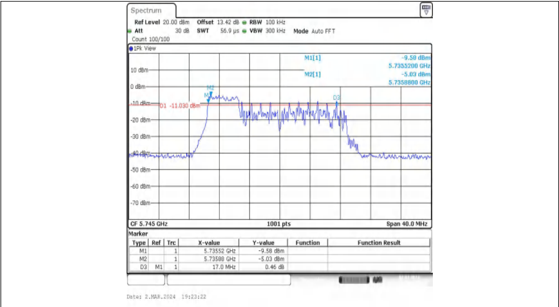
11AX20MIMO-Ant1-5745-52Tone-RU37-PASS
