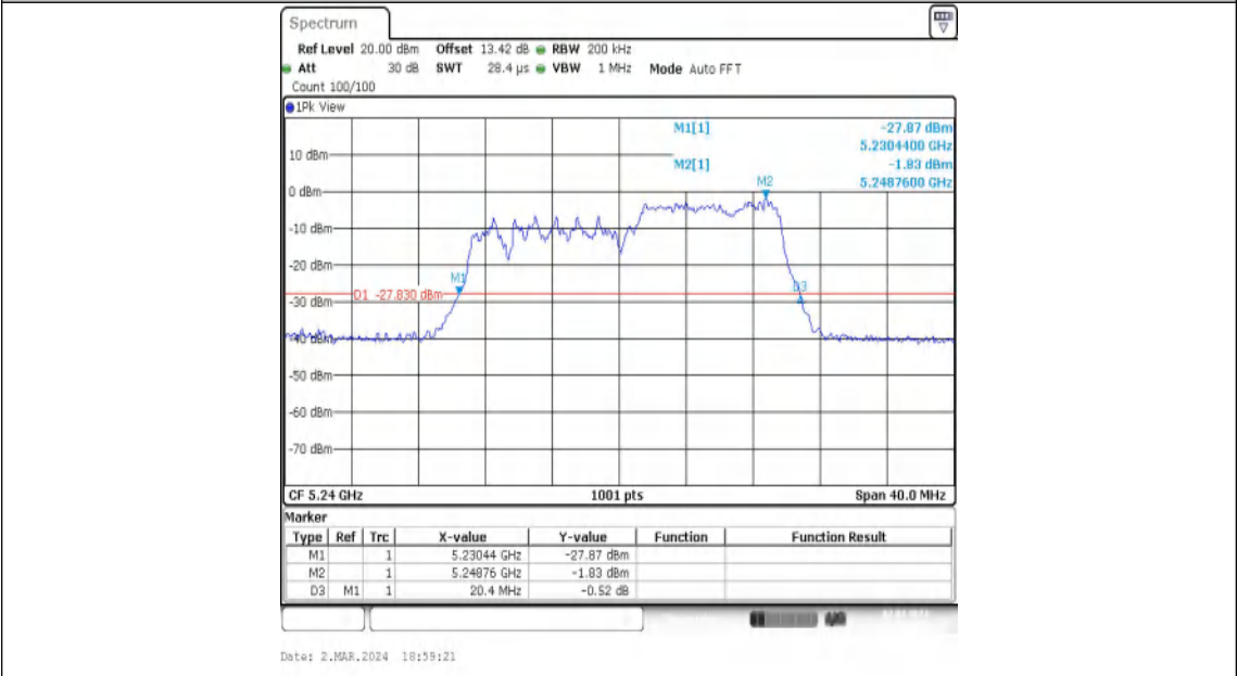
11AX20MIMO-Ant1-5240-106Tone-RU54
