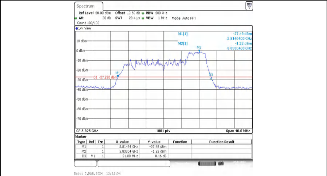
11AX20MIMO-Ant2-5825-52Tone-RU40
