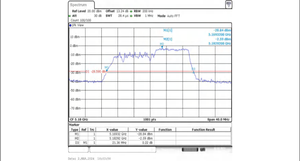
11AX20MIMO-Ant2-5180-106Tone-RU54
