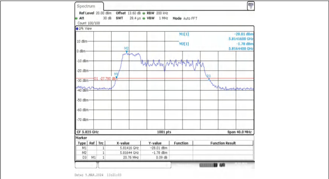
11AX20MIMO-Ant2-5825-52Tone-RU37
