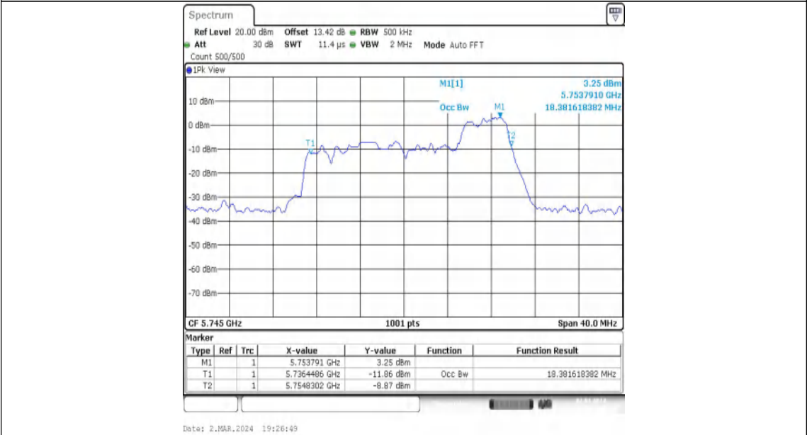
11AX20MIMO-Ant1-5745-52Tone-RU40
