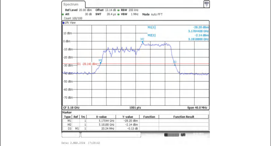
11AX20MIMO-Ant1-5180-106Tone-RU54
