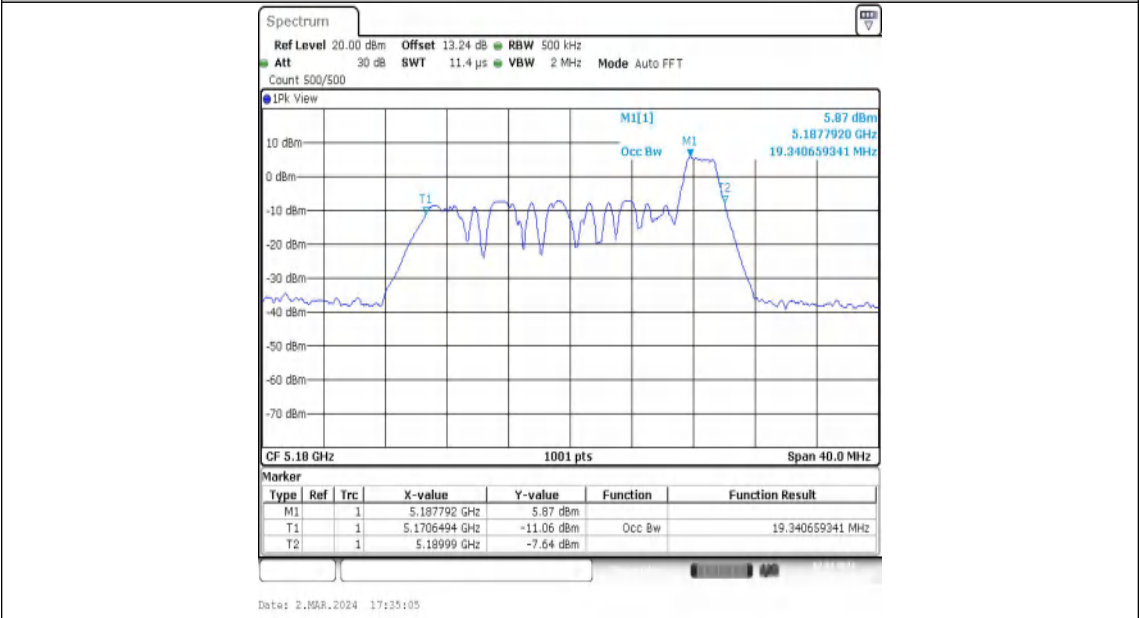
11AX20MIMO-Ant2-5180-26Tone-RU8
