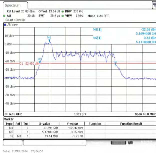
11AX20MIMO-Ant1-5180-26Tone-RU0
