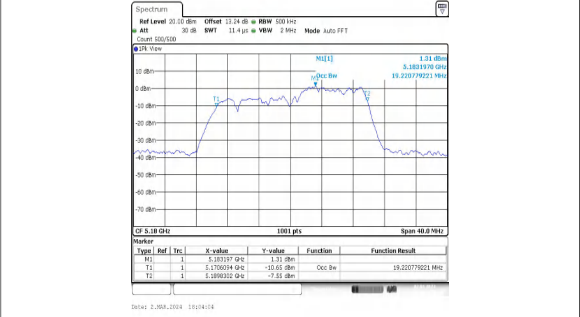
11AX20MIMO-Ant2-5180-106Tone-RU54
