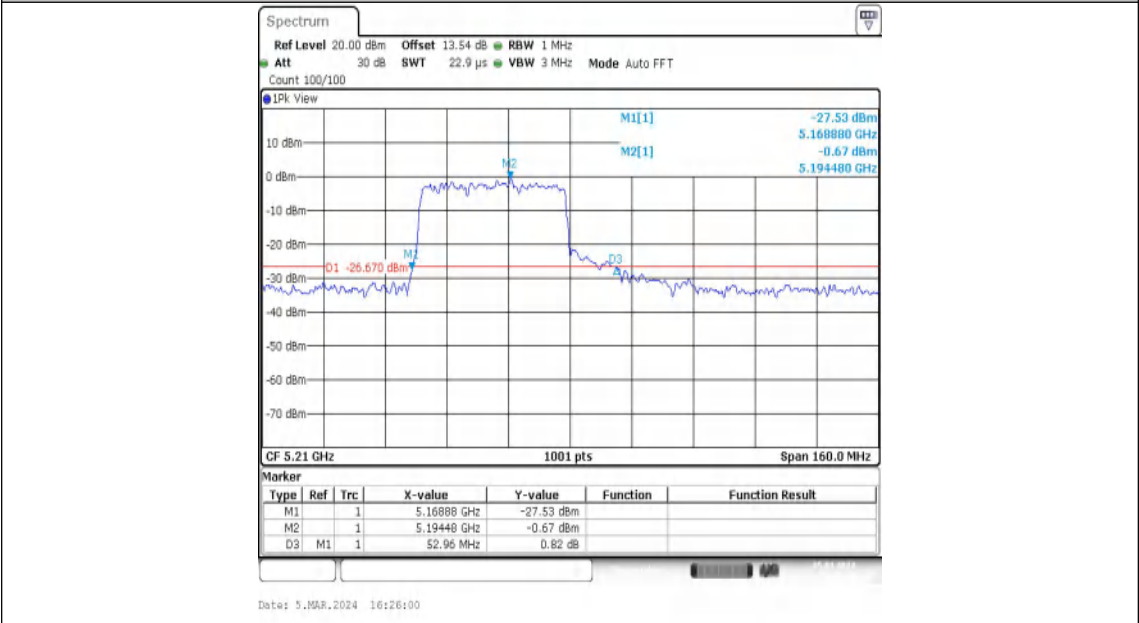
11AX80MIMO-Ant2-5210-484Tone-RU65
