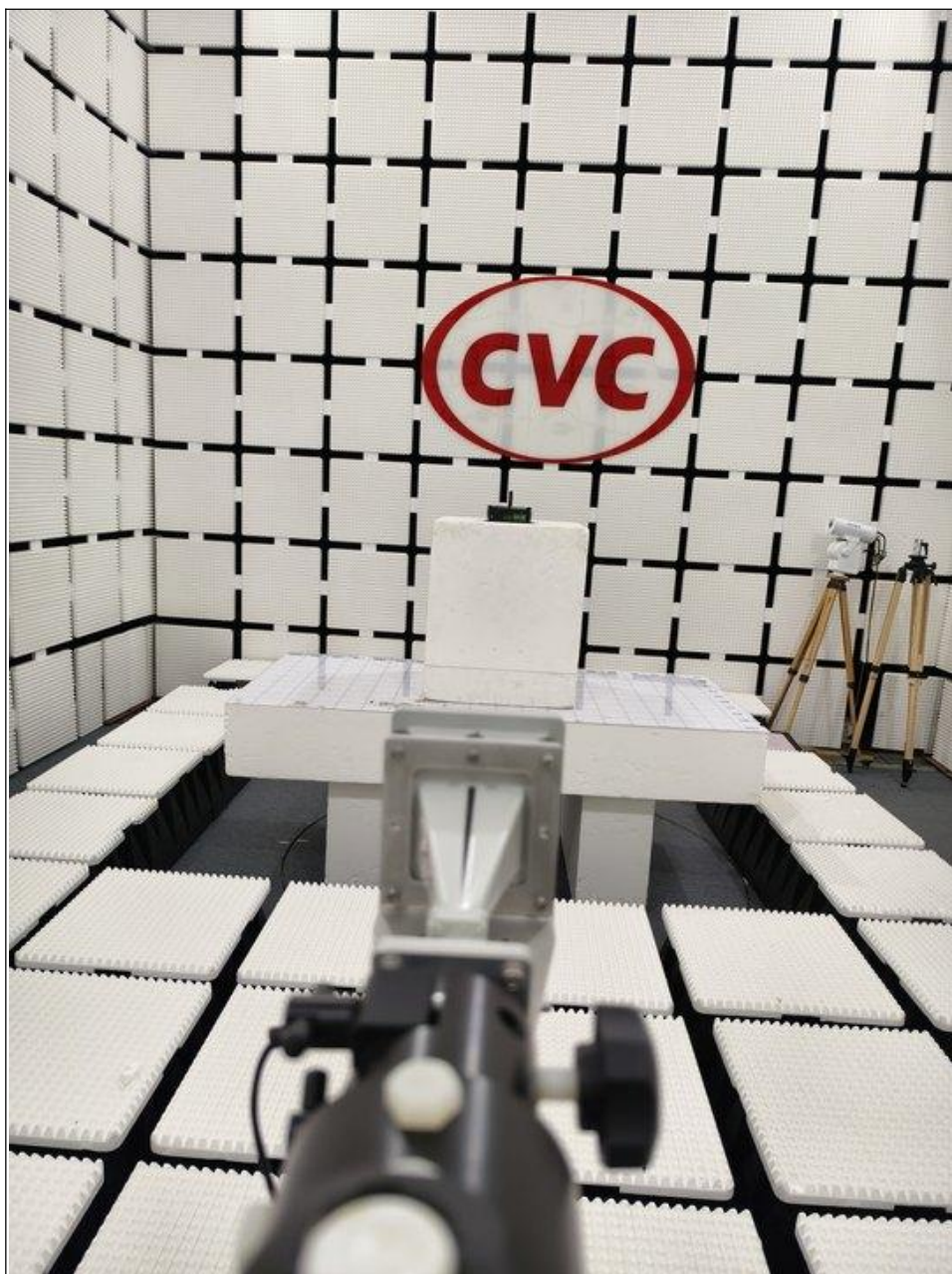
RADIATED EMISSION TEST (18-40GHz)
