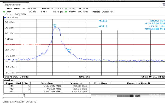
802.11ah 1M_Ant1_High_926.5
