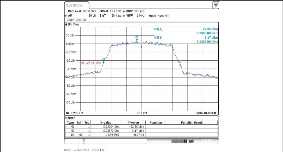
11A-Ant1-5240
