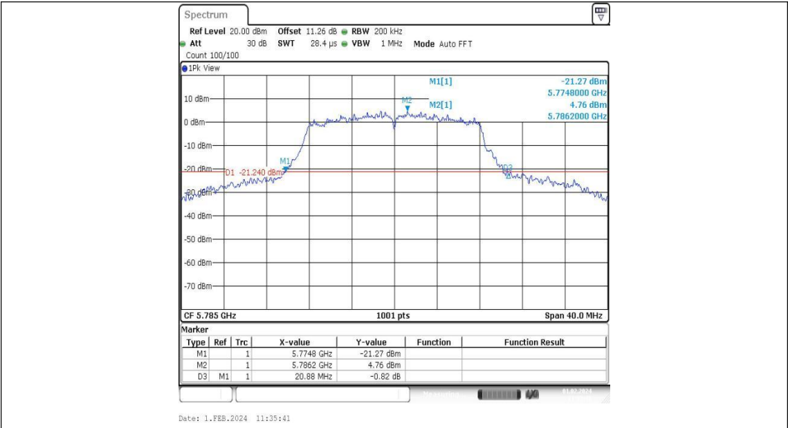
11A-Ant1-5785
