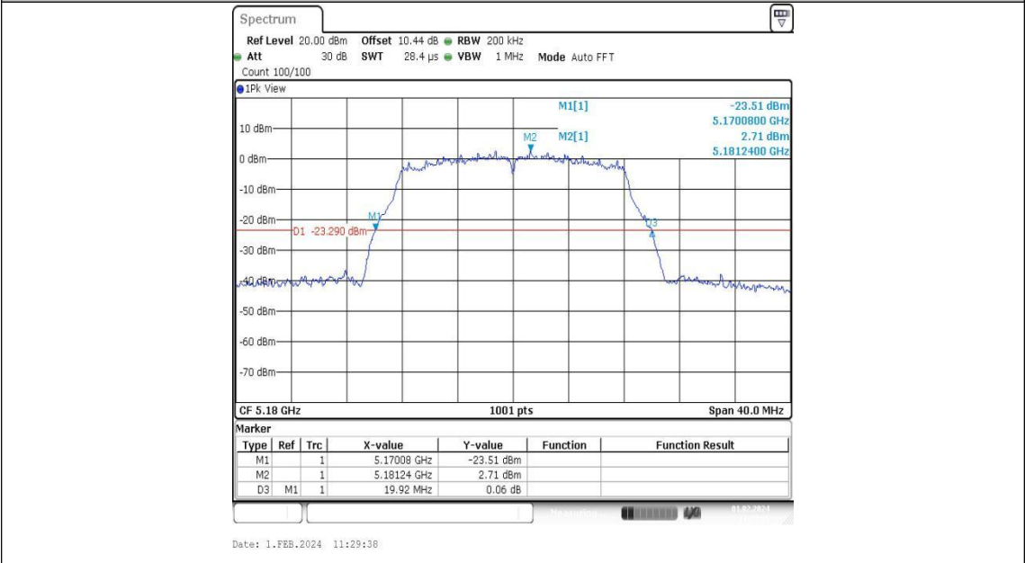
11A-Ant1-5180
