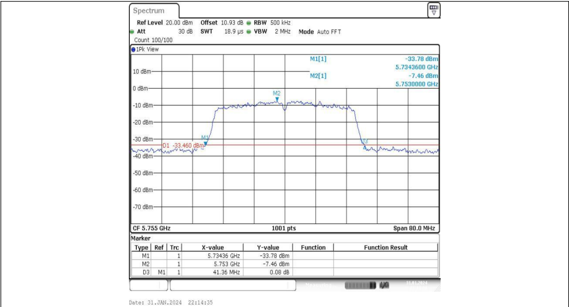
11N40MIMO-Ant2-5755
