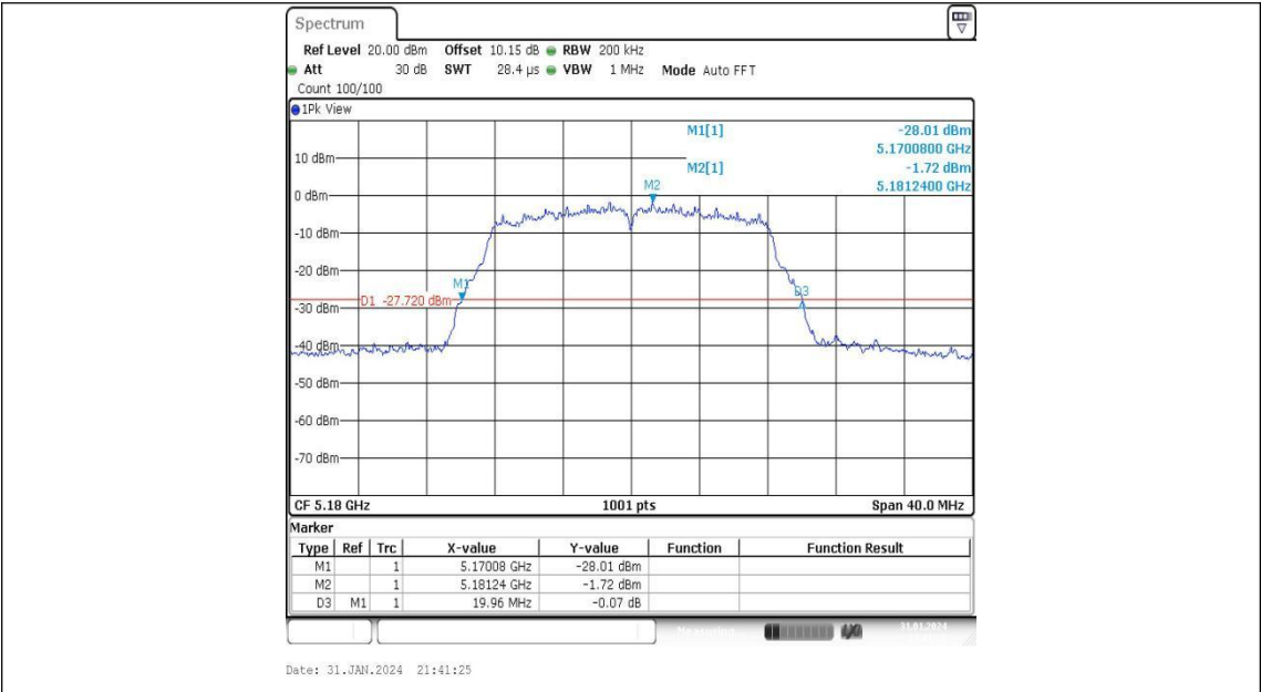
11A-Ant2-5180
