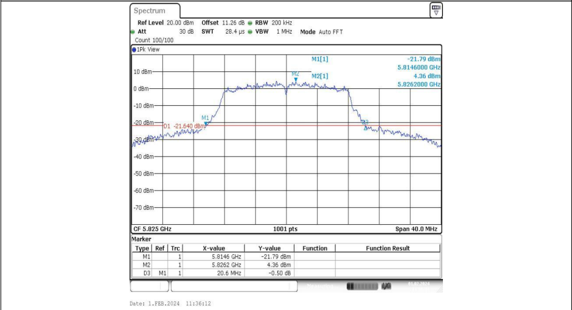
11A-Ant1-5825
