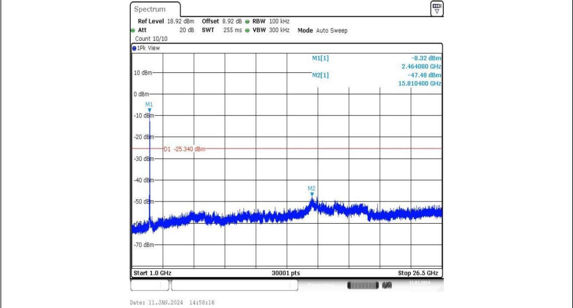
11N20MIMO-Ant2-2462-1000~26500
