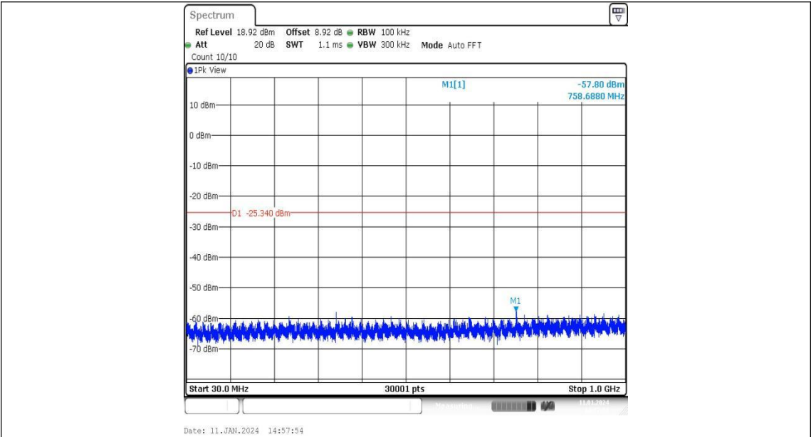
11N20MIMO-Ant2-2462-30~1000
