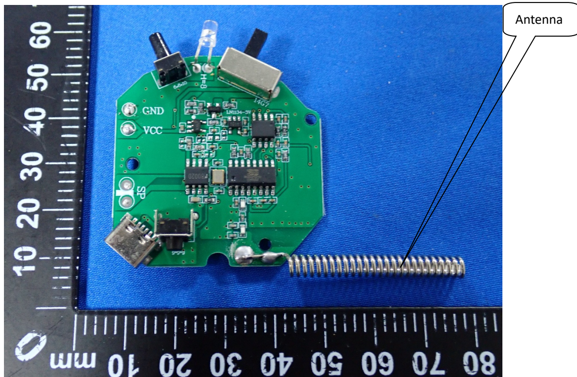
Internal Photo 5
