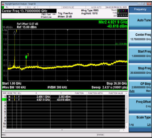
11N20SISO-Ant1-2462-1000~26500-PASS
