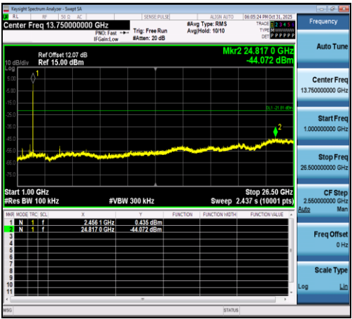
11AX20SISO-Ant1-2462-1000~26500-PASS
