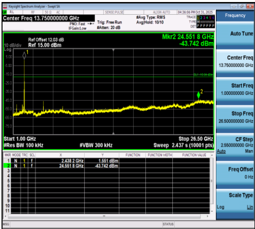
11N20SISO-Ant1-2437-1000~26500-PASS
