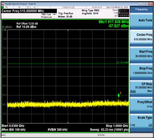
11AX40SISO-Ant1-2422-30~1000-PASS
