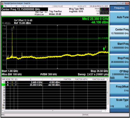
11N40SISO-Ant1-2452-1000~26500-PASS
