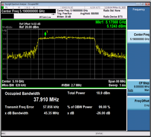
11AX40SISO-Ant1-5190
