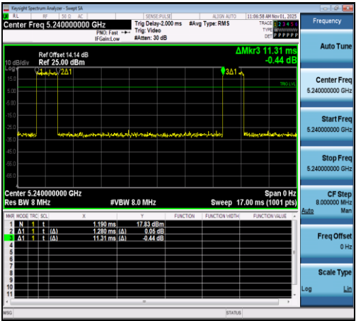
NTNV-11AC20SISO-Ant1-5240
