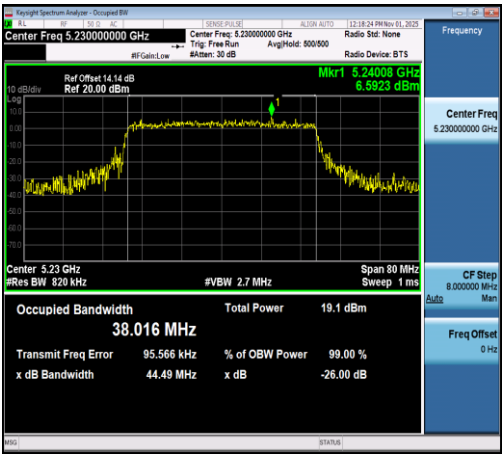
11AX40SISO-Ant1-5230
