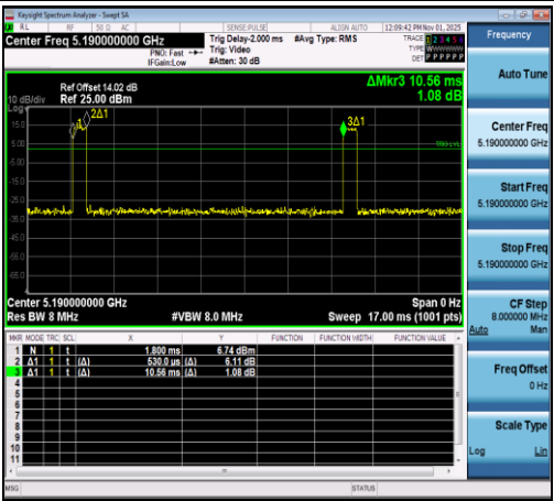
NTNV-11AX40SISO-Ant1-5190
