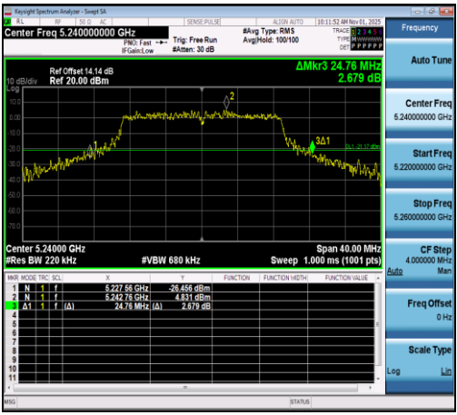
11N20SISO-Ant1-5240
