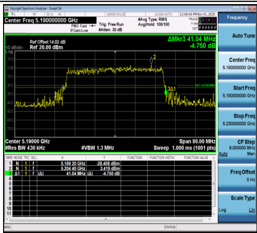
11AX40SISO-Ant1-5190
