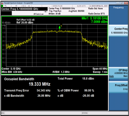
11AX20SISO-Ant1-5180
