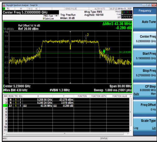
11N40SISO-Ant1-5230
