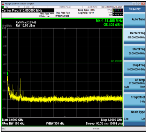
LE_1M-Ant1-2440-30~1000-PASS
