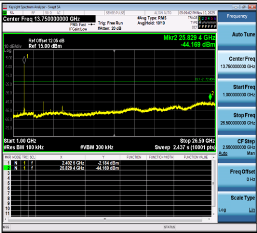
LE_1M-Ant1-2402-1000~26500-PASS
