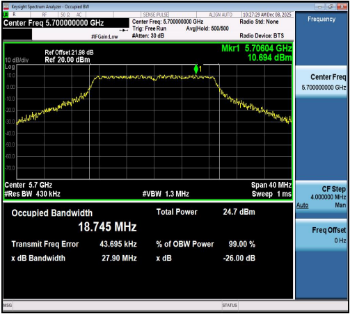
11N20SISO-Ant1-5700
