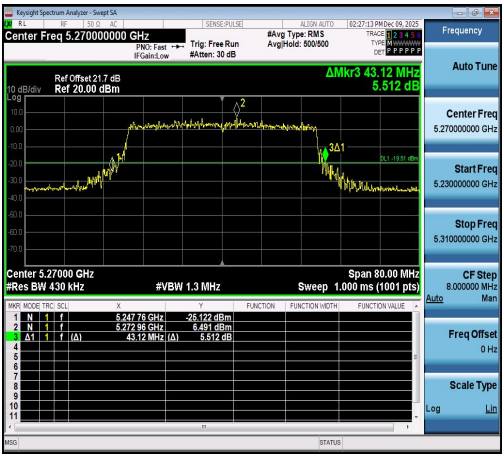
11AX40SISO-Ant1-5270
