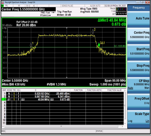
11AX40SISO-Ant1-5550
