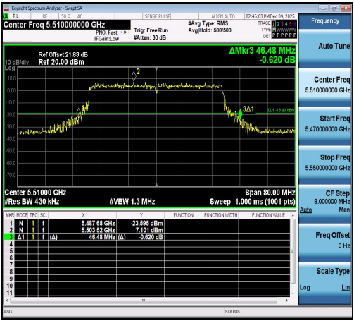
11AX40SISO-Ant1-5510
