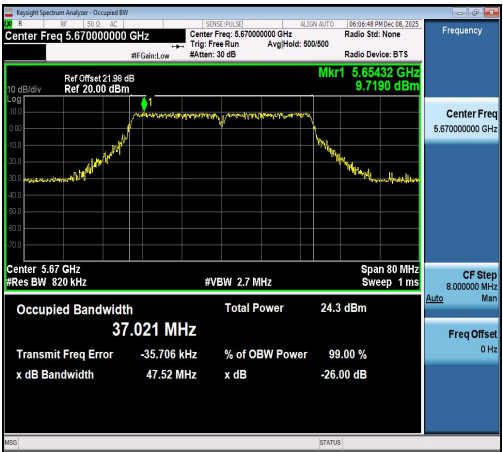
11AC40SISO-Ant1-5670
