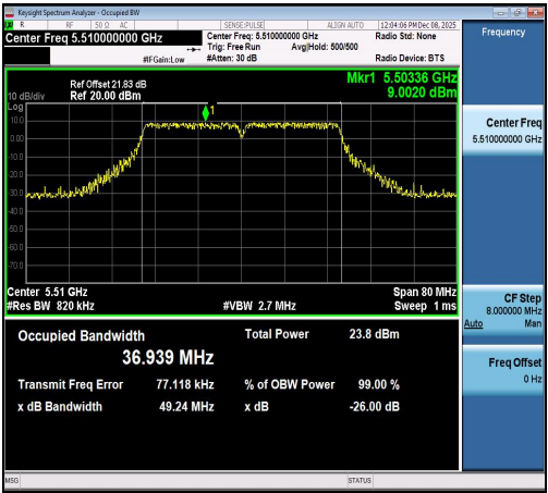
11N40SISO-Ant1-5510
