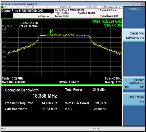
11AX20SISO-Ant1-5280
