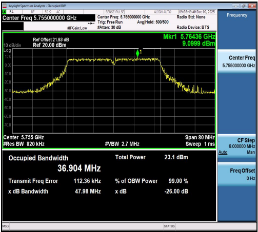
11AC40SISO-Ant1-5755
