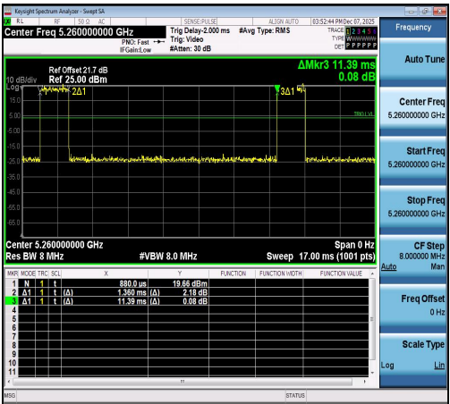
NTNV-11A-Ant1-5260
