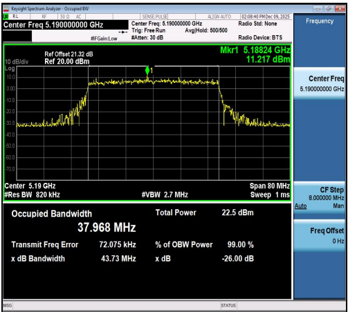
11AX40SISO-Ant1-5190
