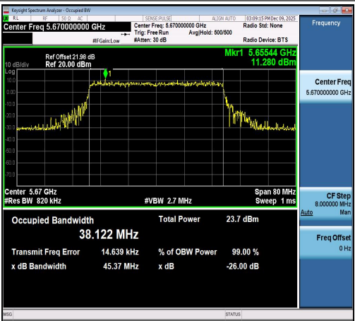
11AX40SISO-Ant1-5670
