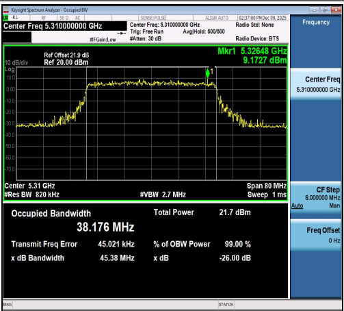
11AX40SISO-Ant1-5310
