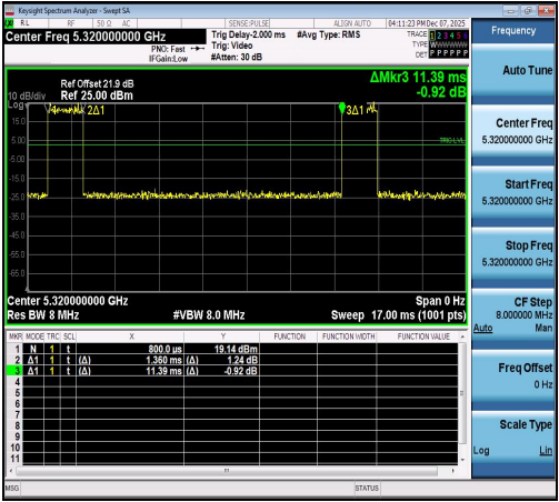
NTNV-11A-Ant1-5320
