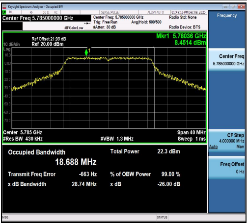
11AX20SISO-Ant1-5785
