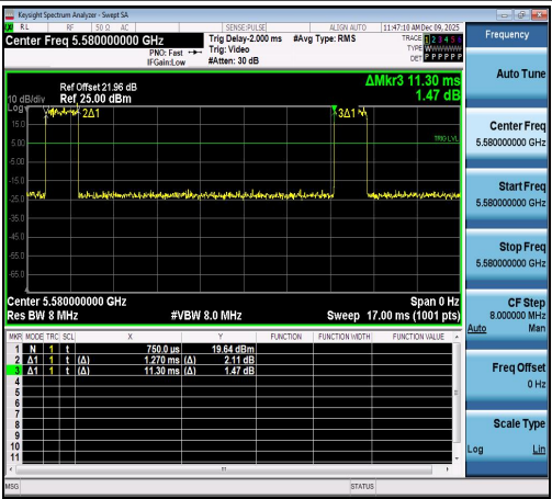
NTNV-11AX20SISO-Ant1-5580
