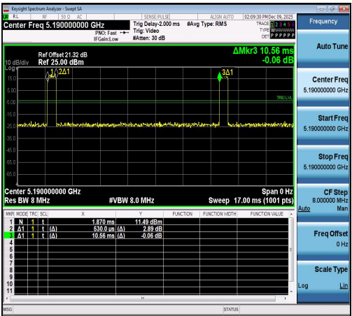
NTNV-11AX40SISO-Ant1-5190
