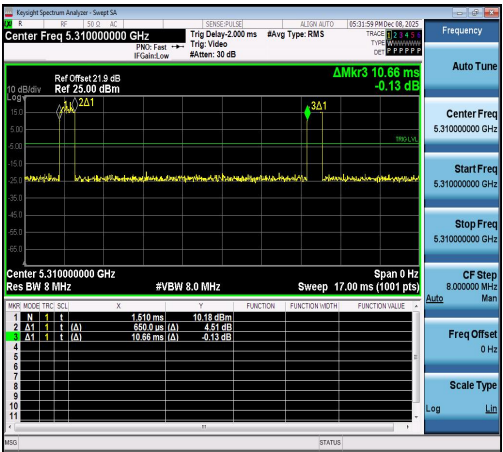
NTNV-11AC40SISO-Ant1-5310
