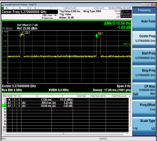
NTNV-11AX40SISO-Ant1-5270
