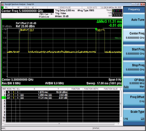
NTNV-11AX20SISO-Ant1-5500
