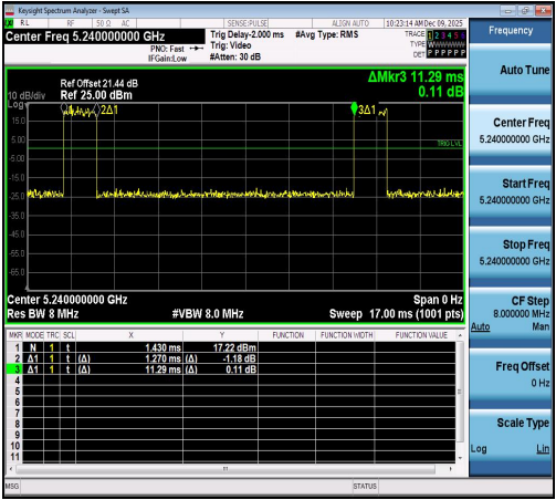
NTNV-11AX20SISO-Ant1-5240
