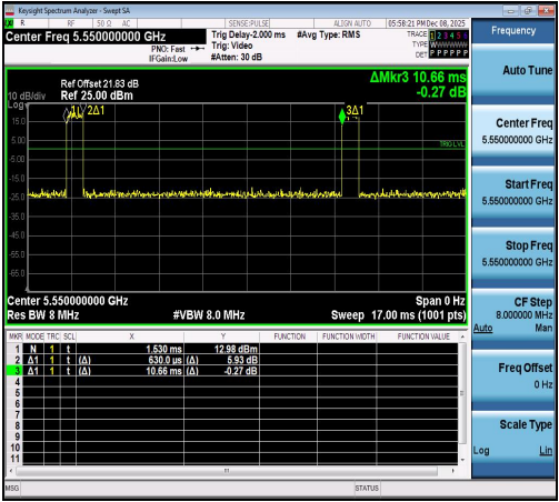
NTNV-11AC40SISO-Ant1-5550
