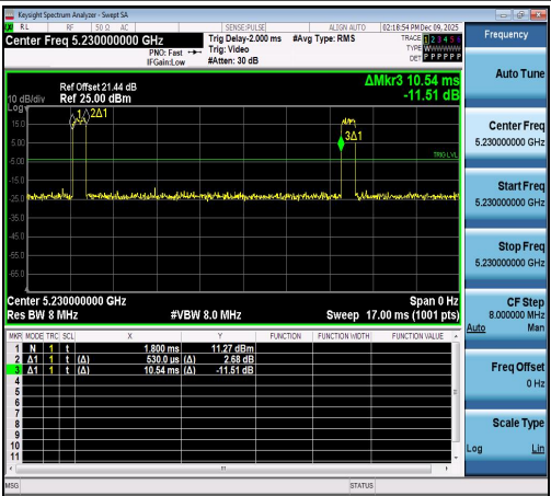
NTNV-11AX40SISO-Ant1-5230
