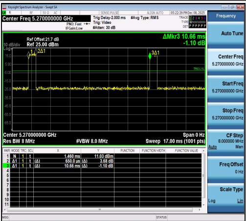
NTNV-11AC40SISO-Ant1-5270
