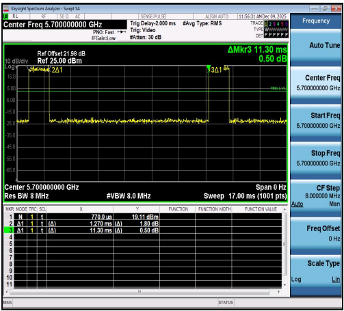
NTNV-11AX20SISO-Ant1-5700
