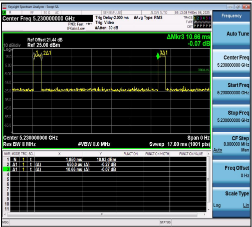
NTNV-11AC40SISO-Ant1-5230
