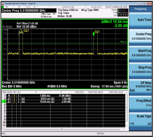
NTNV-11AX40SISO-Ant1-5510
