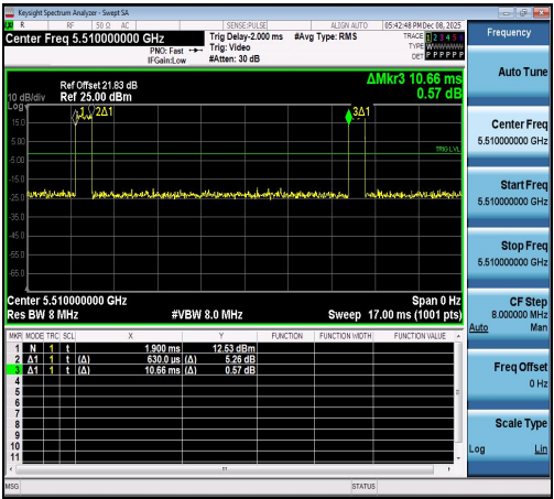
NTNV-11AC40SISO-Ant1-5510
