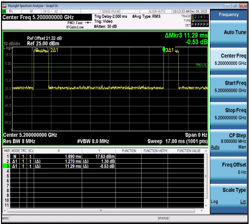
NTNV-11AX20SISO-Ant1-5200
