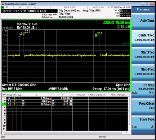
NTNV-11AX40SISO-Ant1-5310
