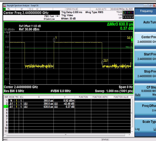
NTNV-LE_1M-Ant1-2440
