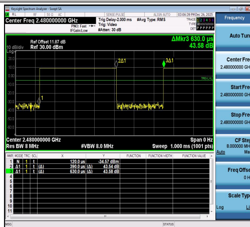
NTNV-LE_1M-Ant1-2480
