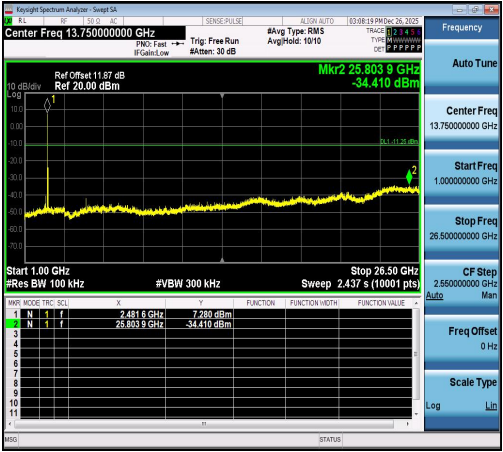
LE_1M-Ant1-2480-1000~26500-PASS
