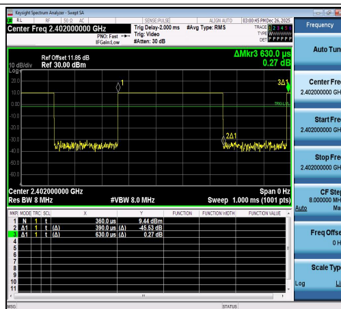
NTNV-LE_1M-Ant1-2402
