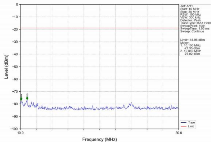
Pi/4DQPSK_2DH5_MCH_2441MHz_Ant1_NTNV
