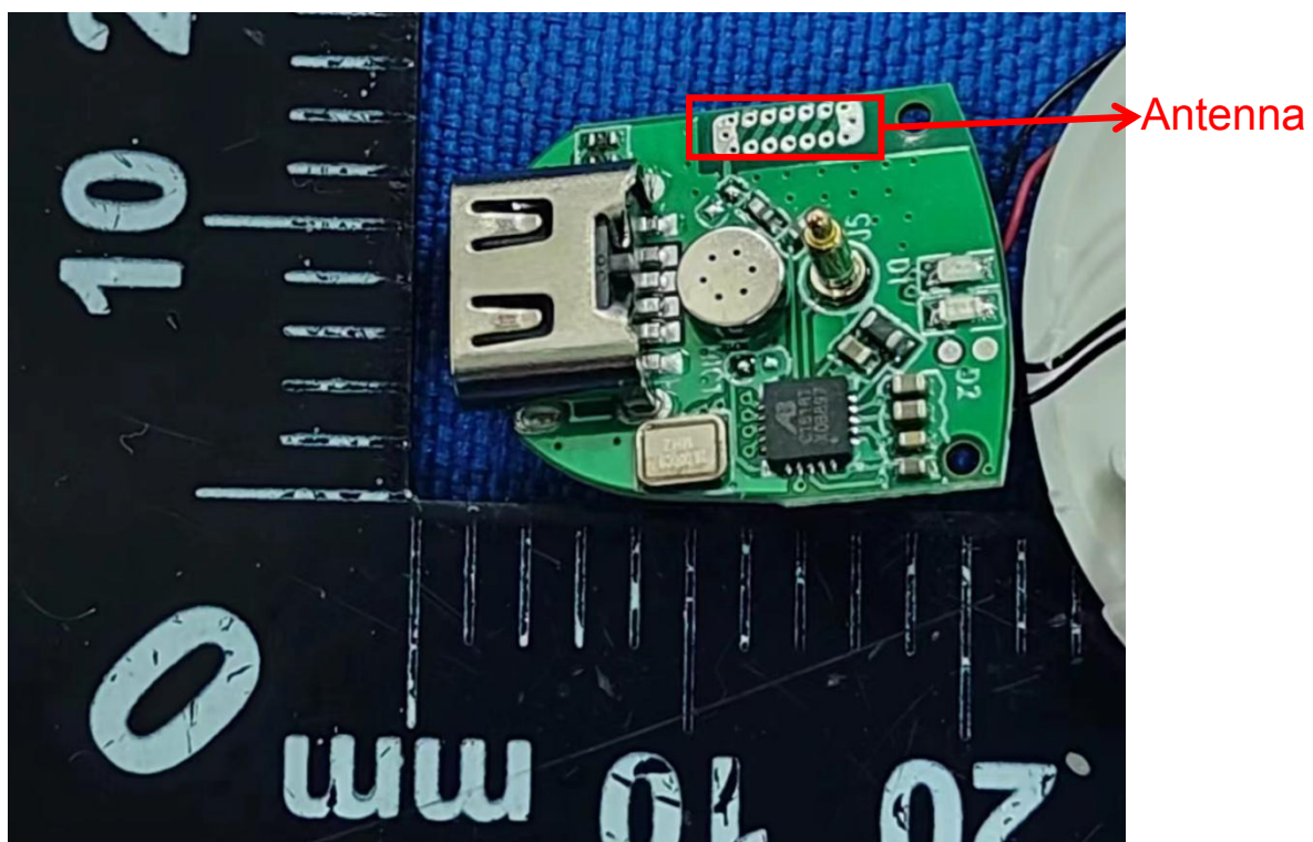
PCB view of unit
