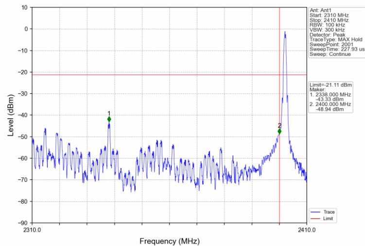
1M_LCH_2402MHz_Ant1_NTNV
