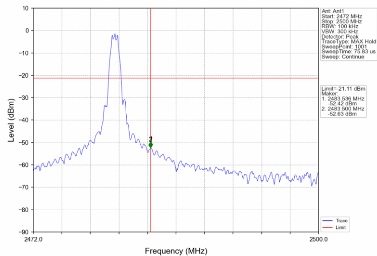
1M_HCH_2480MHz_Ant1_NTNV
