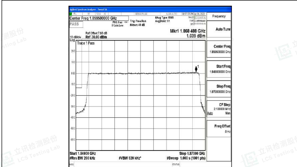
Band2_20MHz_16QAM_18700_100RB#0
