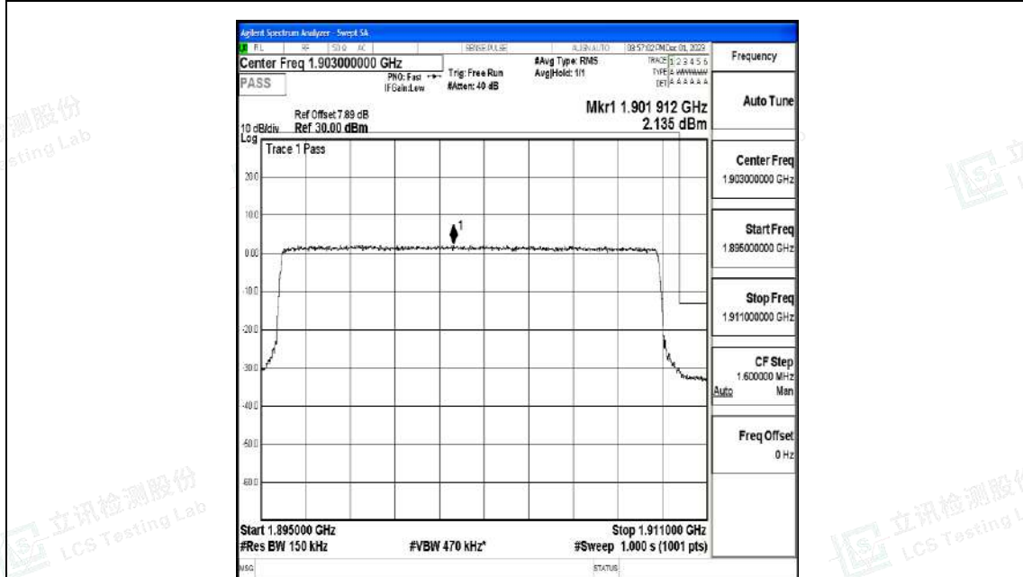
Band2_15MHz_16QAM_19125_75RB#0
