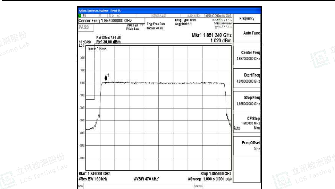
Band2_15MHz_16QAM_18675_75RB#0
