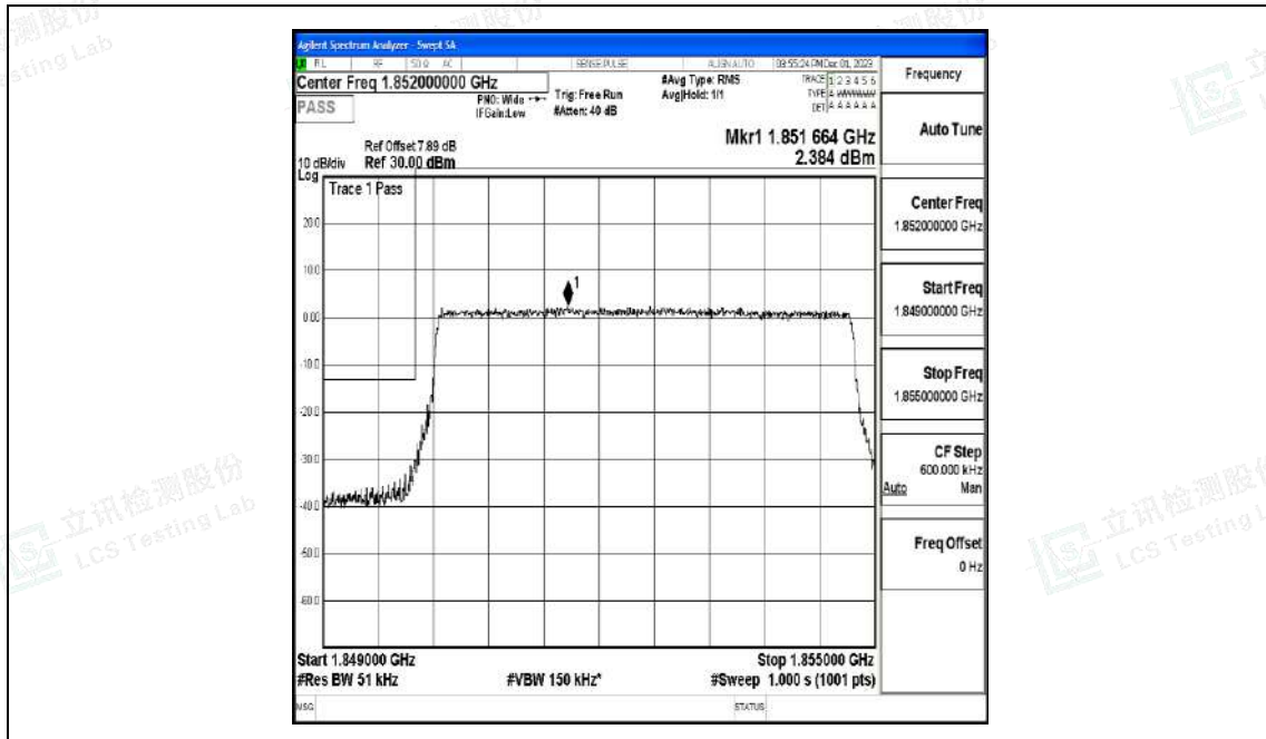
Band2_5MHz_QPSK_18625_25RB#0
