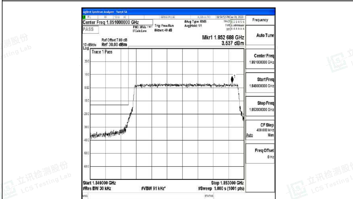
Band2_3MHz_16QAM_18615_15RB#0
