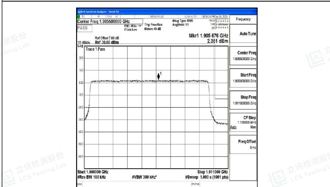
Band2_10MHz_QPSK_19150_50RB#0
