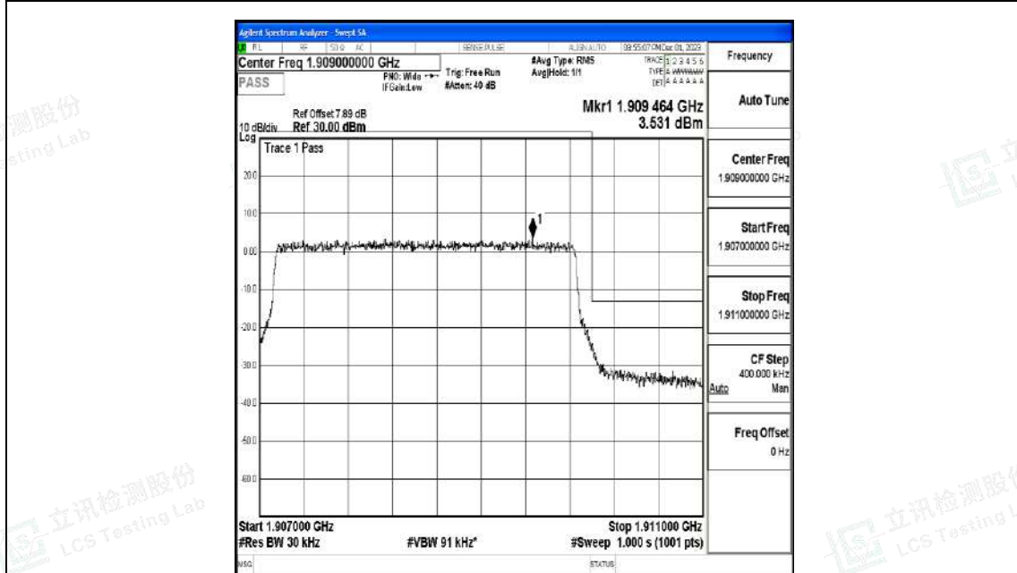
Band2_3MHz_16QAM_19185_15RB#0
