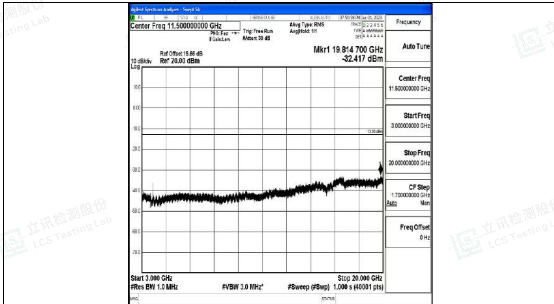
Band2_15MHz_QPSK_19125_1RB#0_3000~20000_3000~20000
