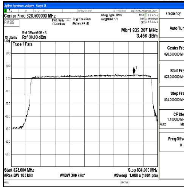
Band5_10MHz_16QAM_20450_50RB#0
