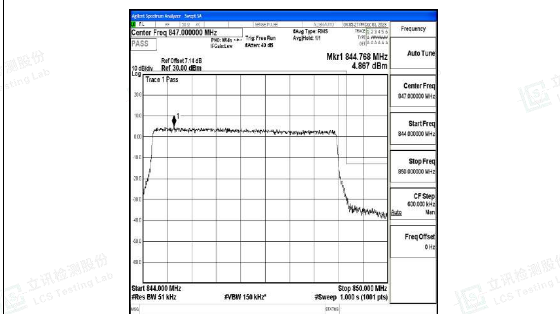
Band5_5MHz_QPSK_20625_25RB#0
