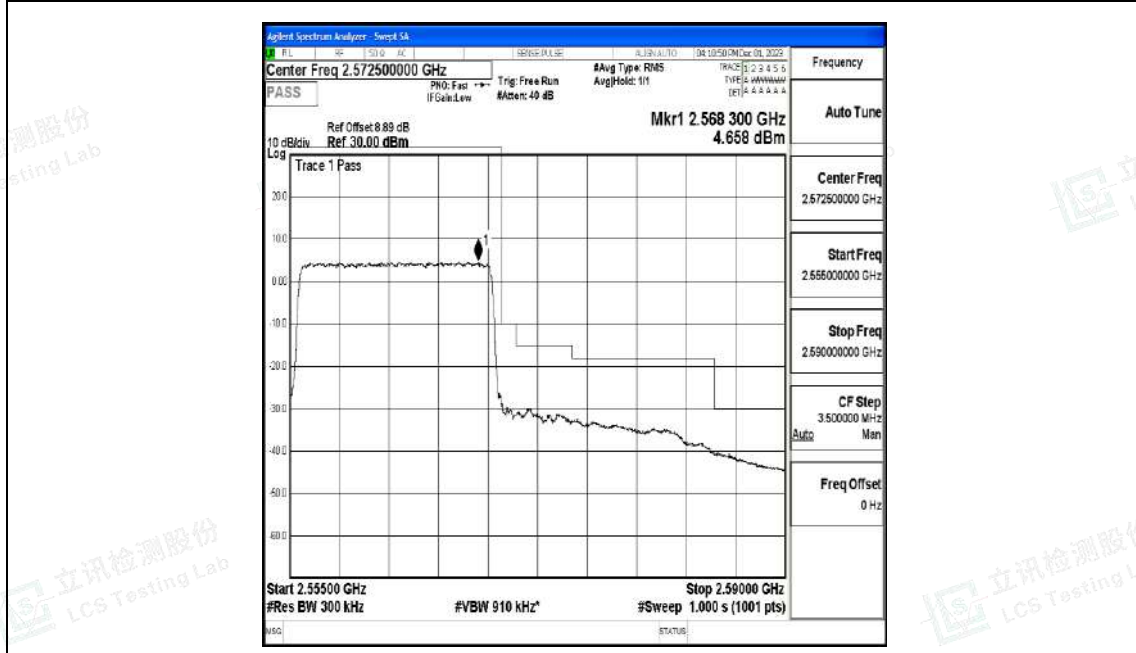
Band7_15MHz_16QAM_21375_75RB#0
