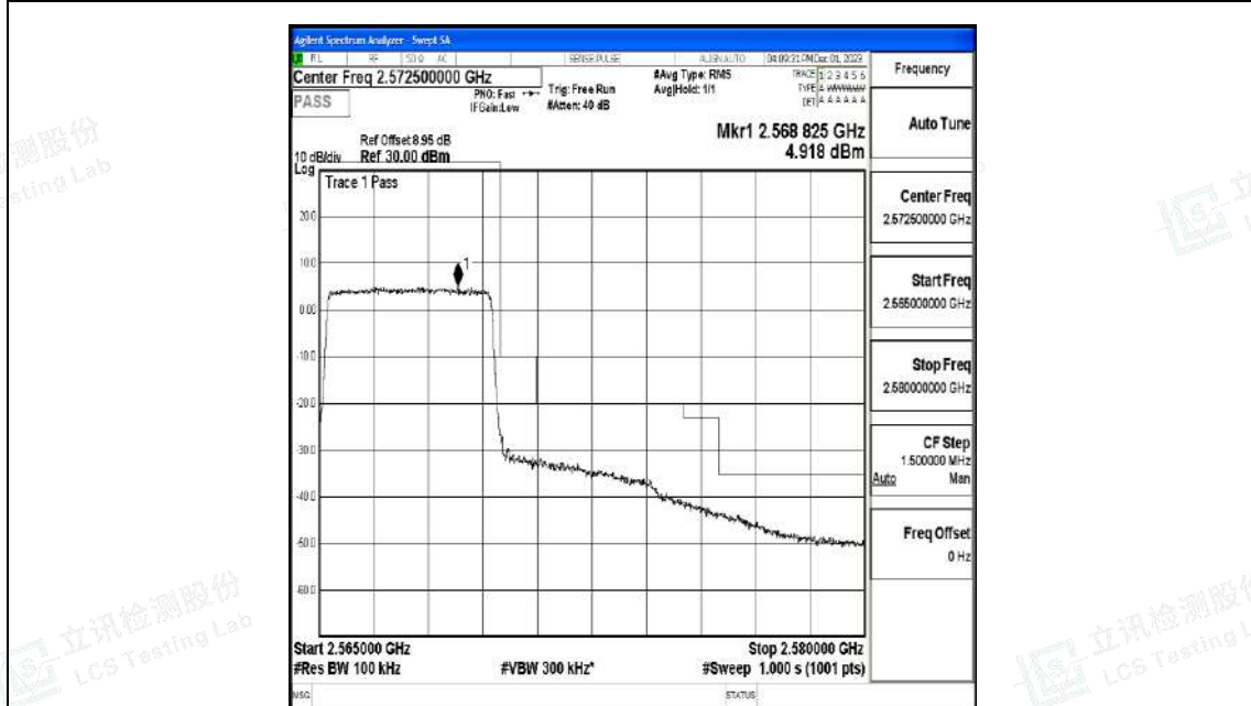
Band7_5MHz_16QAM_21425_25RB#0
