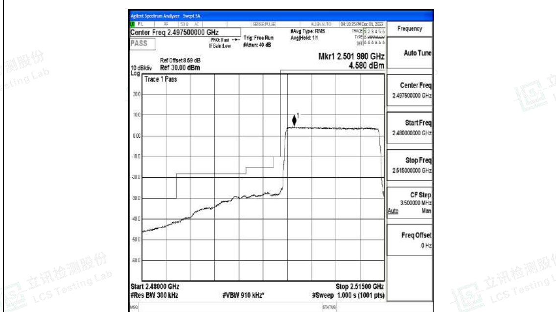
Band7_15MHz_16QAM_20825_75RB#0
