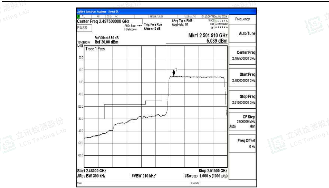
Band7_15MHz_QPSK_20825_75RB#0
