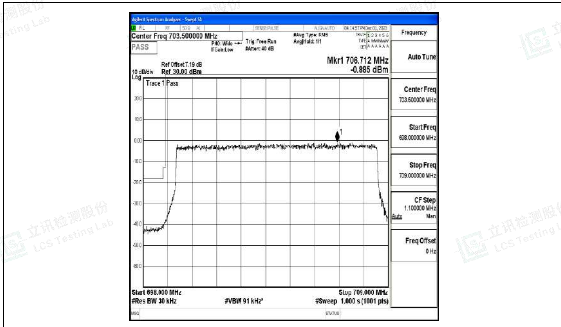
Band12_10MHz_16QAM_23060_50RB#0
