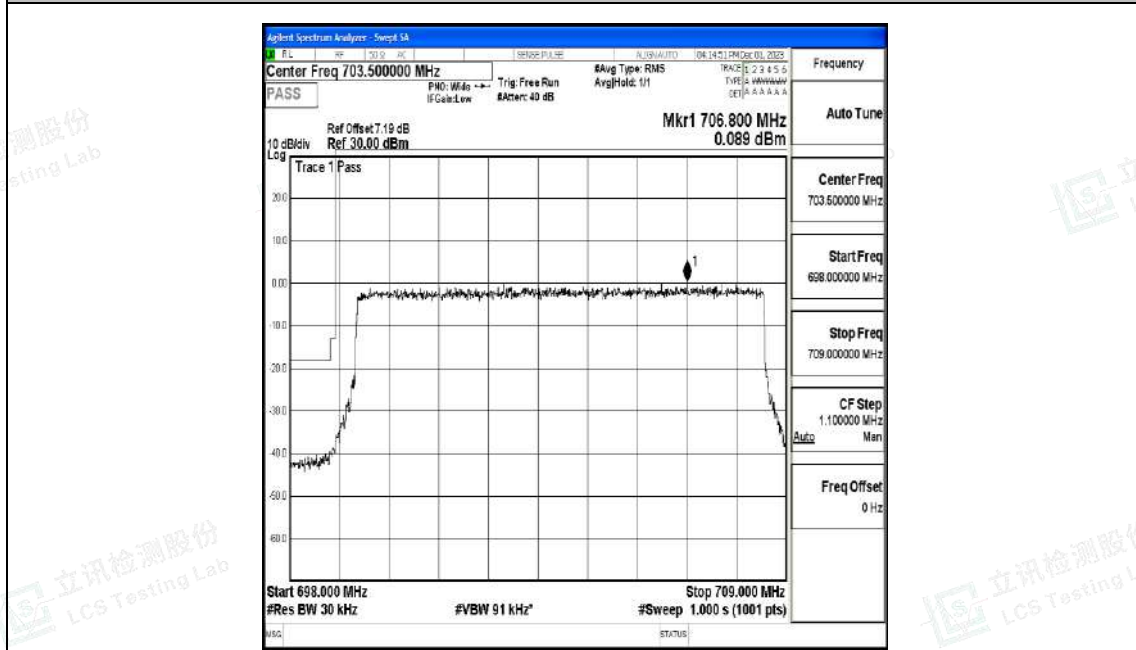
Band12_10MHz_QPSK_23060_50RB#0
