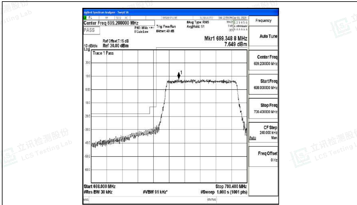
Band12_1.4MHz_16QAM_23017_6RB#0
