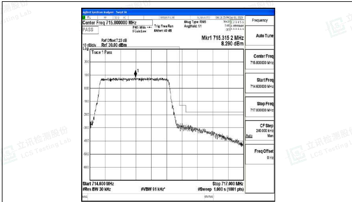
Band12_1.4MHz_16QAM_23173_6RB#0
