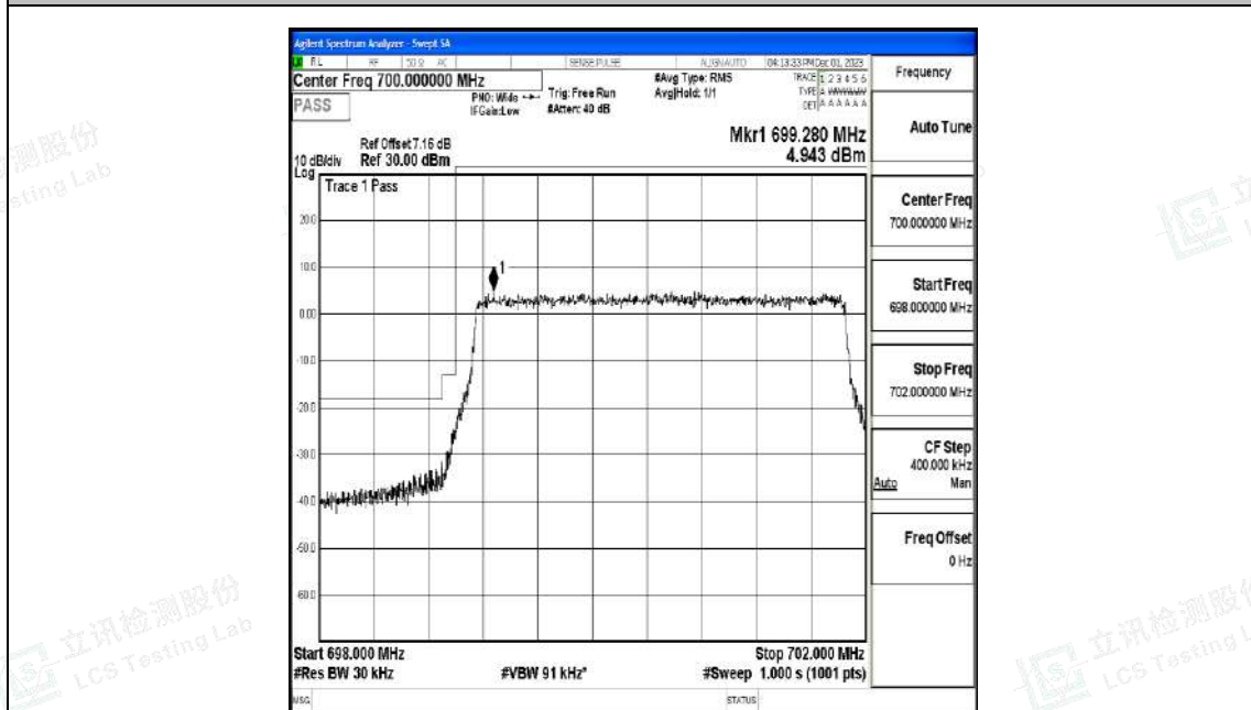
Band12_3MHz_QPSK_23025_15RB#0
