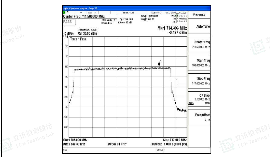
Band12_10MHz_QPSK_23130_50RB#0
