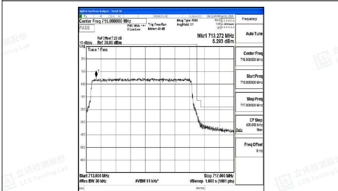
Band12_3MHz_QPSK_23165_15RB#0
