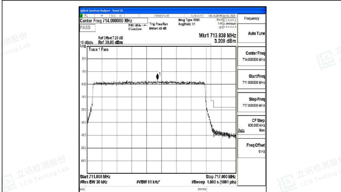
Band12_5MHz_QPSK_23155_25RB#0
