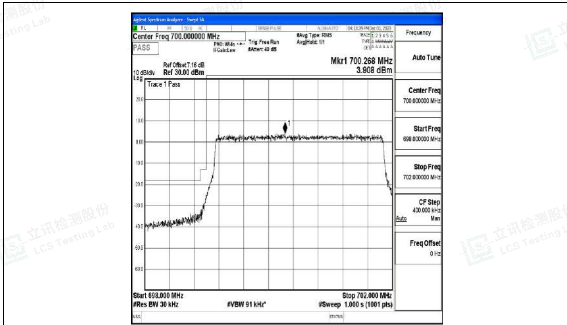
Band12_3MHz_16QAM_23025_15RB#0
