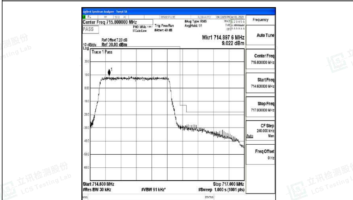
Band12_1.4MHz_QPSK_23173_6RB#0
