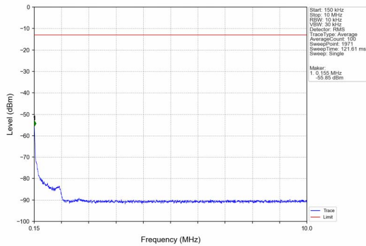
Band26a_1.4MHz_QPSK_MCH_819MHz_RB_1_0_NTNV
