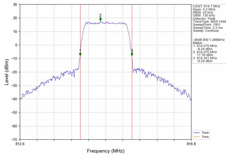
Band26a_1.4MHz_16QAM_LCH_814.7MHz_RB_6_0_NTNV
