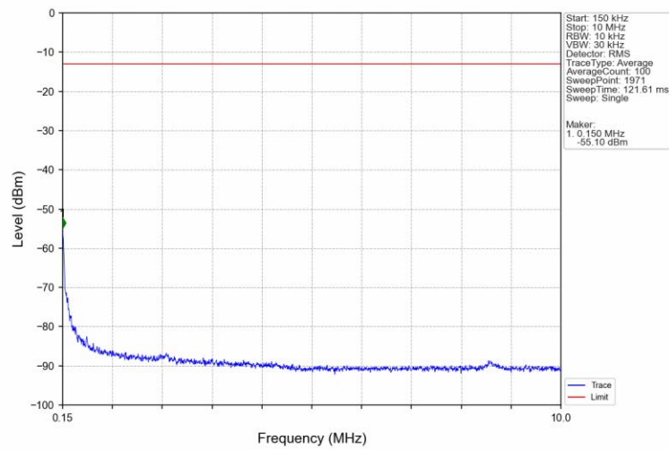
Band26a_5MHz_QPSK_HCH_821.5MHz_RB_1_0_NTNV
