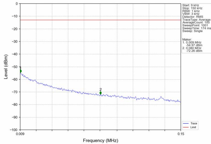
Band26a_3MHz_16QAM_HCH_822.5MHz_RB_1_0_NTNV
