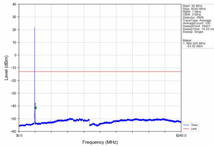
Band26a_3MHz_16QAM_MCH_819MHz_RB_1_0_NTNV
