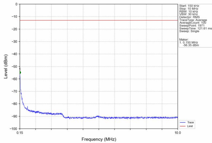
Band26a_3MHz_16QAM_HCH_822.5MHz_RB_1_0_NTNV
