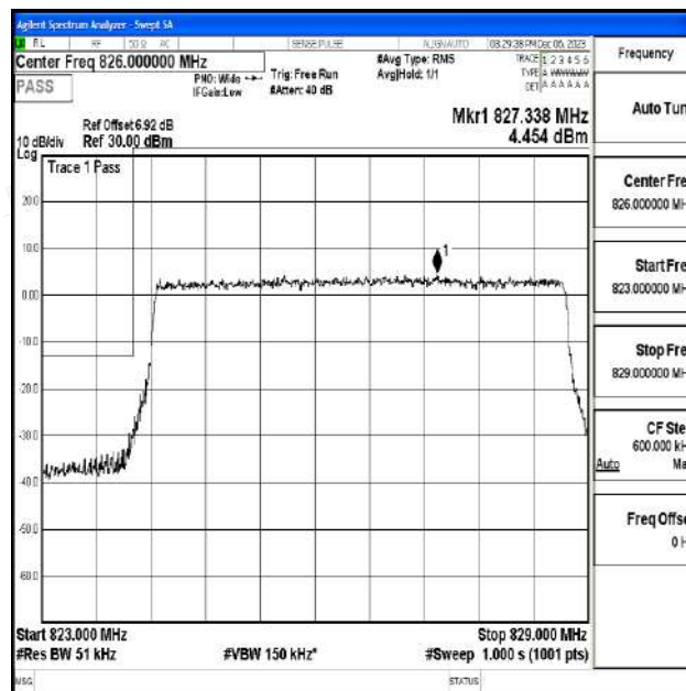
Band5_5MHz_QPSK_20425_25RB#0
