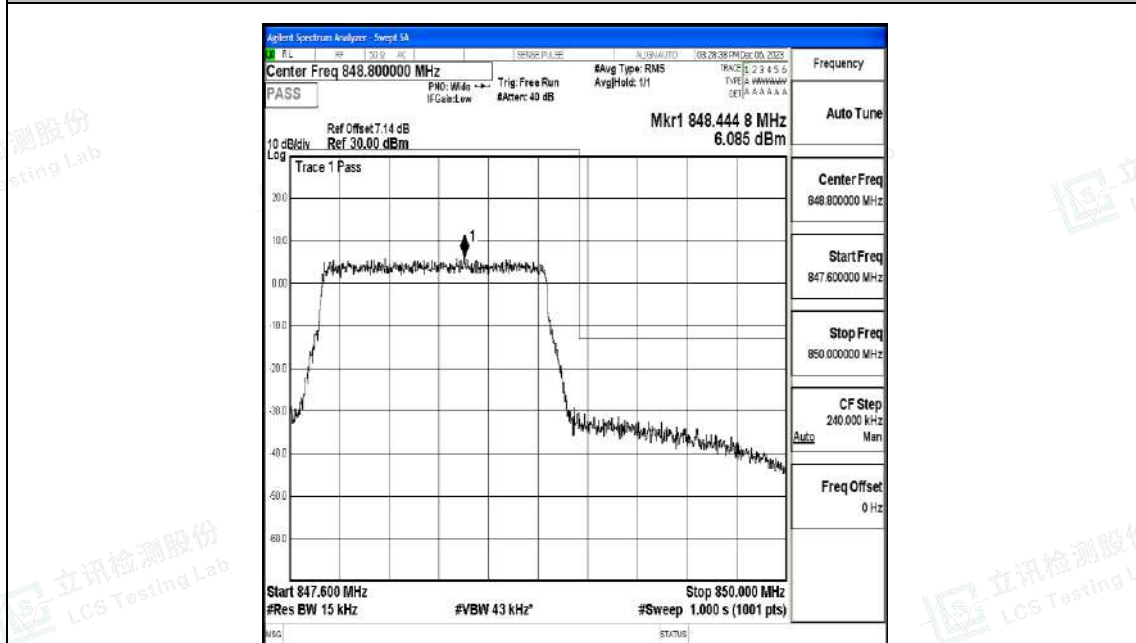
Band5_1.4MHz_QPSK_20643_6RB#0
