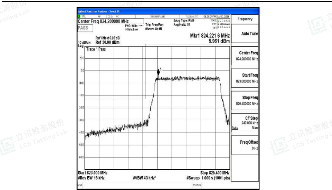
Band5_1.4MHz_16QAM_20407_6RB#0
