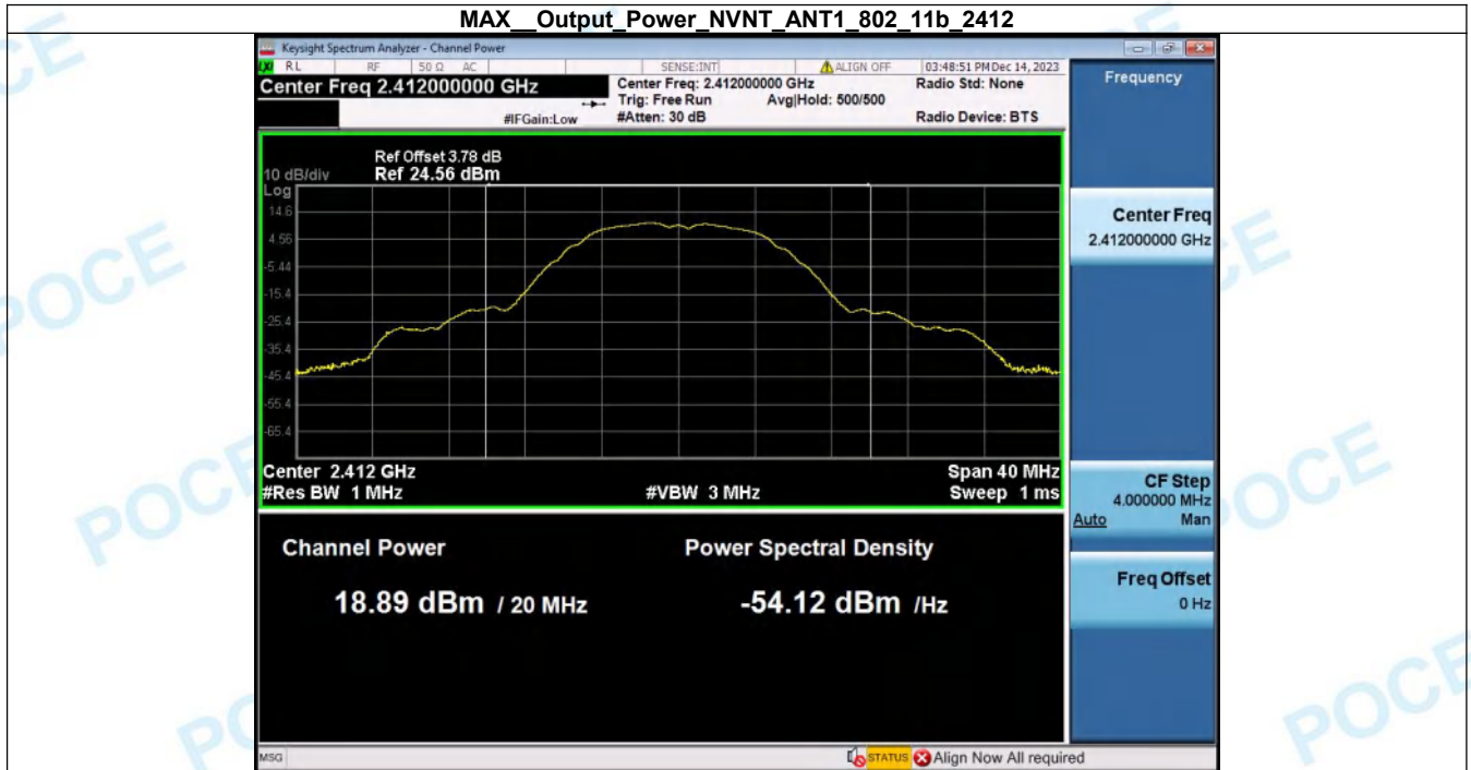
MAX Output Power_NVNT_ANT1_802_11b_2412
