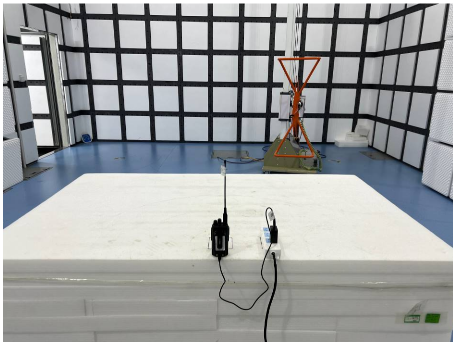
RE - Back View (Below 1GHz) -Mode 1
