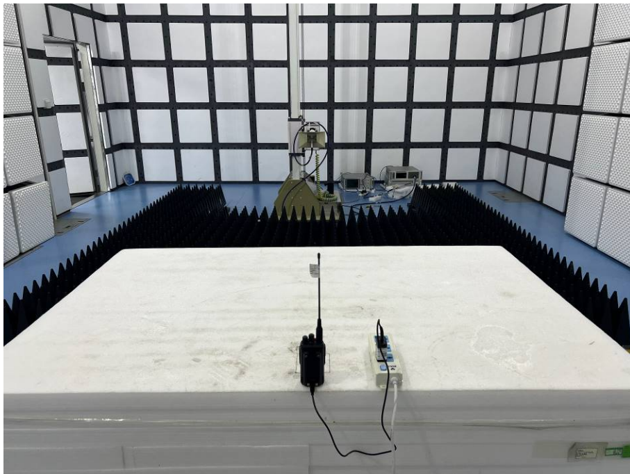
RE - Back View (Above 1GHz) -Mode 1
