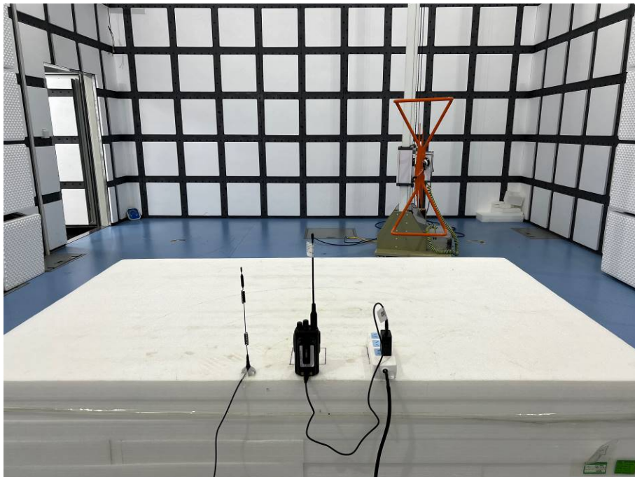
RE - Back View (Below 1GHz) -Mode 2
