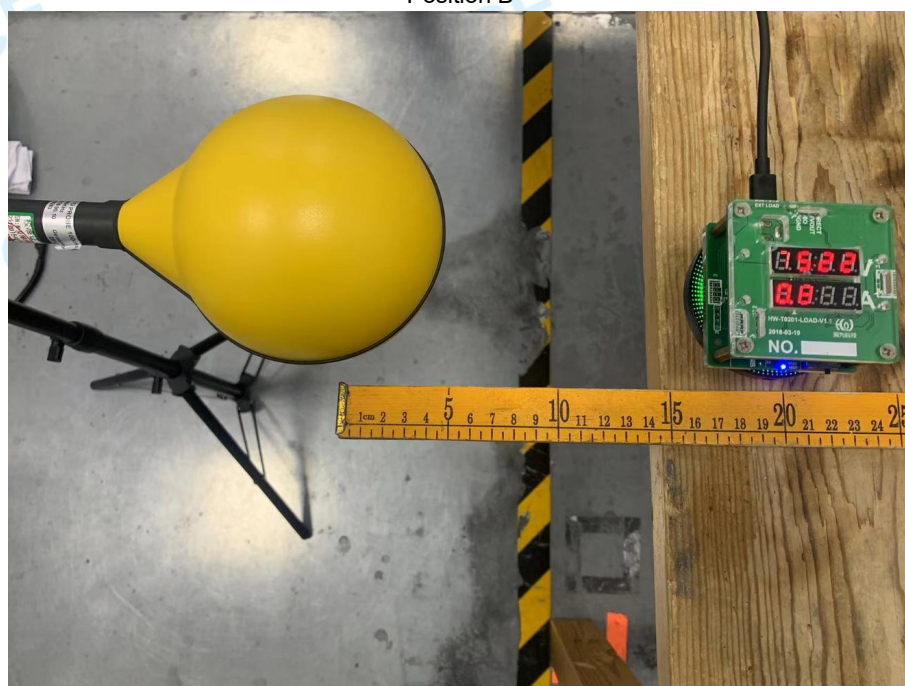
Position B
