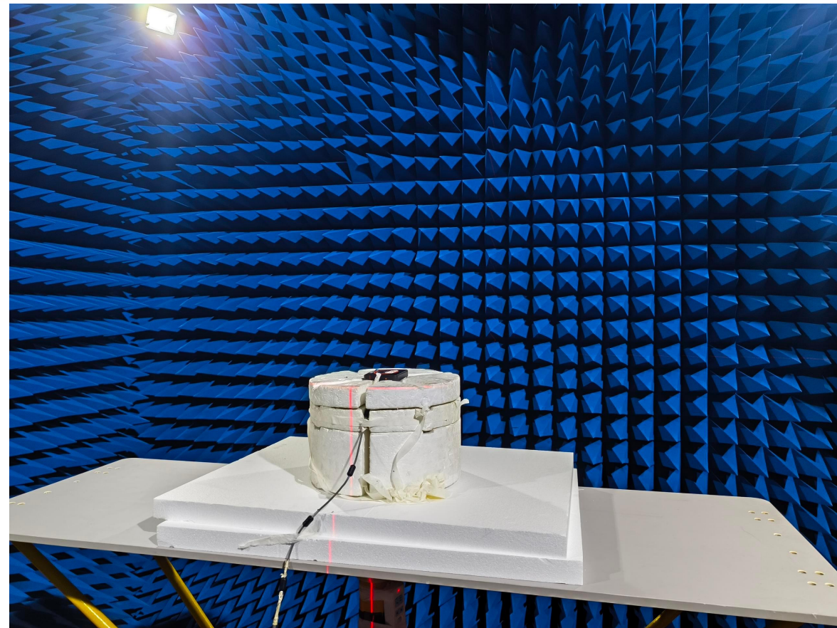
Testing 3D microwave darkroom(6m*6m*6m)
