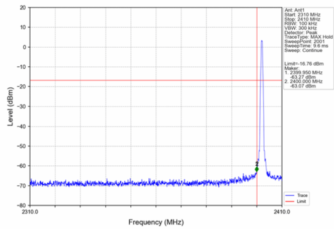
GFSK_DH5_LCH_2402MHz_Ant1_NTNV
