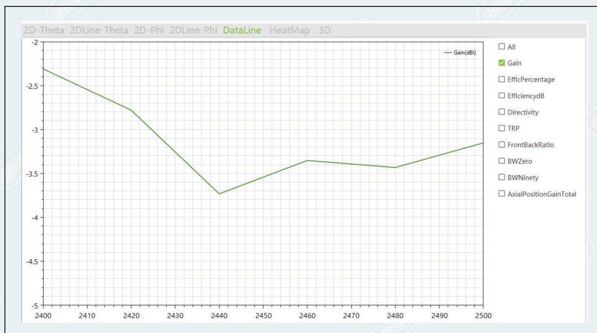
Gain plot
