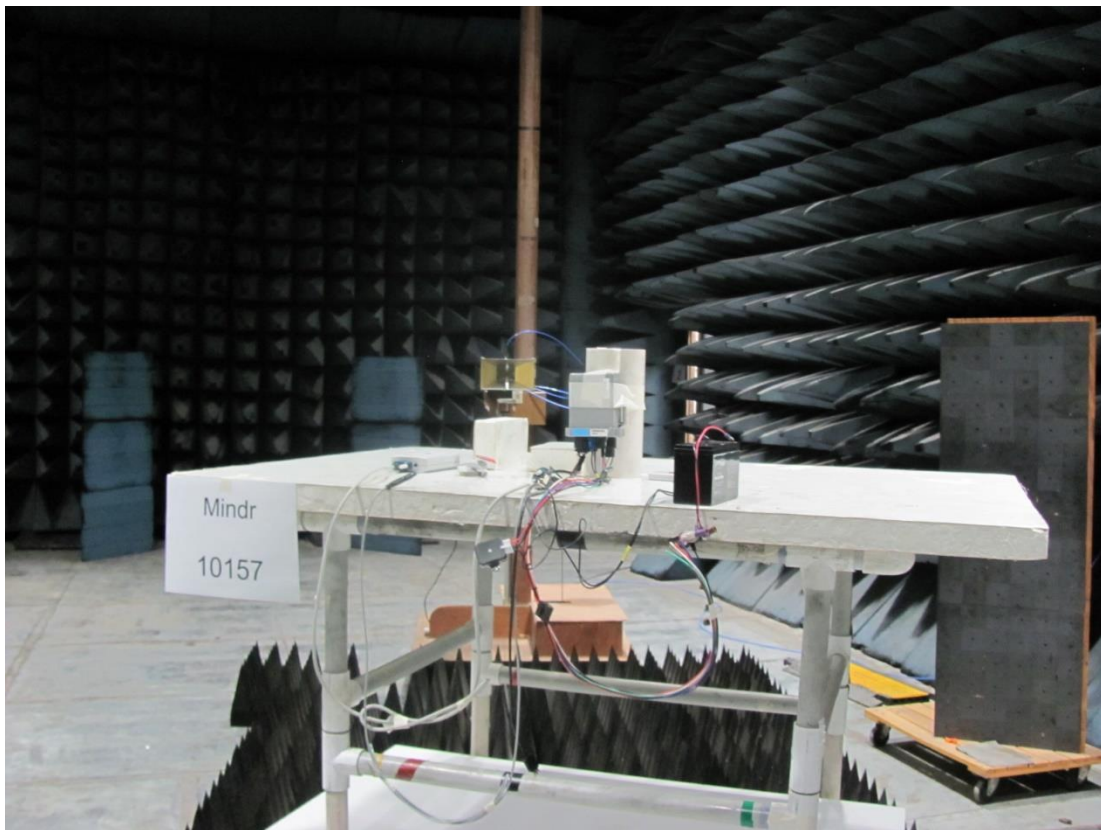
The EUT was taped to a non-conductive stand to change the axis of rotation.
