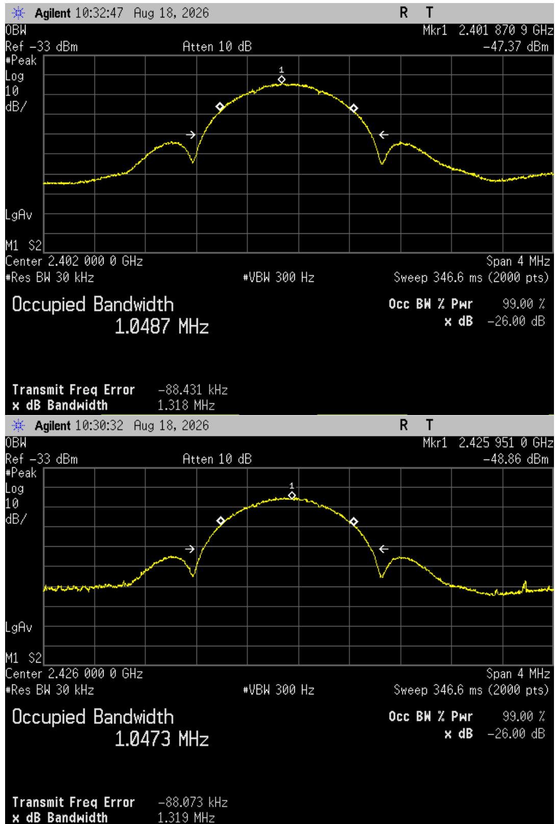
Figure 2. Occupied Bandwidth Plot
