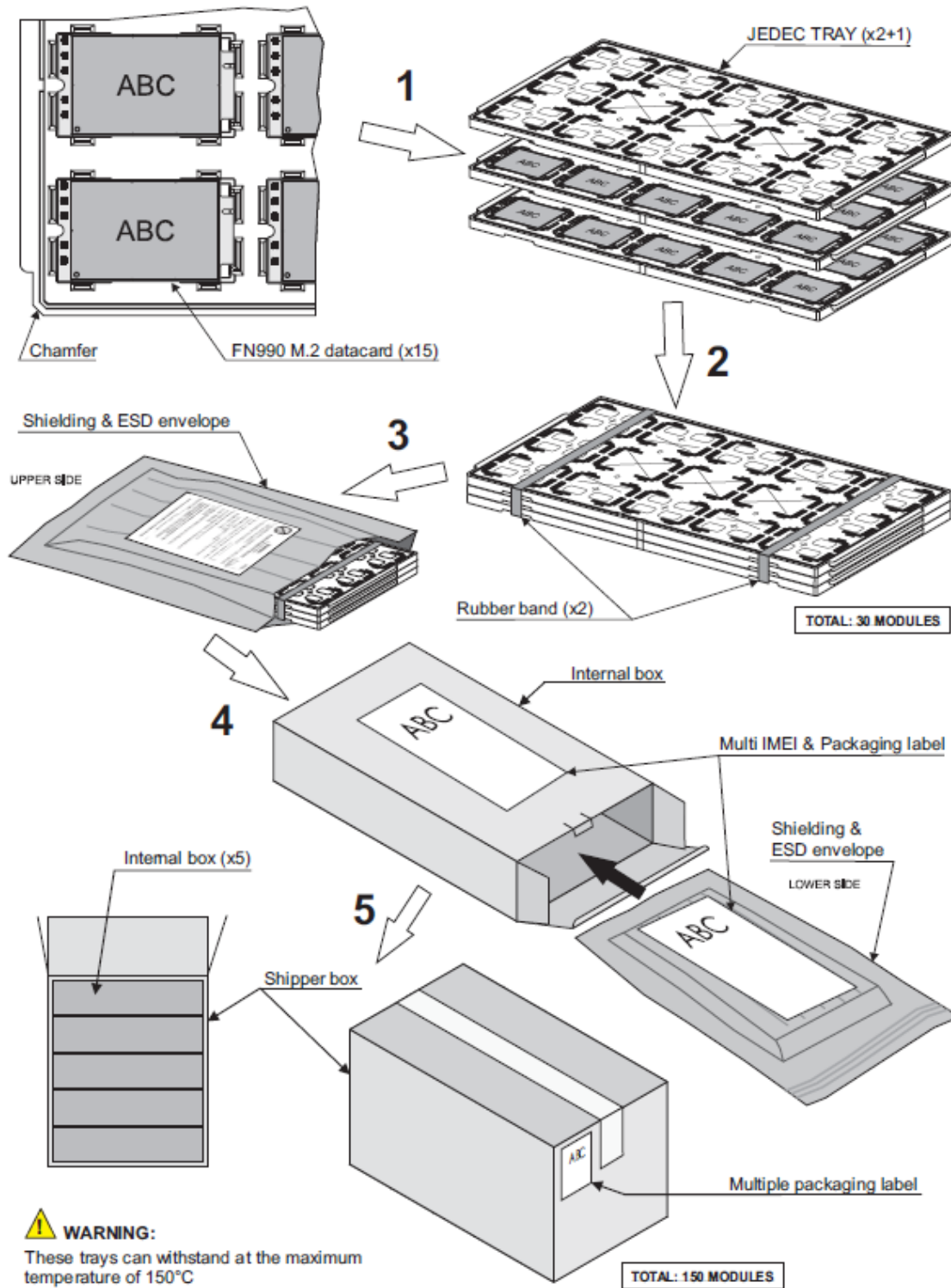
Figure 24: Tray Packaging
