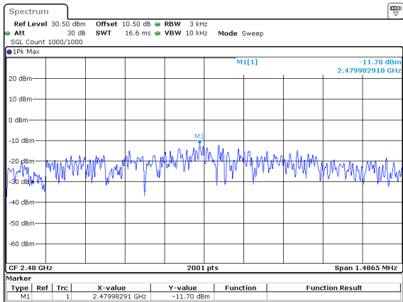
BLE_2M_High_Channel
