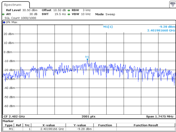
BLE_2M_Low_Channel
