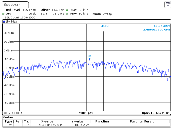
BLE_1M_High_Channel
