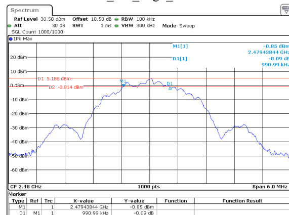
BLE_2M_High_Channel
