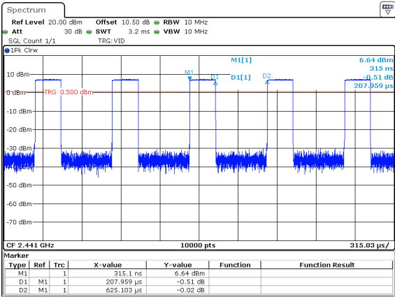
BLE_2M_Middle_Channel
