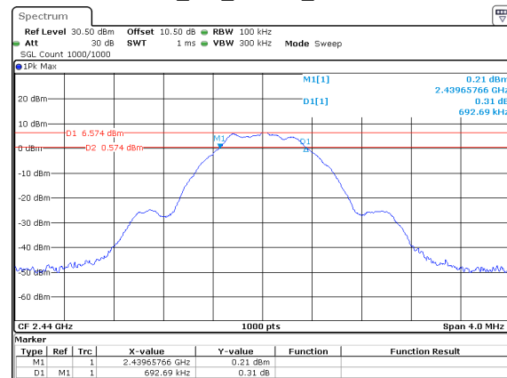
BLE_1M_Middle_Channel
