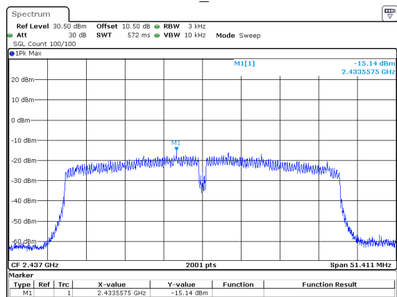
802.11n40_2437MHz
