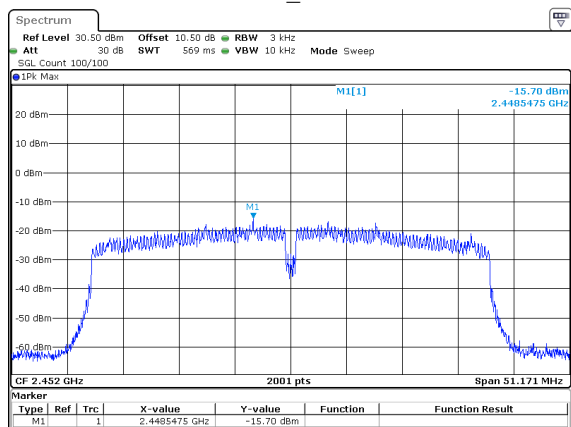
802.11n40_2452MHz
