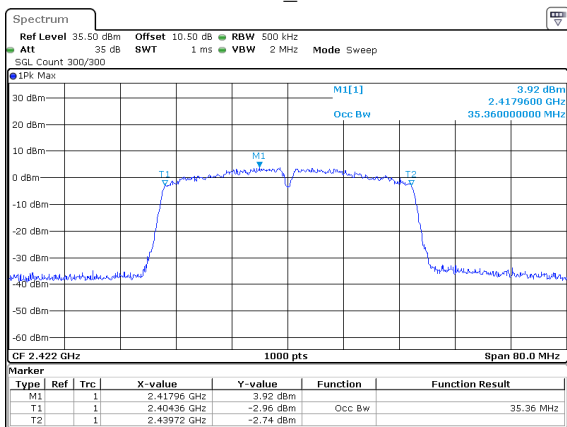
802.11n40_2422MHz
