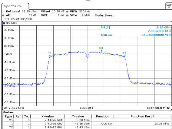
802.11n40_2437MHz
