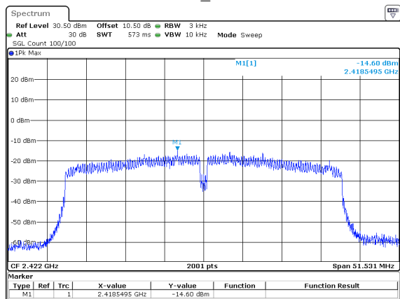
802.11n40_2422MHz
