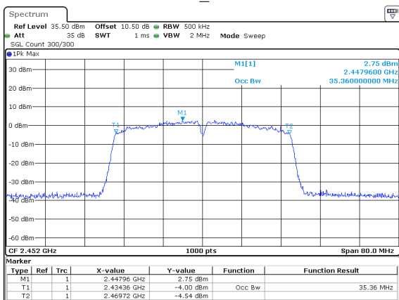
802.11n40_2452MHz
