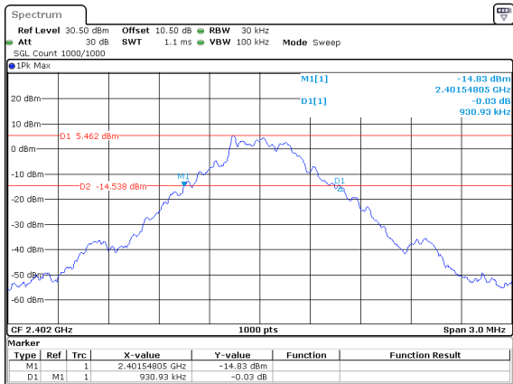
DH1_Low 0.931MHz
