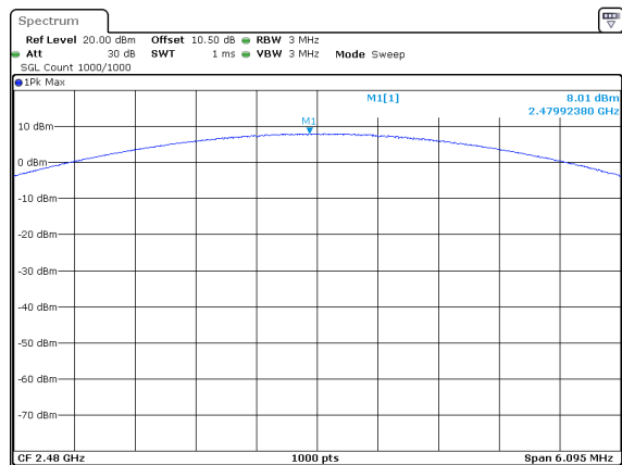
3DH1_High 8.01dBm
