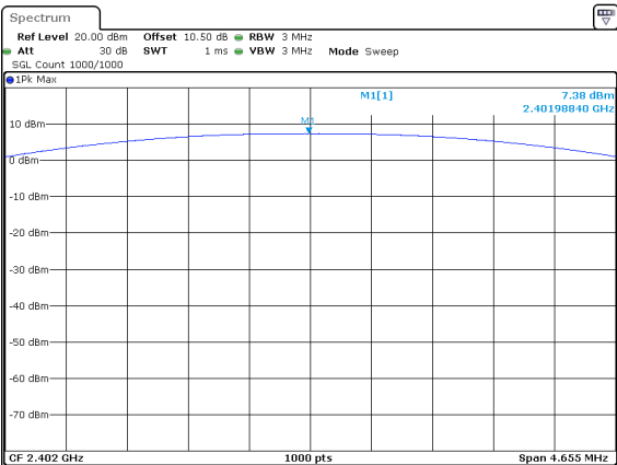
DH1_Low 7.38dBm
