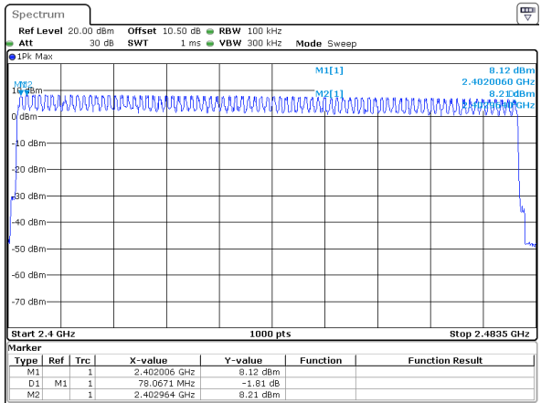
2DH1_Hopping 79
