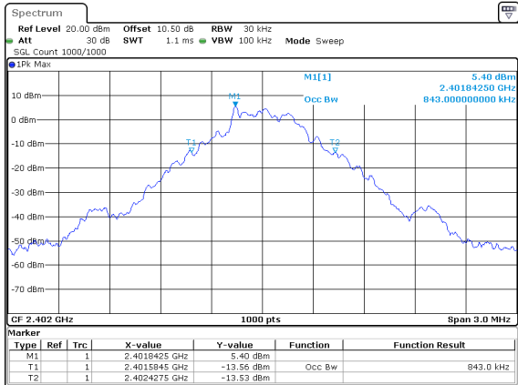
DH1_Low 0.843MHz
