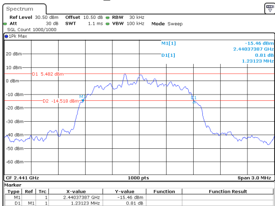
2DH1_Middle 1.231MHz
