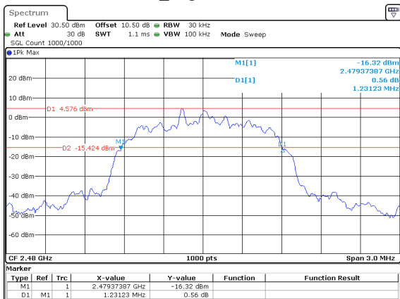
2DH1_High 1.231MHz
