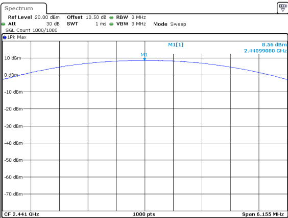
2DH1_Middle 8.56dBm
