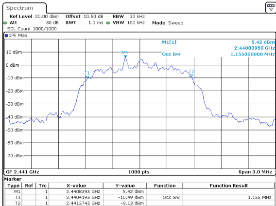
2DH1_Middle 1.155MHz
