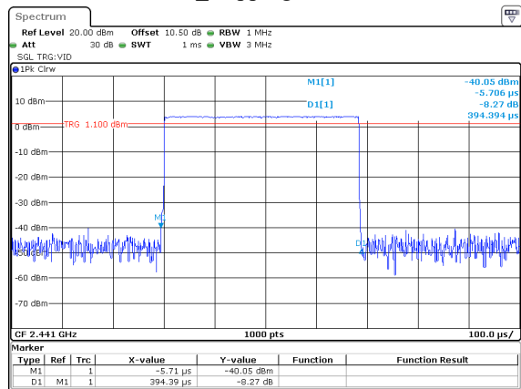
DH1_Hopping 0.394ms
