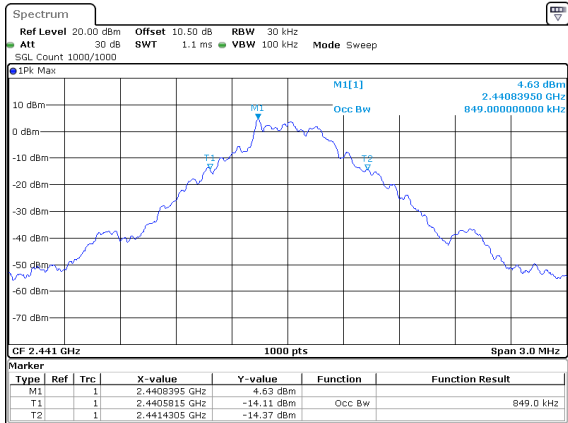
DH1_Middle 0.849MHz
