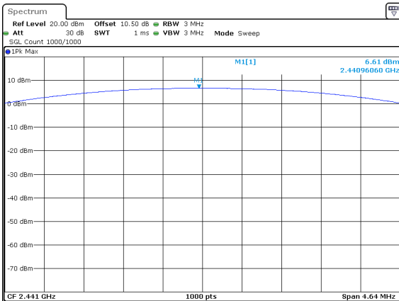
DH1_Middle 6.61dBm
