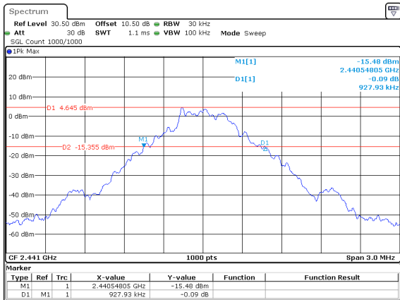
DH1_Middle 0.928MHz
