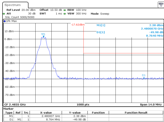
DH1_High
