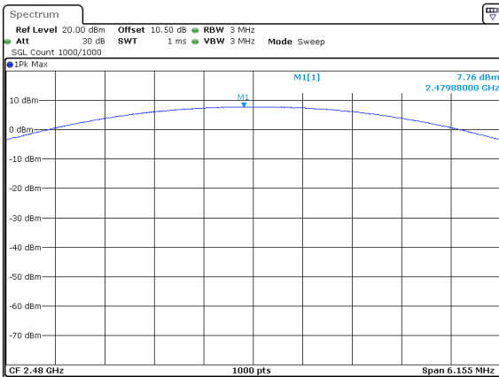
2DH1_High 7.76dBm
