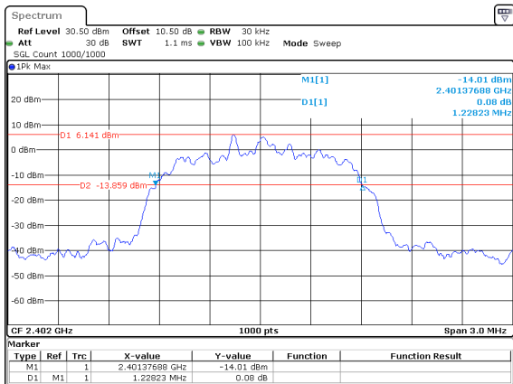
2DH1_Low 1.228MHz
