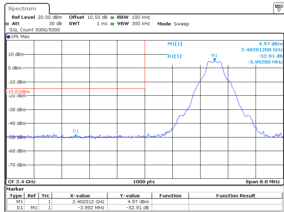
DH1_Low
