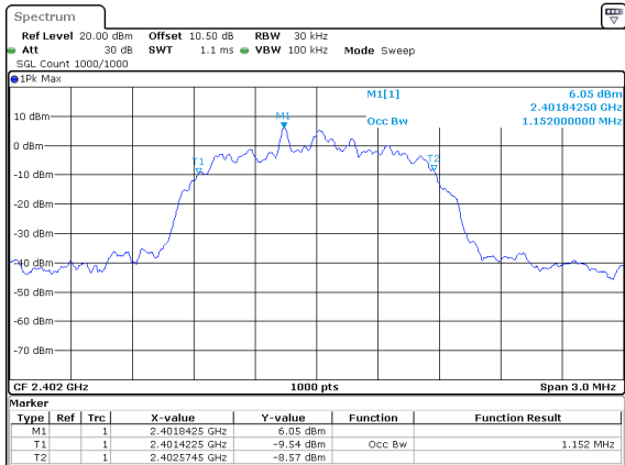
2DH1_Low 1.152MHz
