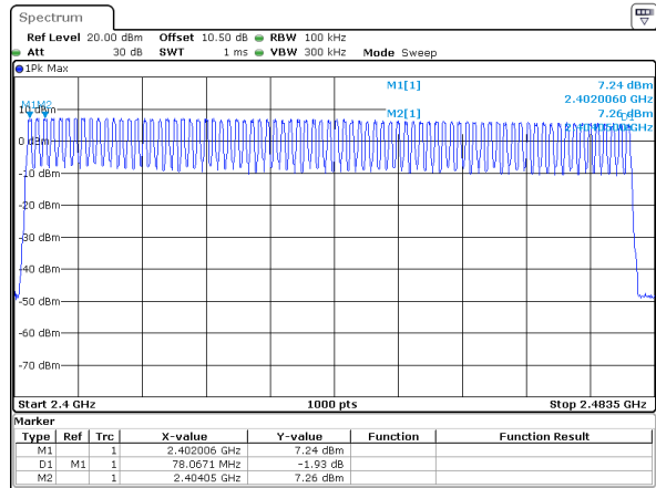
DH1_Hopping 79
