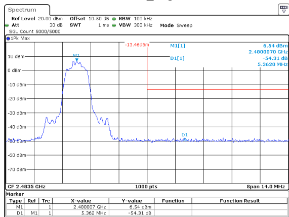
2DH1_High
