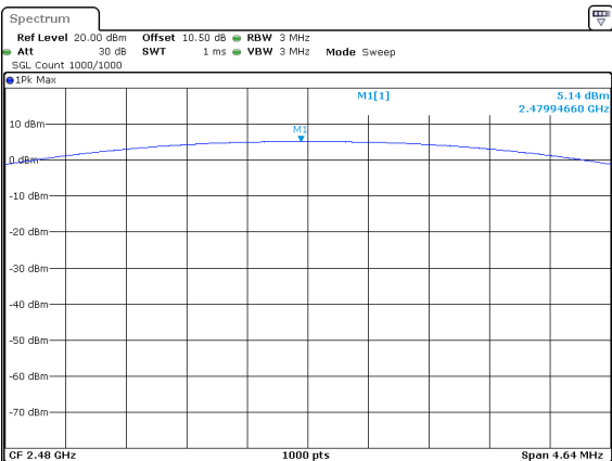
DH1_High 5.14dBm
