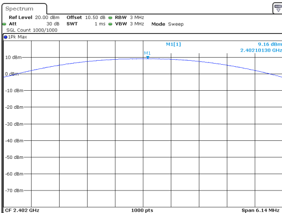
2DH1_Low 9.16dBm
