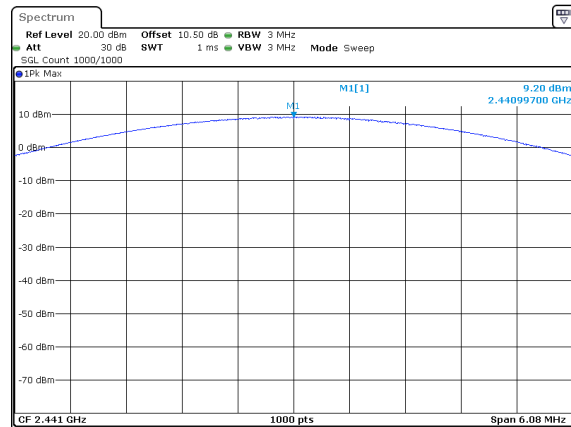
3DH1_Middle 9.20dBm
