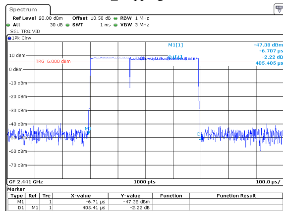
2DH1_Hopping 0.405ms
