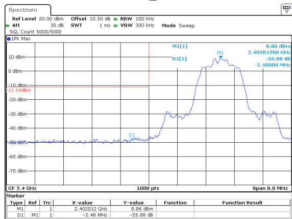
2DH1_Low
