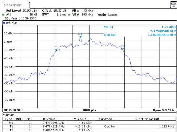
2DH1_High 1.152MHz
