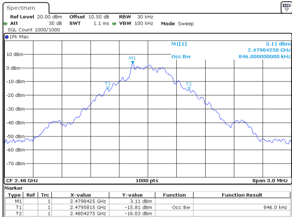
DH1_High 0.846MHz
