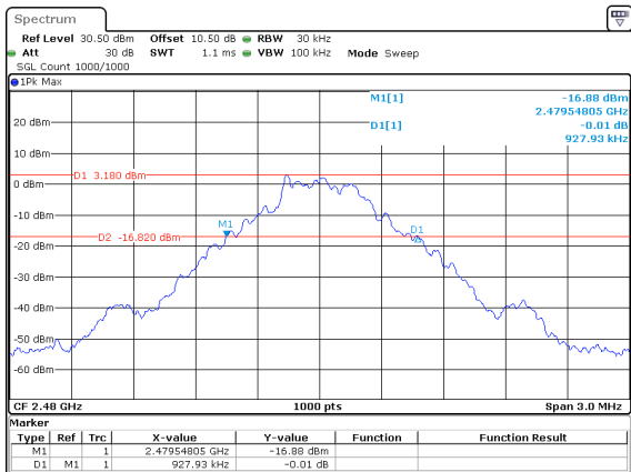
DH1_High 0.928MHz
