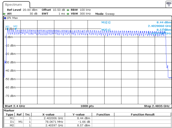
3DH1_Hopping 79
