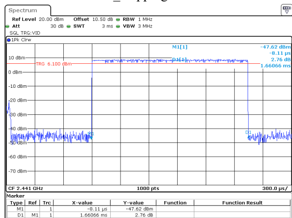
2DH3_Hopping 1.661ms
