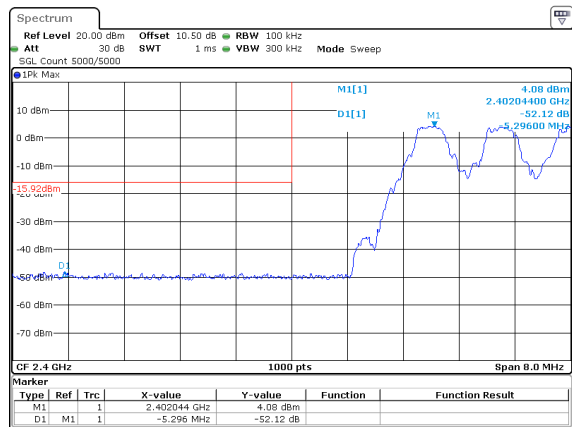
DH1_Hopping_Lower
