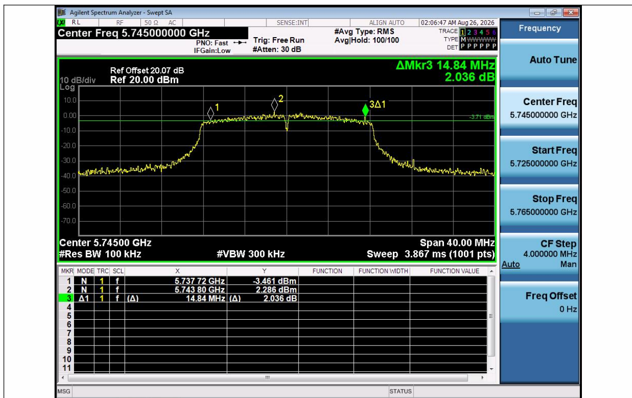
11A-Ant1-5745-PASS
