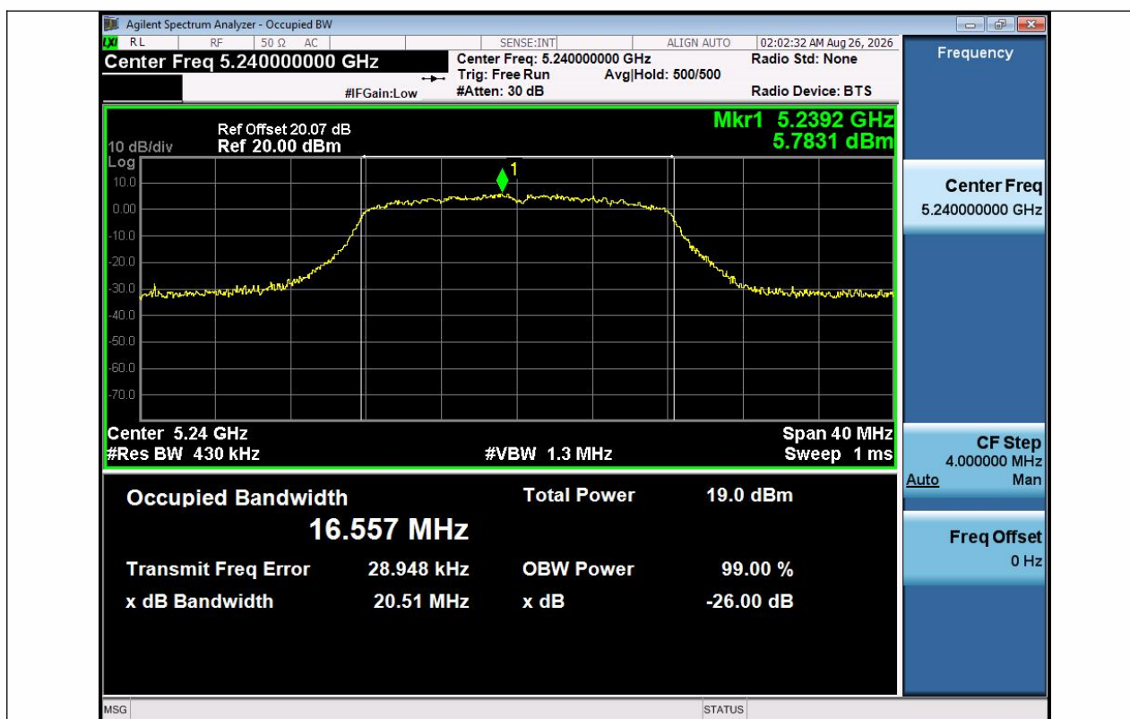
11A-Ant1-5240
