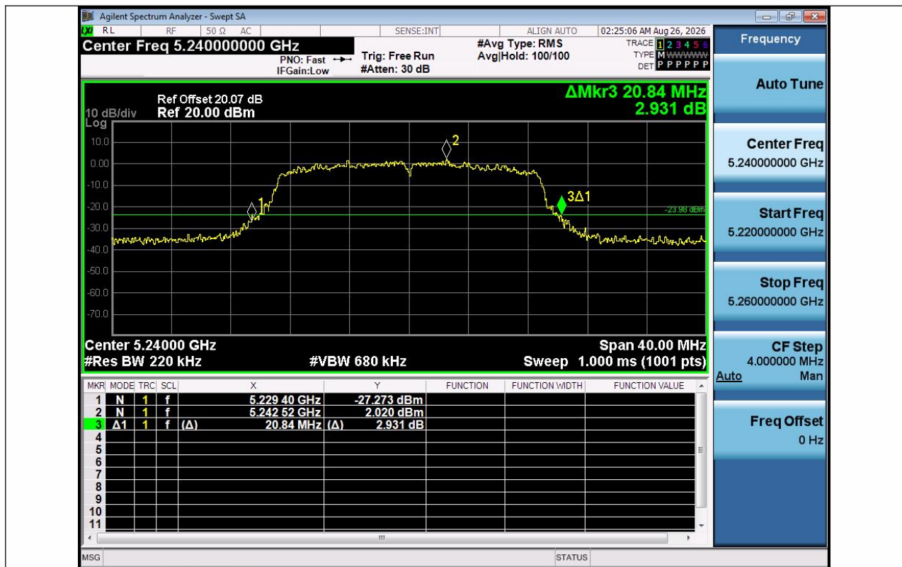
11N20SISO-Ant1-5240
