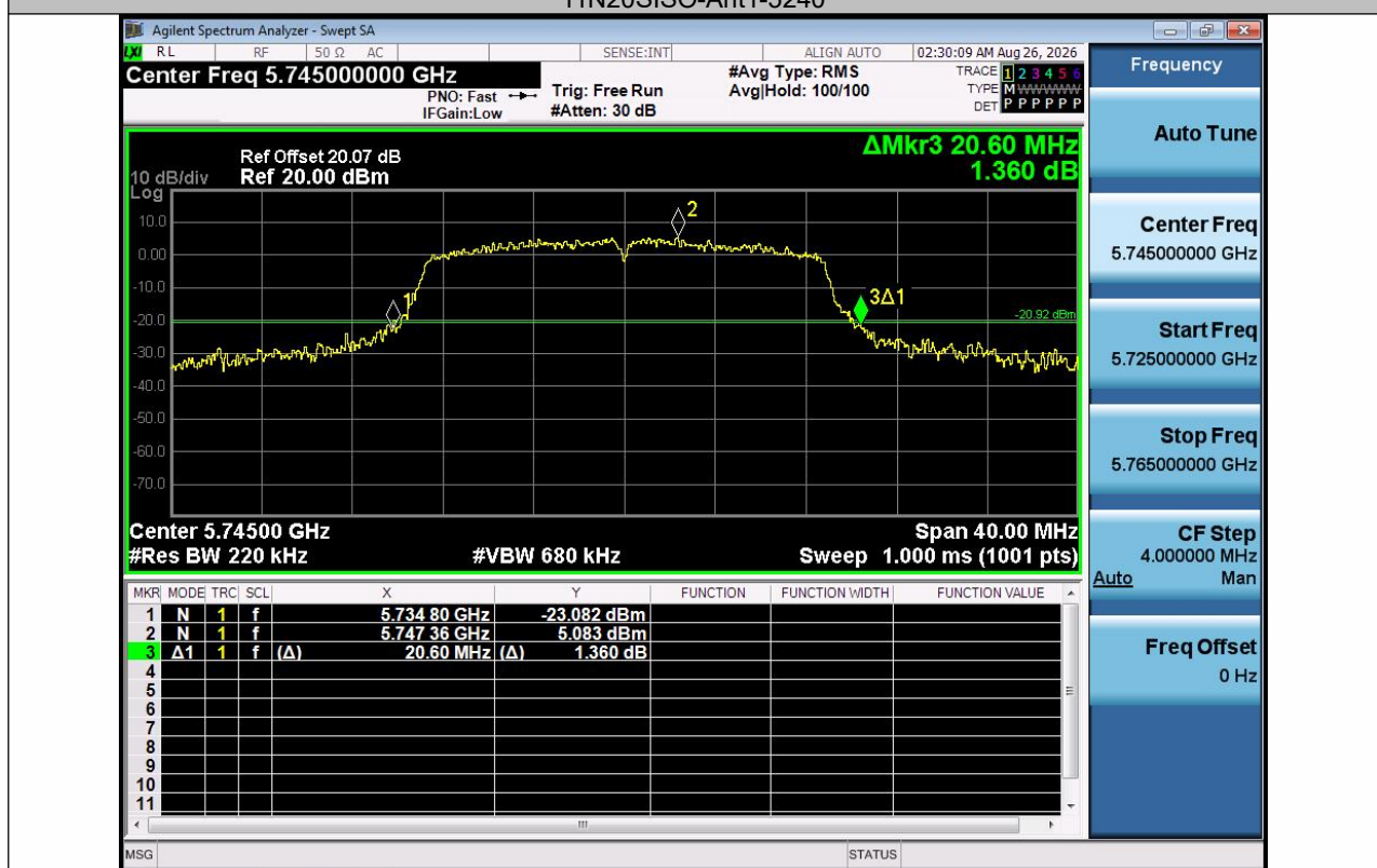
11N20SISO-Ant1-5745
