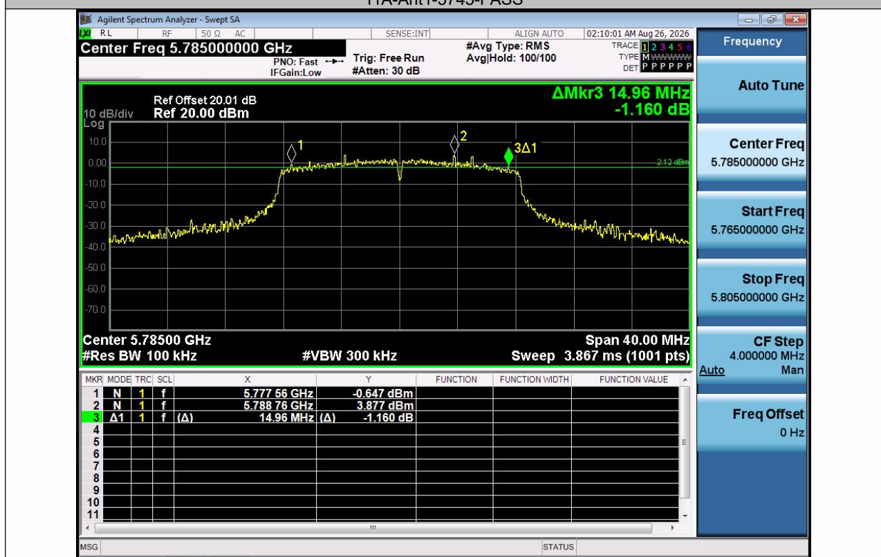
11A-Ant1-5785-PASS
