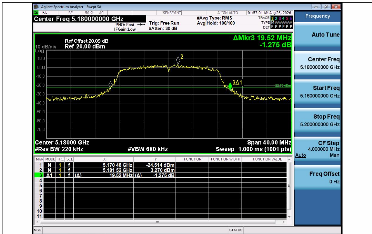
11A-Ant1-5180
