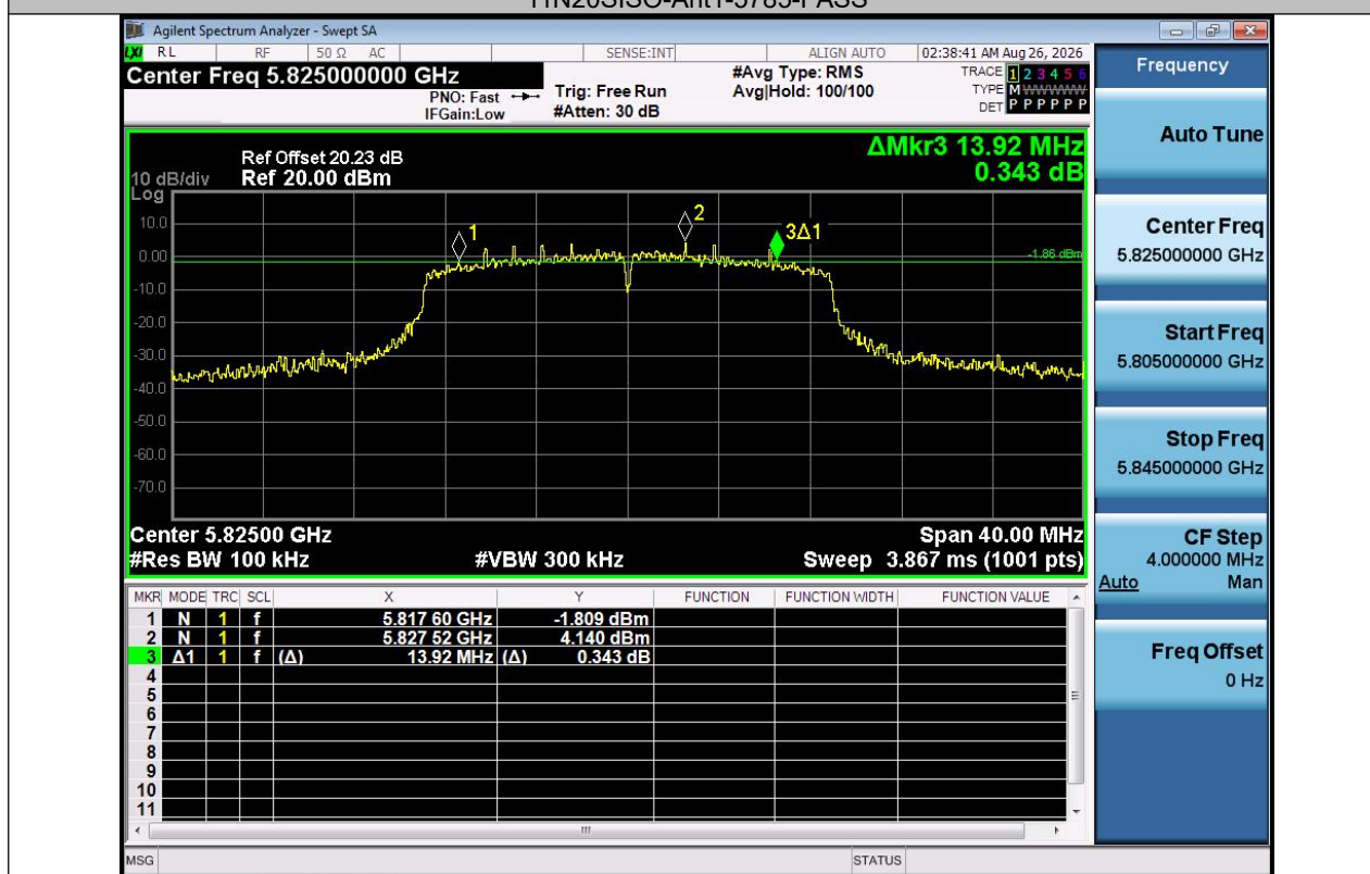
11N20SISO-Ant1-5825-PASS
