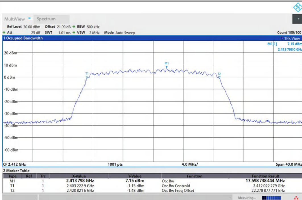
11N20MIMO-Ant2-2412
