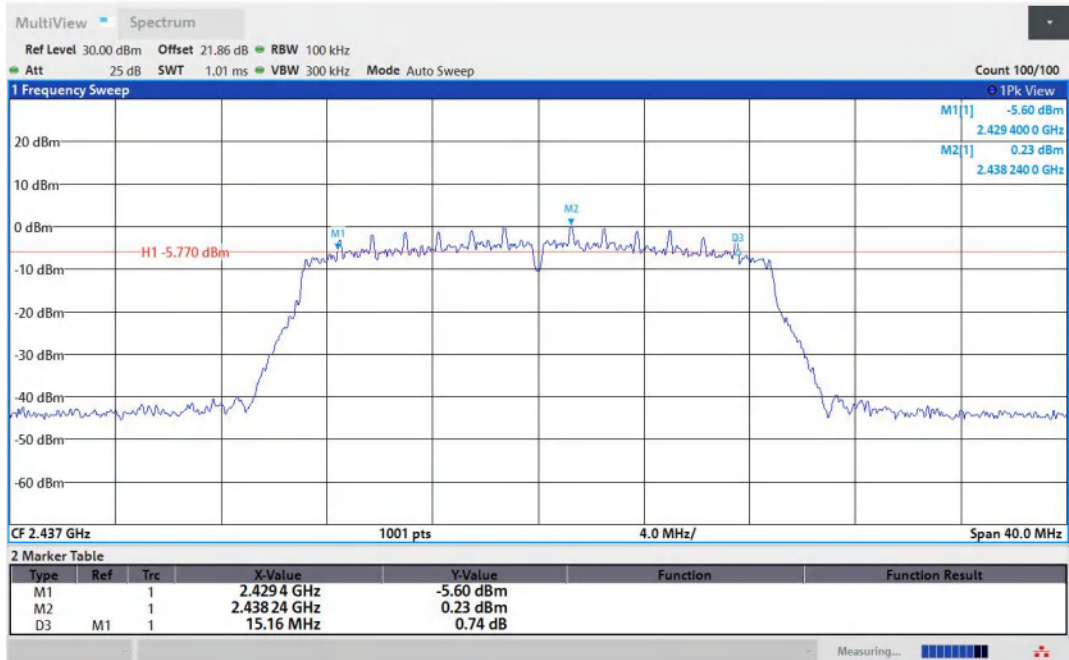
11N20MIMO-Ant1-2437-PASS
