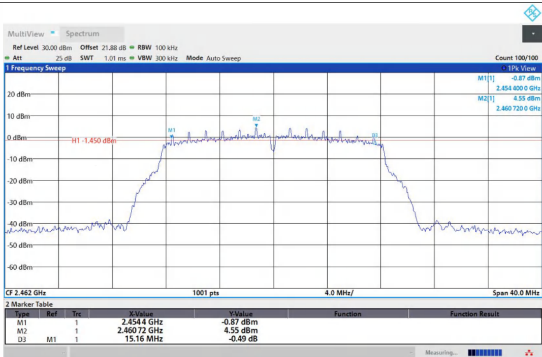
11G-Ant1-2462-PASS
