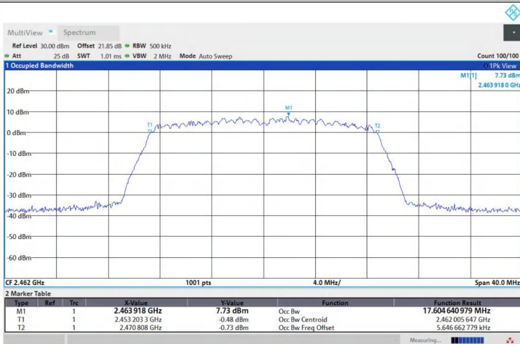
11N20MIMO-Ant2-2462
