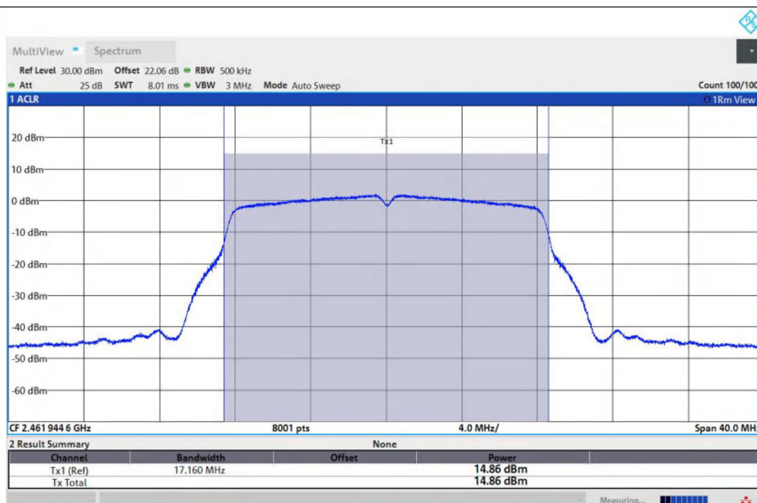
11G-Ant1-2462-PASS
