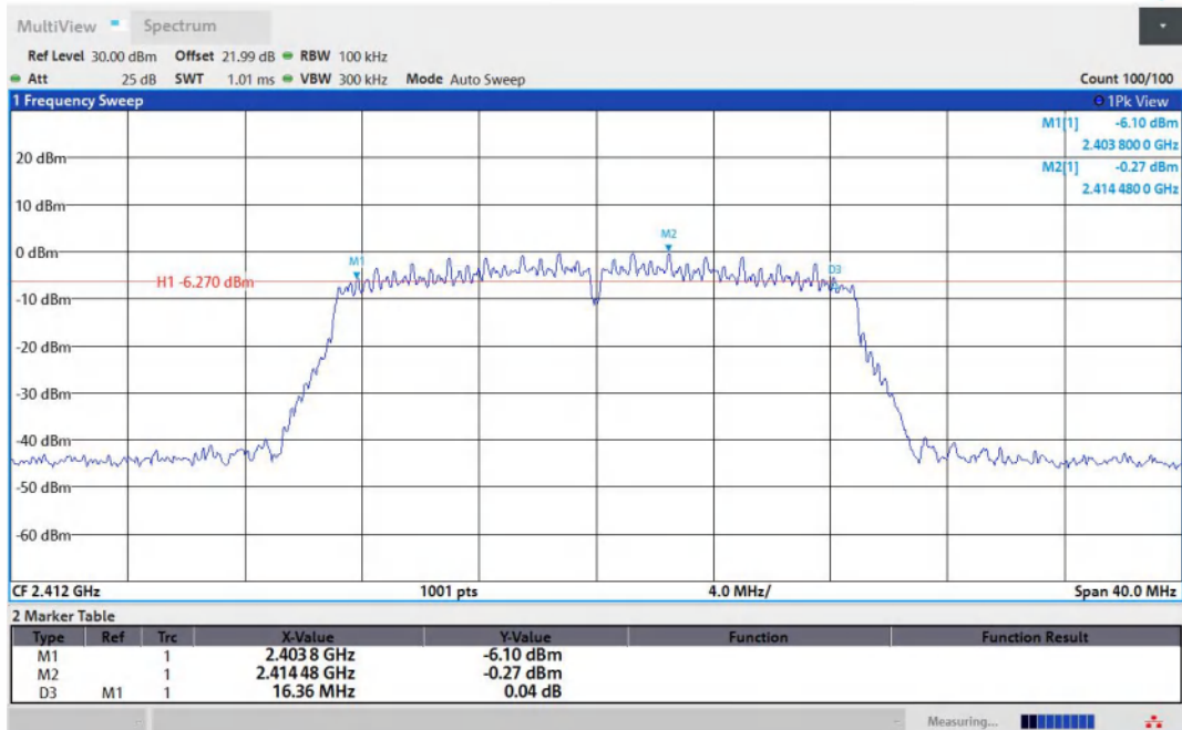
11N20MIMO-Ant2-2412-PASS
