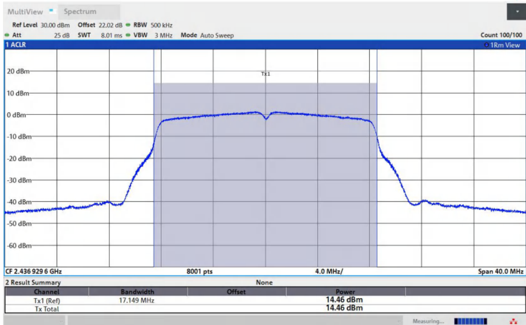
11G-Ant2-2437-PASS
