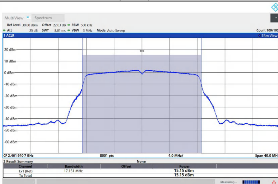
11G-Ant2-2462-PASS
