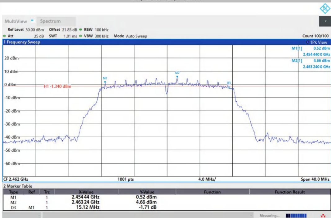
11G-Ant2-2462-PASS
