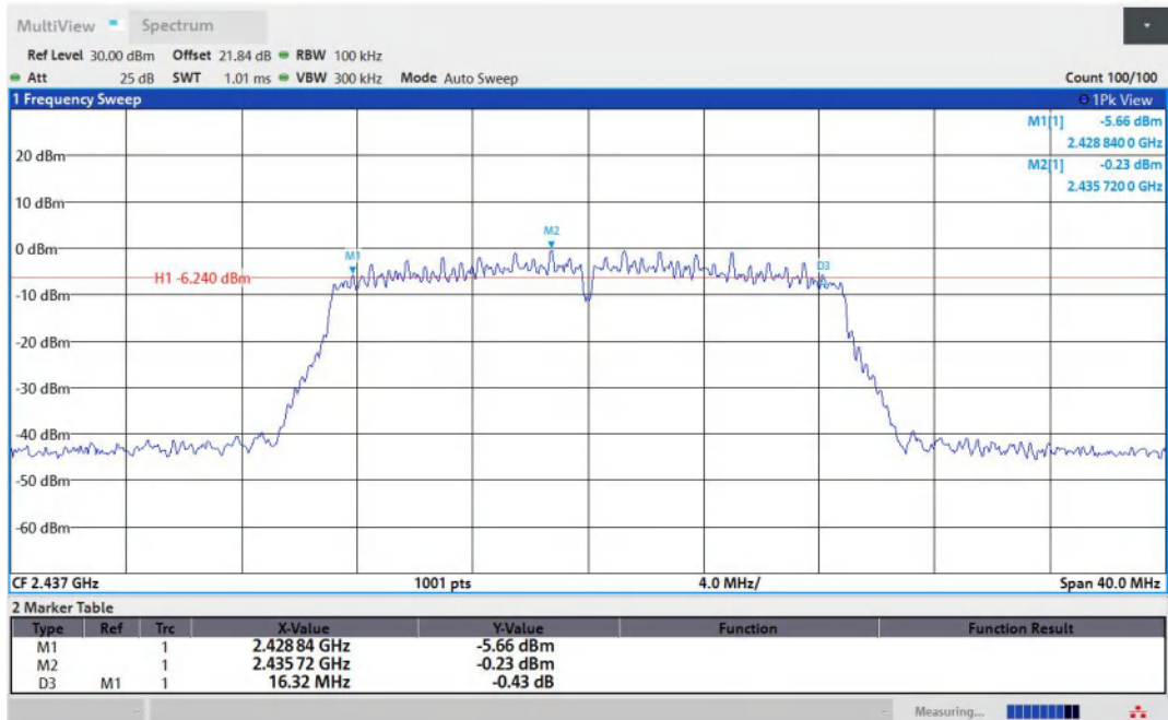
11N20MIMO-Ant2-2437-PASS
