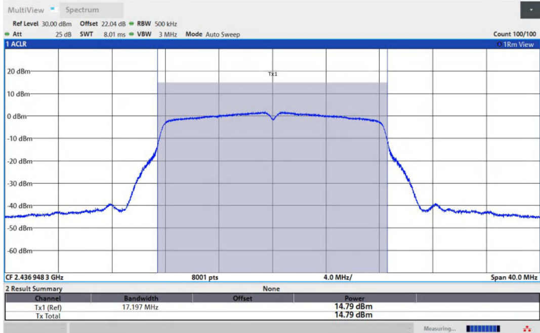
11G-Ant1-2437-PASS
