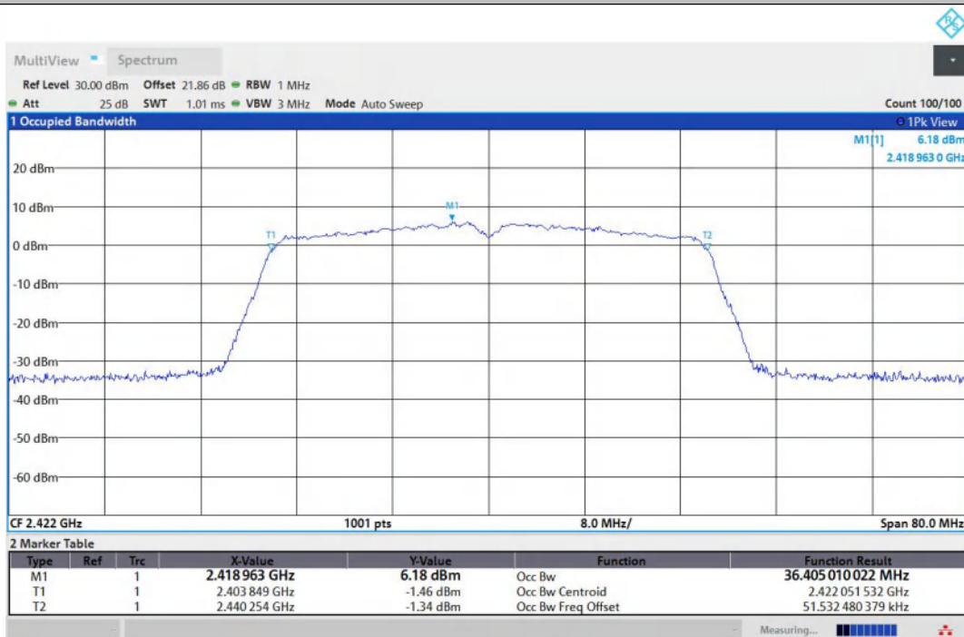
11N40MIMO-Ant2-2422
