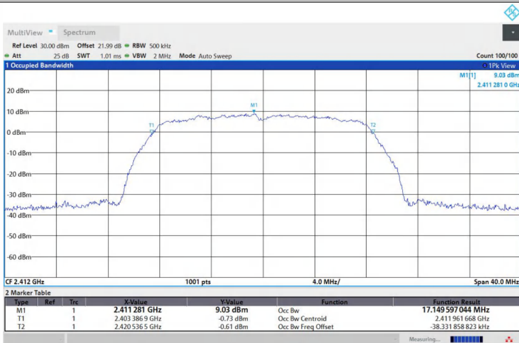
11G-Ant2-2412
