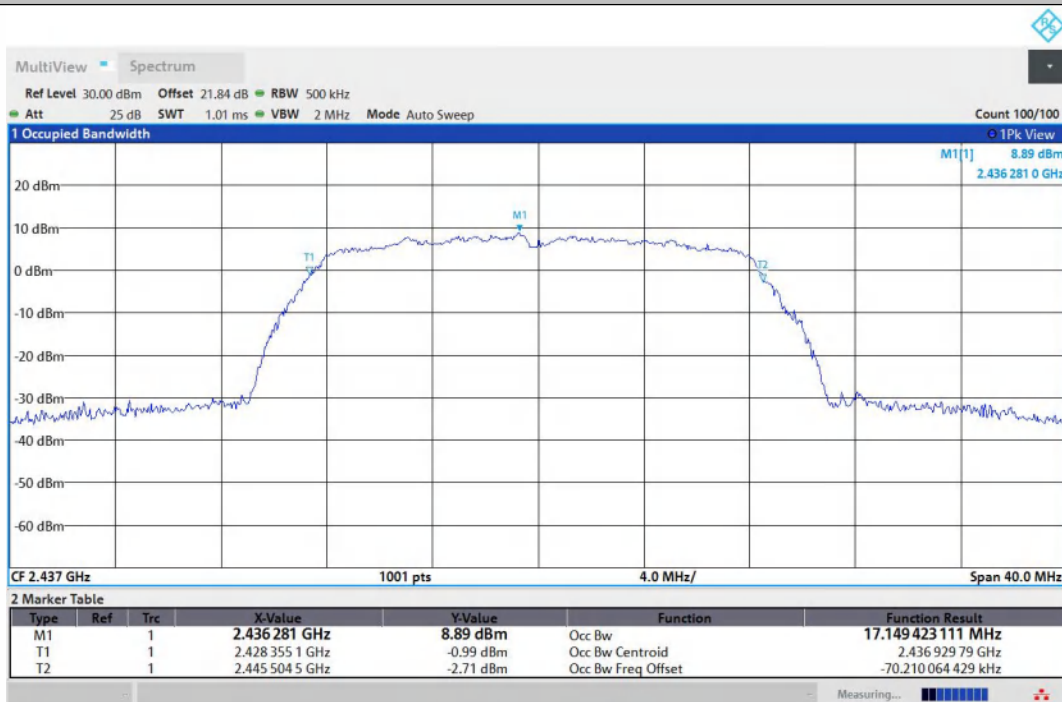
11G-Ant2-2437
