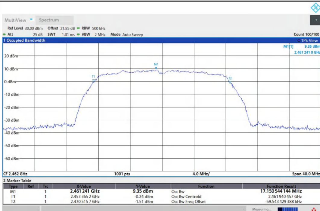
11G-Ant2-2462
