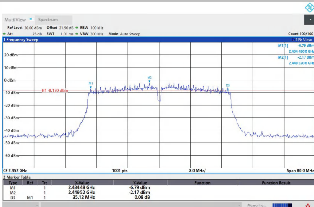
11N40MIMO-Ant2-2452-PASS
