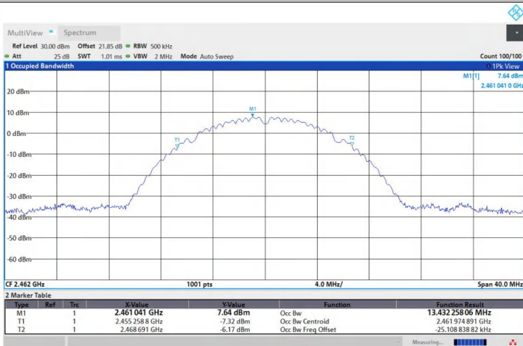
11B-Ant2-2462
