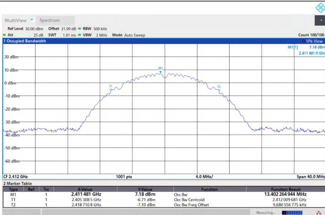
11B-Ant2-2412
