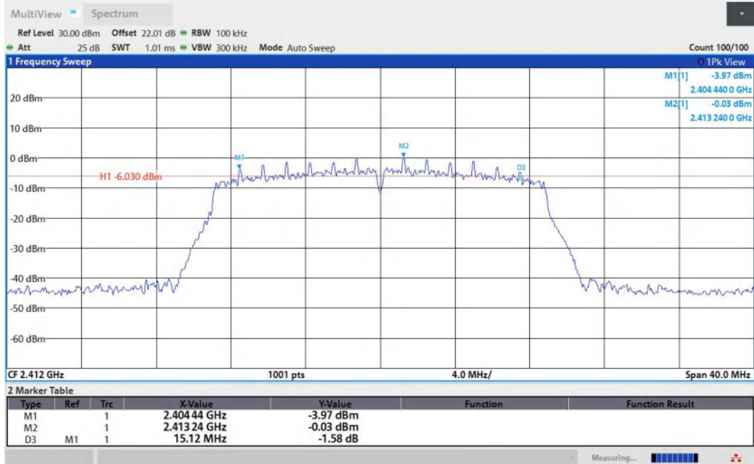
11N20MIMO-Ant1-2412-PASS
