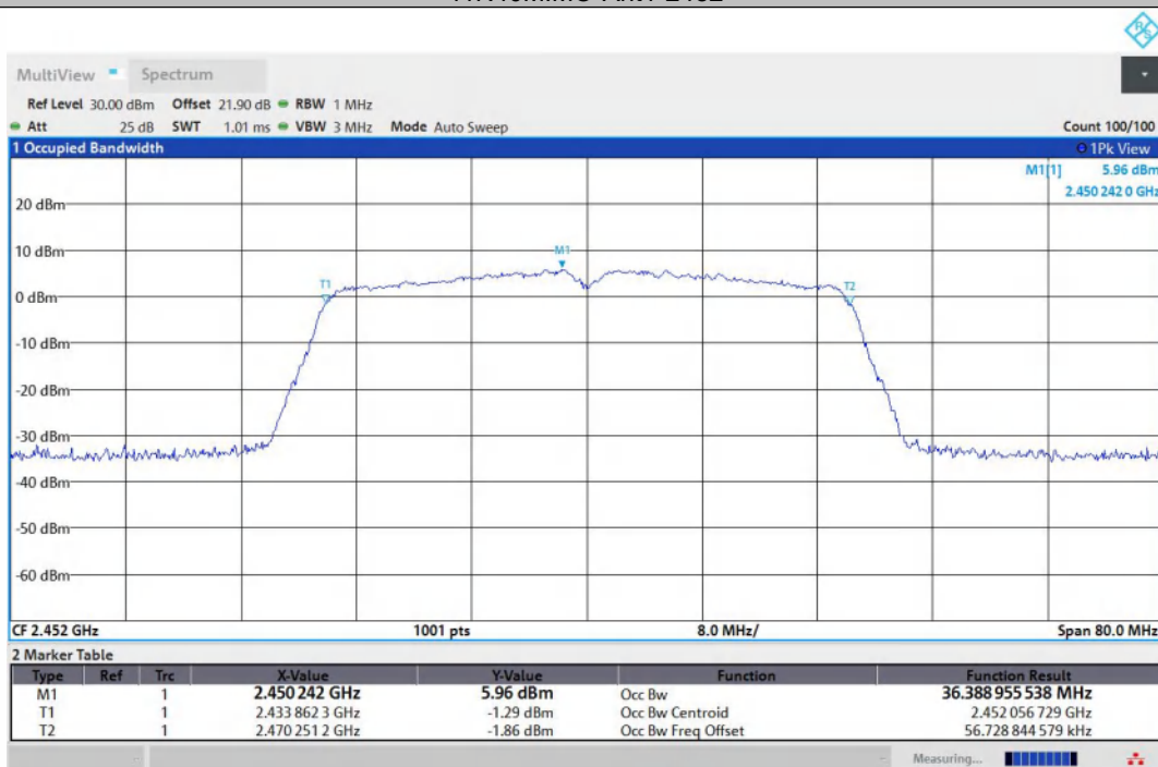
11N40MIMO-Ant2-2452
