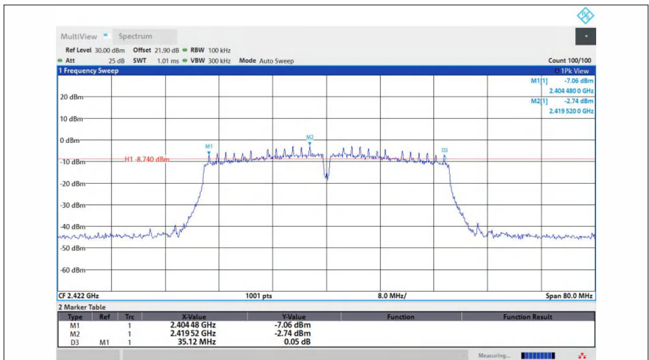
11N40MIMO-Ant1-2422-PASS
