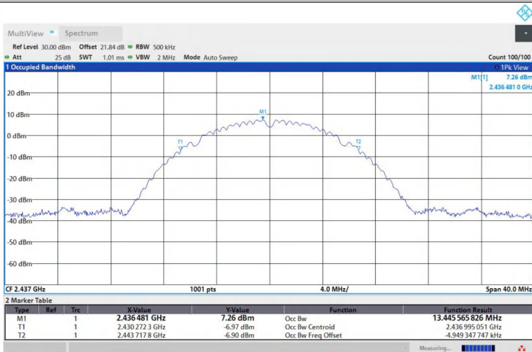
11B-Ant2-2437
